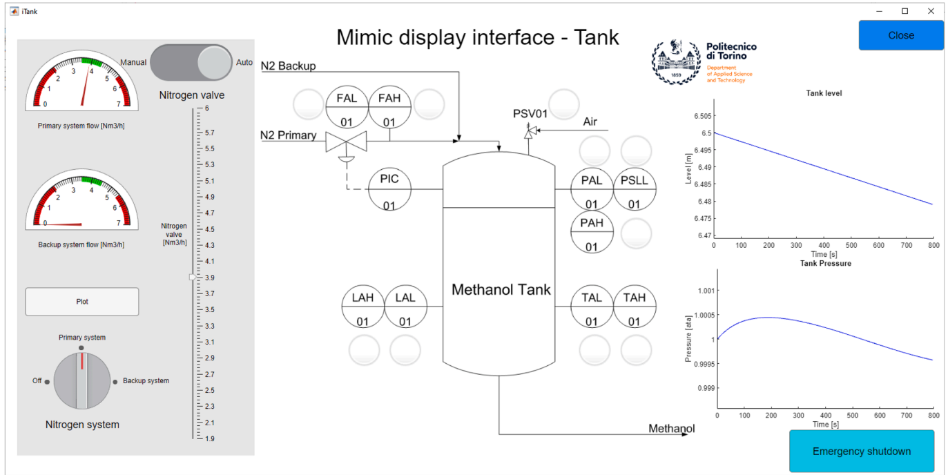
Fig. 2. Tank mimic of the simulator [26].
