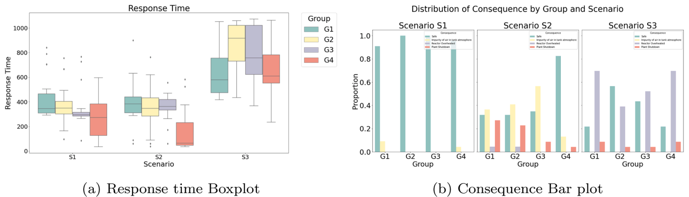
Fig. 9. Response time and consequence distribution.
