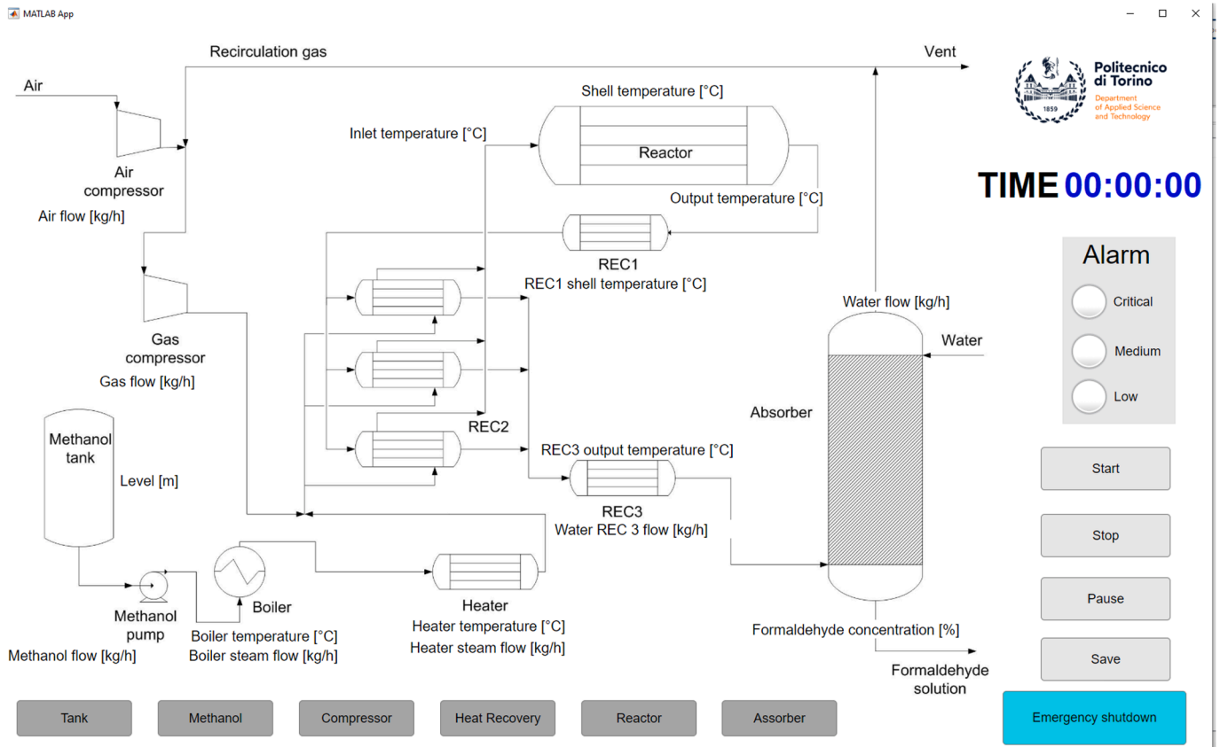
Fig. 1. Main screen of the simulator [26].
