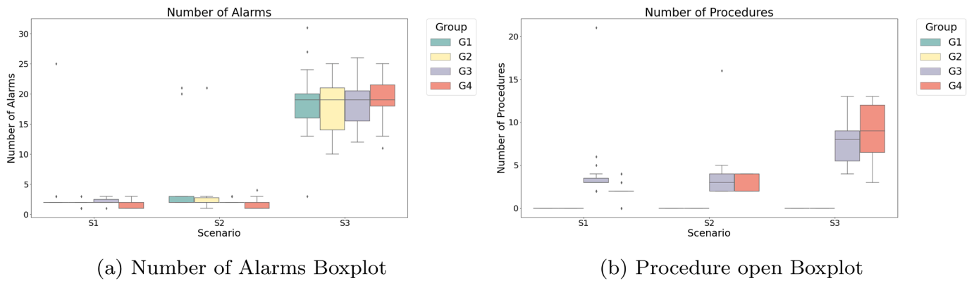
Fig. 7. Number of alarms and procedures distribution.
