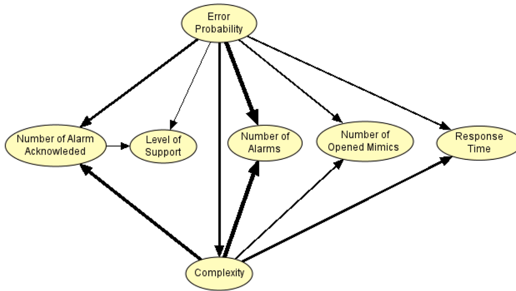
Fig. 11. TAN model structure for predicting operator error probability. "Error Probability" (top centre, class variable) connects to all predictor variables. Predictor variables form a maximum-weight spanning tree rooted at "Complexity" (Scenario), with edges pointing away from the root. This structure indicates that scenario complexity primarily drives most behavioural metrics, while support configuration type behaviour is more strongly associated with alarm acknowledgement. Edge thickness indicates mutual information strength.
