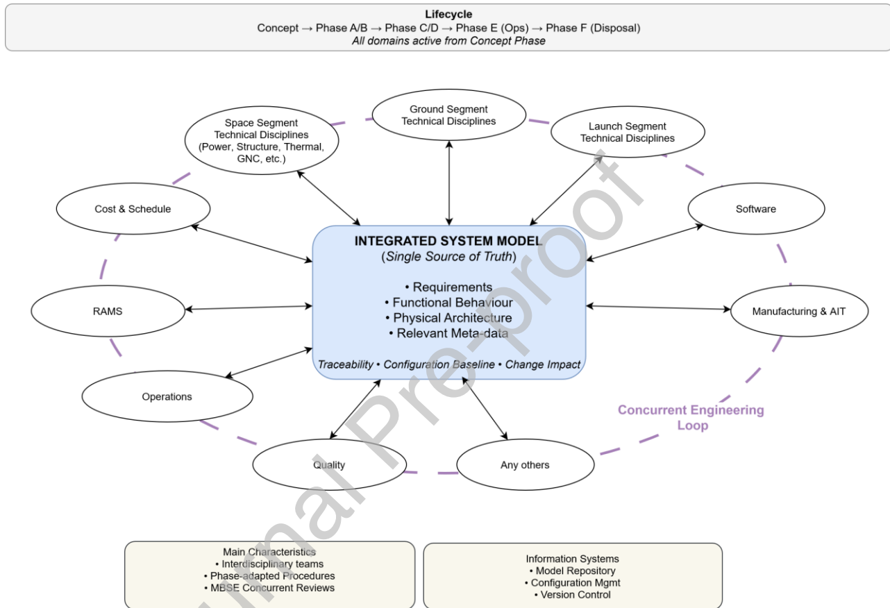
Figure 2 CE-MBSE methodology high level overview
