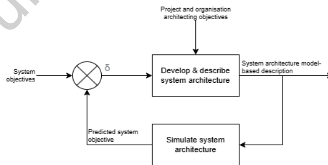
Figure 4 Simulation in architecture design process [29]
