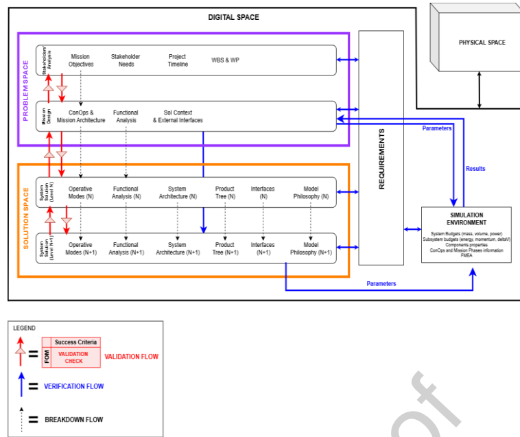
Figure 3 Model-Based approach integration with a focus on V&V
