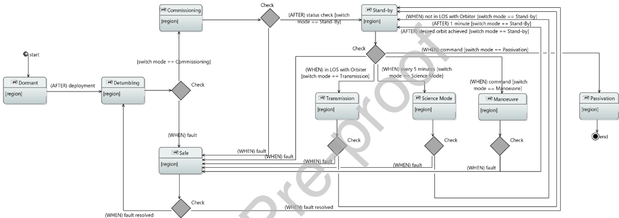
Figure 14 Operative Modes in Capella
