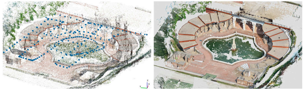
Figure 2. Sparse point cloud reconstructions of the Fontana d'Ercole generated from the same DJI Mini 5 Pro image dataset: Agisoft Metashape Professional ( left ) and RealityScan ( right ). Metashape produced 312k points in 20 min; RealityScan produced 1.9M points in 3 min.
