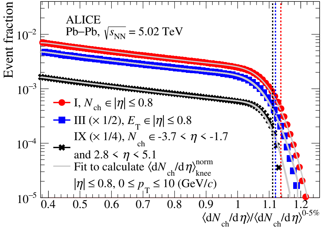
Figure 3. Event fraction distribution as a function of the normalized charged-particle density in Pb-Pb collisions at \sqrt{s_{\text{NN}}} = 5.02 TeV. Centrality classification is based on N_{\text{ch}} (red circles) and E_{\text{T}} (blue squares) in |\eta| \leq 0.8 , and on forward N_{\text{ch}} for the V0 (black crosses). \langle dN_{\text{ch}}/d\eta \rangle^{\text{norm}}_{\text{knee}} is derived from the extrapolated spectra in |\eta| \leq 0.8 . Gray curves represent fits using the model from ref. [54]. The positions of \langle dN_{\text{ch}}/d\eta \rangle^{\text{norm}}_{\text{knee}} , indicated by dashed vertical lines, are 1.137, 1.120, and 1.111 for the N_{\text{ch}} -, E_{\text{T}} -, and V0-based centrality estimators, respectively.
