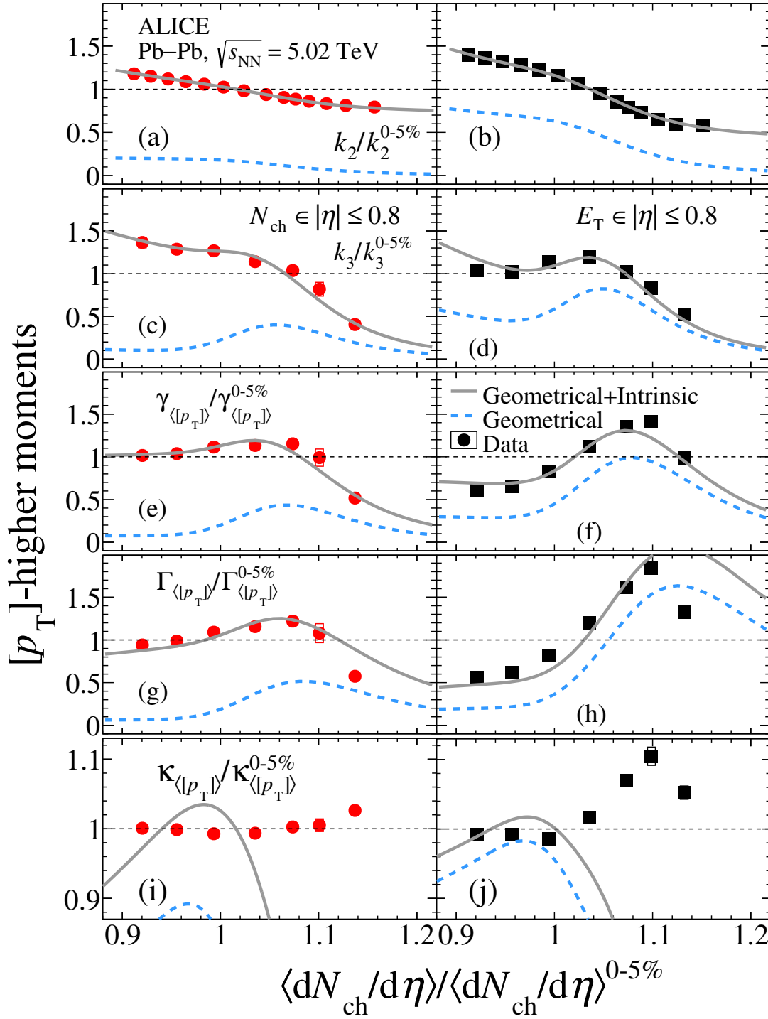
Figure 7. Higher-order moments of [p_T] measured for events selected with the N_{ch} (I) and E_T (III) centrality estimators at mid-rapidity in Pb-Pb collisions at \sqrt{s_{NN}} = 5.02 TeV are shown in the left and right columns, respectively. The k_2^{\text{norm}} distributions are fitted with a two-component model (continuous gray line), where the estimated Geometrical component is also shown (dotted-dashed blue line) [27]. The curves for the k_3^{\text{norm}} , \gamma_{\langle [p_T] \rangle}^{\text{norm}} , \Gamma_{\langle [p_T] \rangle}^{\text{norm}} , and \kappa_{\langle [p_T] \rangle}^{\text{norm}} distributions correspond to predictions based on the fit of k_2^{\text{norm}} [26].
