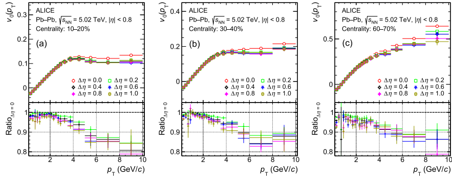
FIG. 5. v_0(p_T) of inclusive charged particles shown as a function of p_T for centrality intervals 10%–20% (a), 30%–40% (b), and 60%–70% (c) for varying pseudorapidity gap ( \Delta\eta ) in Pb-Pb collisions at \sqrt{s_{NN}} = 5.02 TeV. The error bars represent statistical uncertainties. The bottom panel presents the ratio relative to the results for \Delta\eta = 0 .
