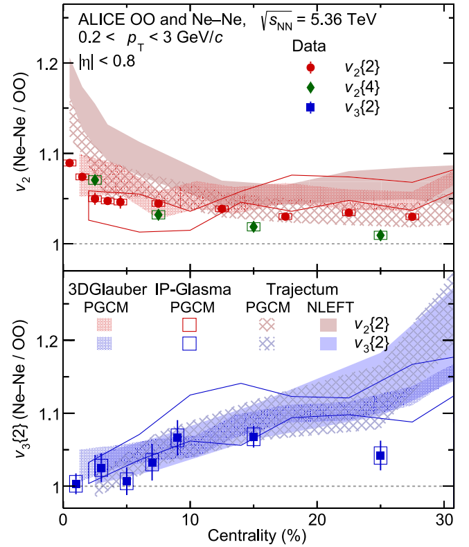
FIG. 3. Ratios v_2(\text{Ne–Ne}/\text{OO}) and v_3(\text{Ne–Ne}/\text{OO}) as a function of centrality in the 0%–30% centrality range. The vertical lines represent statistical uncertainties, and the open boxes represent the systematic uncertainties, while most of them are smaller than the symbol size. The measurements are compared with Trajectum calculations with NLEFT and PGCM inputs [55] as well as IP-Glasma + JIMWLK + MUSIC + UrQMD [93] and 3DGlauber + MUSIC + UrQMD [94] calculations with PGCM input.
