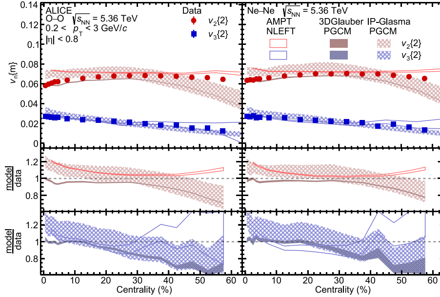
FIG. 6. Charged particle v_2\{2\} and v_3\{2\} as a function of centrality in OO (left) and Ne-Ne (right) collisions. The data points are the same as those in Fig. 2. The measurements are compared with IP-Glasma + JIMWLK + MUSIC + UrQMD [93] and 3DGlauber + MUSIC + UrQMD [94] calculations with PGCM input, as well as AMPT [58] with NLEFT input.
