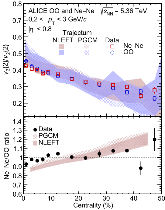
FIG. 4. Top: ratio of the charged particle v_3\{2\} to v_2\{2\} as a function of centrality in OO and Ne–Ne collisions at \sqrt{s_{NN}} = 5.36 TeV. Bottom: double ratios v_3\{2\}/v_2\{2\} (Ne–Ne:OO). The vertical lines represent statistical uncertainties, and the open boxes represent the systematic uncertainties while most of them are smaller than the symbol size. The measurements are compared with Trajectory calculations with NLEFT and PGCM inputs [55].
