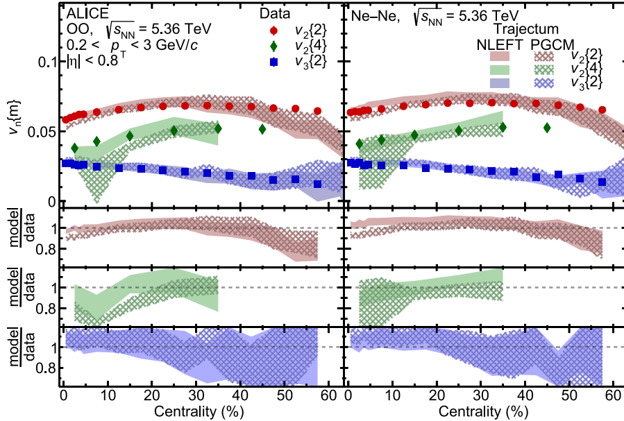
FIG. 2. Charged particle v_2\{2\} , v_3\{2\} , and v_2\{4\} as a function of centrality in OO (left) and Ne-Ne (right) collisions at \sqrt{s_{NN}} = 5.36 TeV. The vertical lines represent statistical uncertainties, and the open boxes represent systematic uncertainties, with most of them being smaller than the symbol size. The measurements are compared with Trajectum calculations with NLEFT and PGCM inputs [55].
