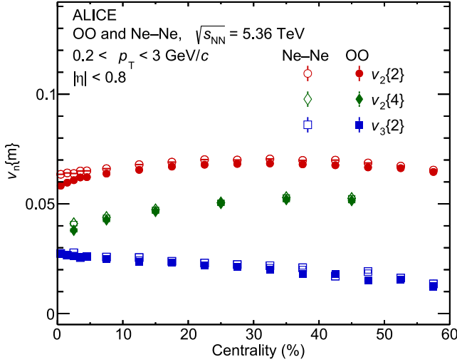
FIG. 1. Charged particle v_2\{2\} , v_3\{2\} , and v_2\{4\} as a function of centrality in OO (solid markers) and Ne-Ne (open markers) collisions at \sqrt{s_{NN}} = 5.36 TeV. The vertical lines represent statistical uncertainties, and the open boxes represent systematic uncertainties, with most of them being smaller than the symbol size.
