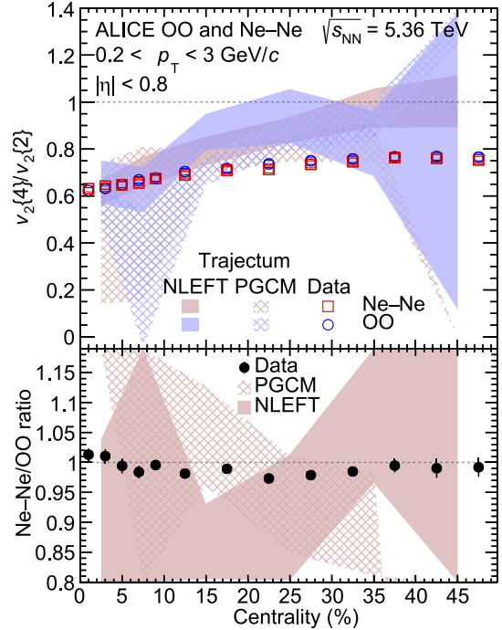
FIG. 5. Top: ratio of the charged particle v_2\{4\} to v_2\{2\} as a function of centrality in OO and Ne–Ne collisions at \sqrt{s_{NN}} = 5.36 TeV. Bottom: double ratios v_2\{4\}/v_2\{2\} (Ne–Ne:OO). The vertical lines represent statistical uncertainties, and the open boxes represent the systematic uncertainties while most of them are smaller than symbol size. The measurements are compared to Trajectory calculations with NLEFT and PGCM inputs [55].
