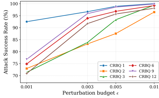
(a) ASR of the input attack for the CRBQ configurations as a function of the perturbation budget \epsilon , expressed as a percentage. Each curve corresponds to one configuration.
