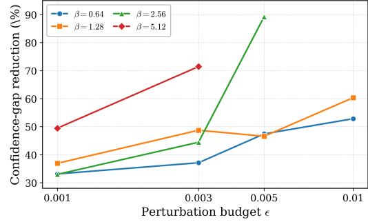
(b) Relative S_{\Delta} reduction for the Entropic Student configurations, measured on the images whose prediction is unchanged, as a function of \epsilon .
