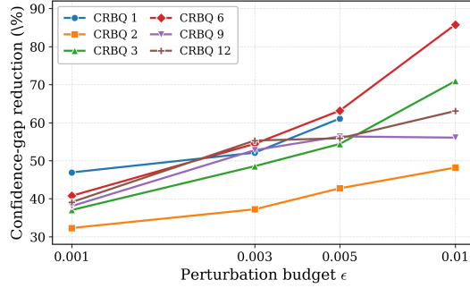
(a) Relative S_{\Delta} reduction for the CRBQ configurations, measured on the images whose prediction is unchanged, as a function of \epsilon .
