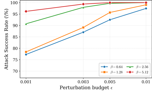
(b) ASR of the input attack for the Entropic Student configurations as a function of \epsilon , expressed as a percentage. Each curve corresponds to one value of \beta .
