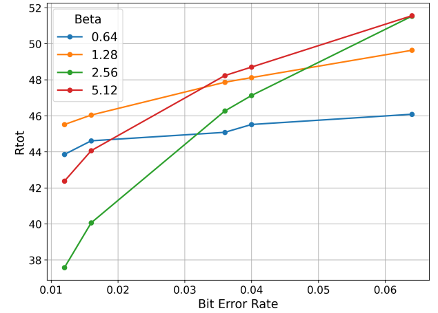
(b) R_{tot} , Entropic Student.
