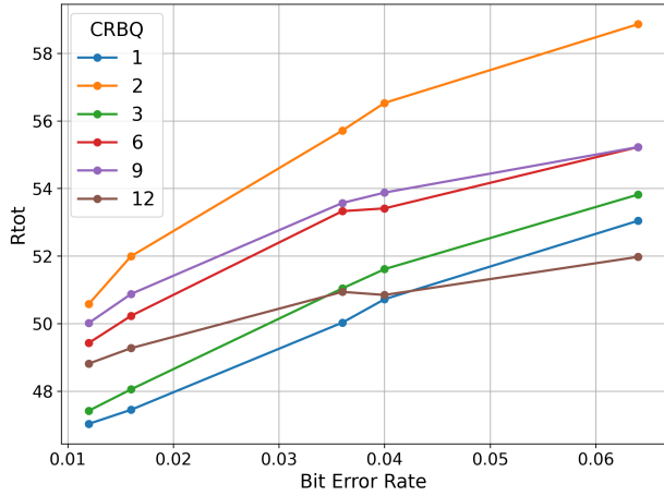
(a) R_{tot} , CRBQ.
