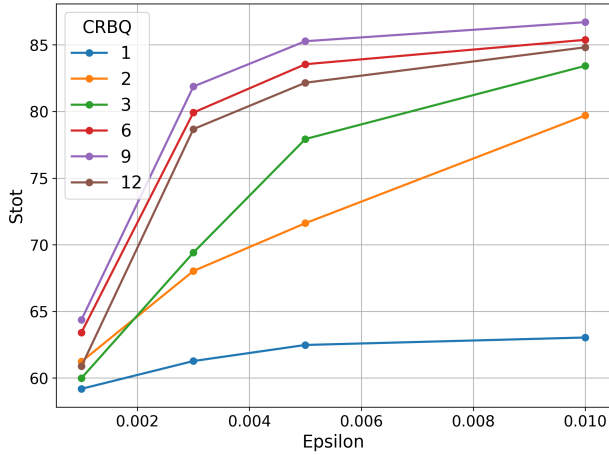
(c) S_{tot} , CRBQ.
