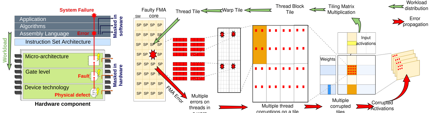
Fig. 2: A general scheme from [11] of physical defects propagation across system components (Left), and an illustration of fault propagation effects on matrix multiplication operations through different levels of the tiling (Right).
