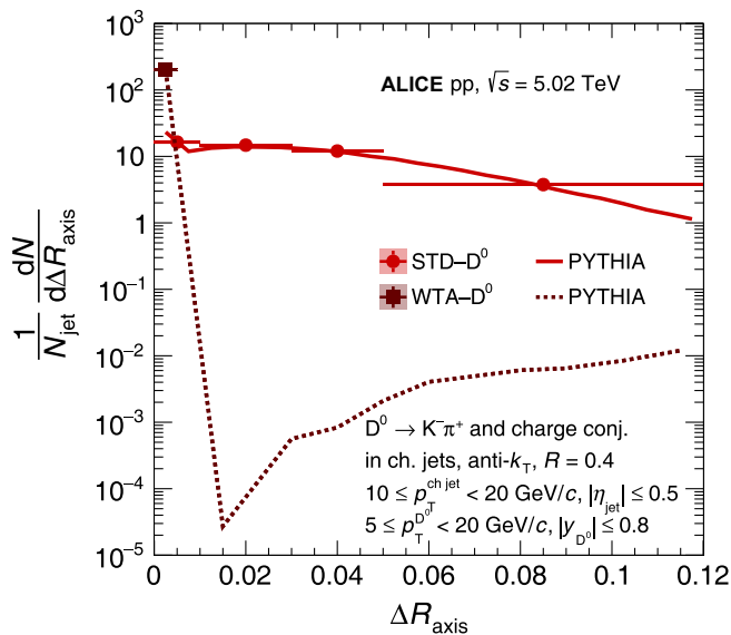
FIG. 4. Unfolded jet axes difference distribution for \Delta R_{\text{WTA-}D^0} and \Delta R_{\text{STD-}D^0} in 10 \leq p_T^{\text{ch jet}} < 20 GeV/ c . Includes systematic and statistical uncertainties represented by color boxes and error bars, respectively, and a comparison to predictions from PYTHIA8.
