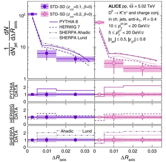
FIG. 9. Fully unfolded jet axes difference distributions for \Delta R_{STD-SD} with z_{cut} = 0.1 (left) and z_{cut} = 0.2 (right), \beta = 0 and 10 \leq p_T^{ch jet} < 20 GeV/c. Systematic and statistical uncertainties are represented by color boxes and error bars, respectively, and MC event generator comparisons are shown in the bottom panels.
