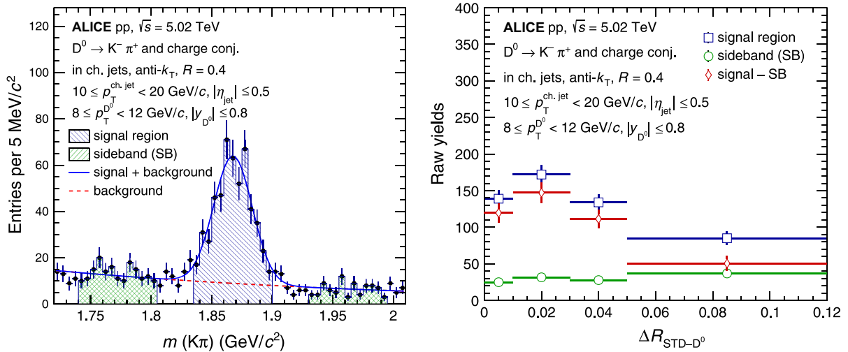
FIG. 2. Left: the D^0 -decay candidate invariant-mass distribution for 10 \leq p_T^{\text{ch jet}} < 20 GeV/ c and 8 < p_T^{D^0} < 12 GeV/ c . The total fit function of the signal and background is represented by the blue line. The background fit function is represented by the red line. Right: the raw yields of the D^0 -tagged jets as a function of \Delta R_{\text{STD-}D^0} in the signal region and sideband region.
