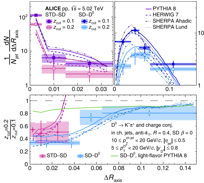
FIG. 12. Fully unfolded jet axes difference distributions for \Delta R_{\text{STD-SD}} (left) and \Delta R_{\text{SD-}D^0} (right), in 10 \leq p_T^{\text{ch jet}} < 20 \text{ GeV}/c . The soft drop parameter, z_{\text{cut}} , is varied between z_{\text{cut}} = 0.1 and z_{\text{cut}} = 0.2 ; the parameter \beta = 0 throughout. Systematic and statistical uncertainties are represented by color boxes and error bars, respectively. Comparisons to MC event generators are included. The bottom panel shows a ratio of the z_{\text{cut}} = 0.2 distribution over the z_{\text{cut}} = 0.1 distribution for \Delta R_{\text{SD-}D^0} and \Delta R_{\text{STD-SD}} . These ratios are taken for both the D^0 -tagged data and each MC event generator.
