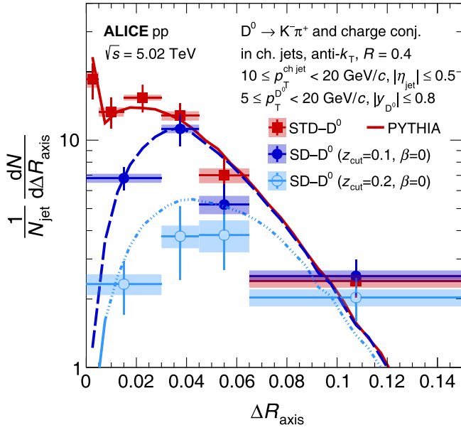
FIG. 6. Fully unfolded jet axes difference distributions for \Delta R_{STD-D^0} and \Delta R_{SD-D^0} , where the soft drop parameters are \beta = 0 and z_{\text{cut}} = 0.1 or 0.2 , in 10 \leq p_T^{\text{ch jet}} < 20 GeV/c. Systematic and statistical uncertainties are represented by color boxes and error bars, respectively. Comparisons to predictions from PYTHIA8 are included.
