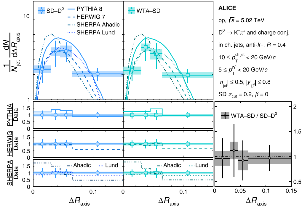
FIG. 8. Fully unfolded jet axes difference distributions for \Delta R_{SD-D^0} (left) and \Delta R_{WTA-SD} (middle), with grooming parameters z_{cut} = 0.2 and \beta = 0 , for 10 \leq p_T^{ch jet} < 20 GeV/c. Systematic and statistical uncertainties are represented by color boxes and error bars, respectively, and MC event generator comparisons are shown in the bottom panels. The bottom right panel shows a ratio of the two data distributions.
