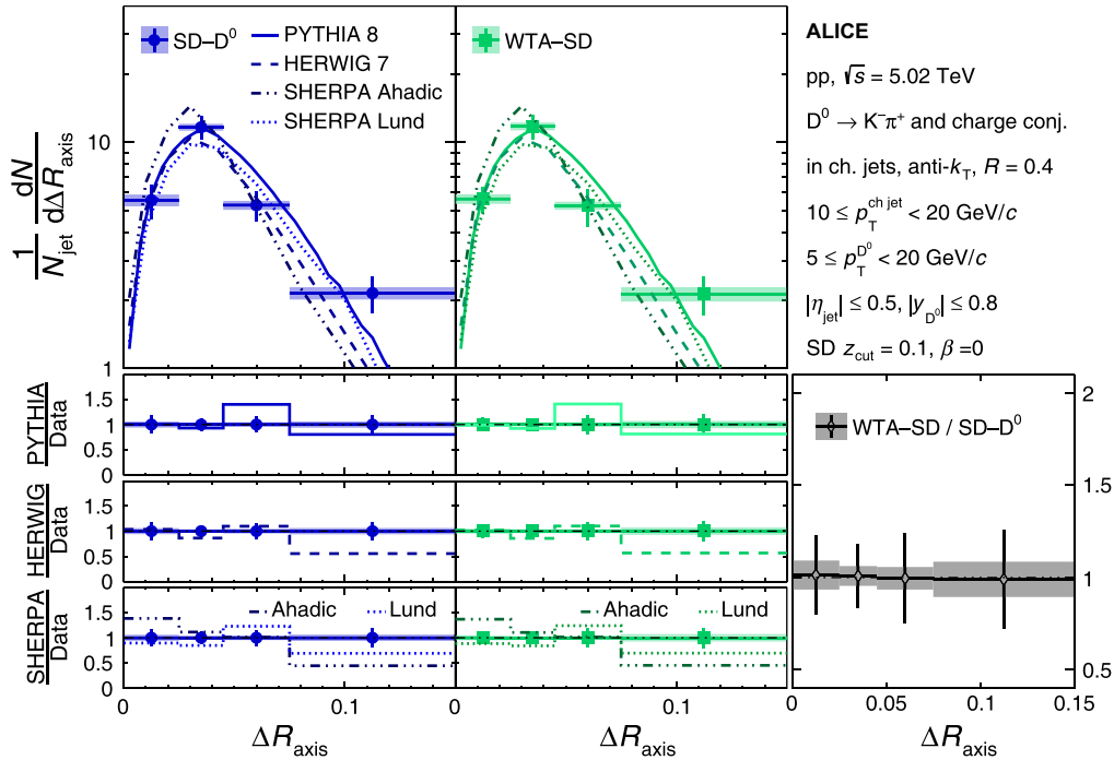
FIG. 7. Fully unfolded jet axes difference distributions for \Delta R_{SD-D^0} (left) and \Delta R_{WTA-SD} (middle), with grooming parameters z_{\text{cut}} = 0.1 and \beta = 0 , for 10 \leq p_T^{\text{ch jet}} < 20 GeV/c. Systematic and statistical uncertainties are represented by color boxes and error bars, respectively, and MC event generator comparisons are shown in the bottom panels. The bottom right panel shows a ratio of the two data distributions.
