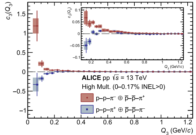
Fig. 9 Extracted cumulants of p\text{-}p\text{-}\pi^+ (blue) and p\text{-}p\text{-}\pi^- (red) as a function of Q_3 after subtracting the lower-order contributions from the triplet correlations. The lines (boxes) represent the statistical (systematic) uncertainties
