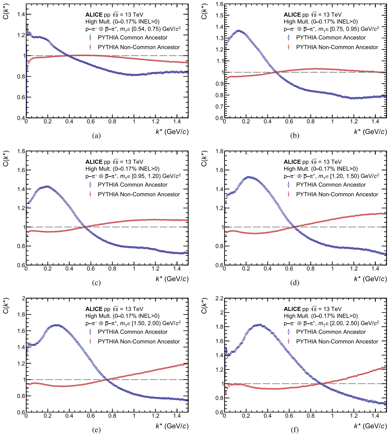
Fig. 13 The correlation function of p-\pi^- pairs for common and non-common ancestor obtained with PYTHIA 8.2 (Monash 2013 Tune) [65,66] together with GEANT3 [67] as a function of the pair relative momentum k^* in several intervals of the pair m_T : a [0.54, 0.75] GeV/c 2 , b [0.75, 0.95] GeV/c 2 , c [0.95, 1.2] GeV/c 2 , d
