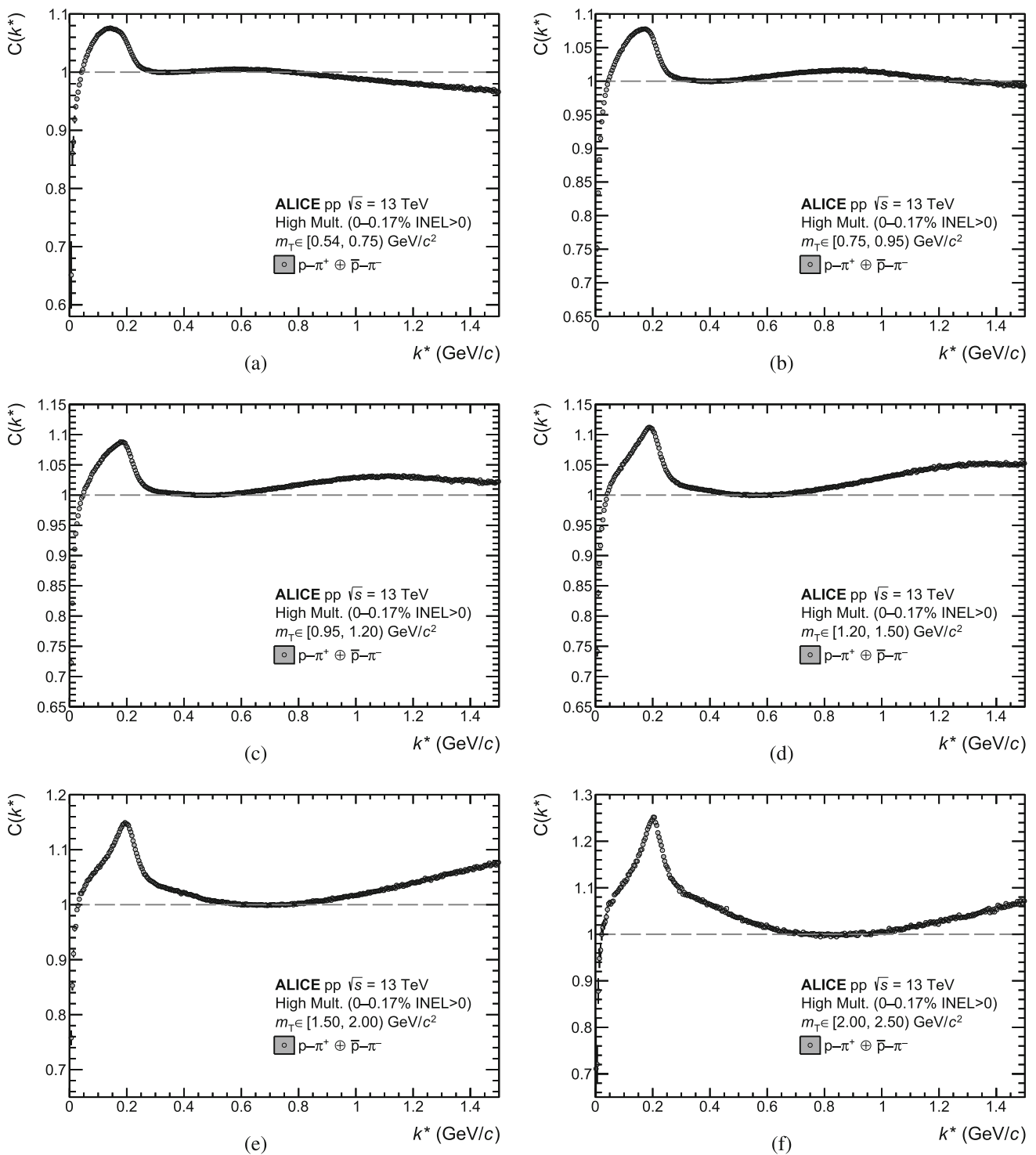
Fig. 10 The experimental correlation function of p-\pi^+ pairs as a function of the pair relative momentum k^* in several intervals of the pair m_T : a [0.54, 0.75] GeV/c 2 , b [0.75, 0.95] GeV/c 2 , c [0.95, 1.2] GeV/c 2 , d
