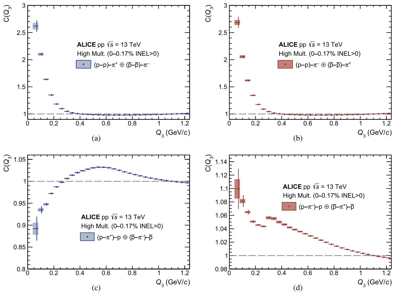
Fig. 7 Lower-order contributions present in the p\text{-}p\text{-}\pi^\pm systems. The contributions of a (p\text{-}p)\text{-}\pi^+ and b (p\text{-}p)\text{-}\pi^- , as well as c (p\text{-}\pi^+)\text{-}p and d (p\text{-}\pi^-)\text{-}p are shown. The statistical (systematic) uncertainties are represented by the lines (boxes). The horizontal lines show the over-
