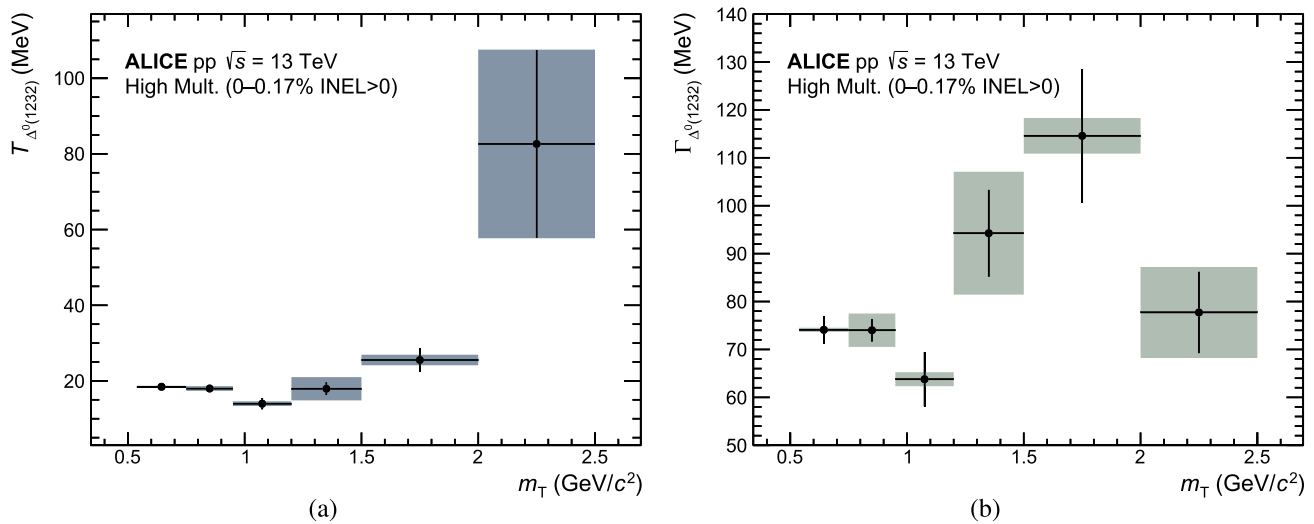
Fig. 5 Extracted a \Delta^0 spectral temperature and b width as a function of the pair transverse mass m_T for the \Delta^0(1232) . The lines show the statistical uncertainties, while the boxes represent the systematic uncertainties
