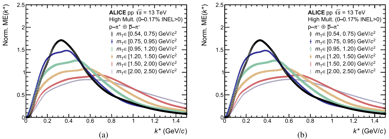
Fig. 15 The normalized mixed event distributions of a p\text{--}\pi^+ and b p\text{--}\pi^- pairs for all relevant m_T intervals
