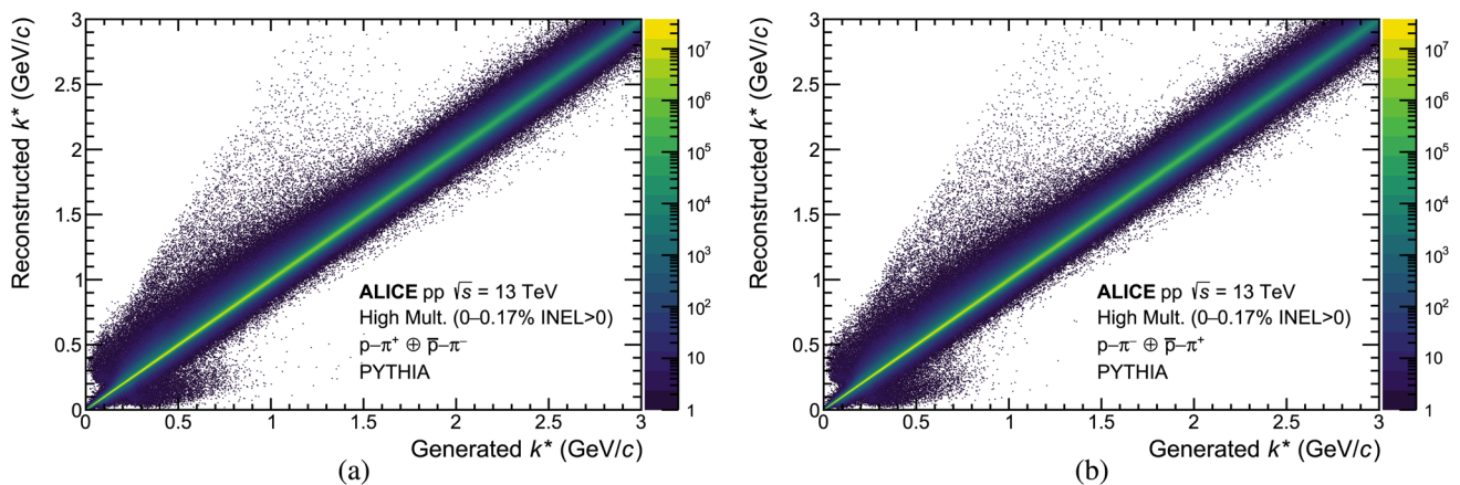
Fig. 14 Momentum smearing matrix of a p\text{--}\pi^+ pairs and b p\text{--}\pi^- pairs obtained with PYTHIA 8.2 (Monash 2013 Tune) [65,66] together with GEANT3 [67]
