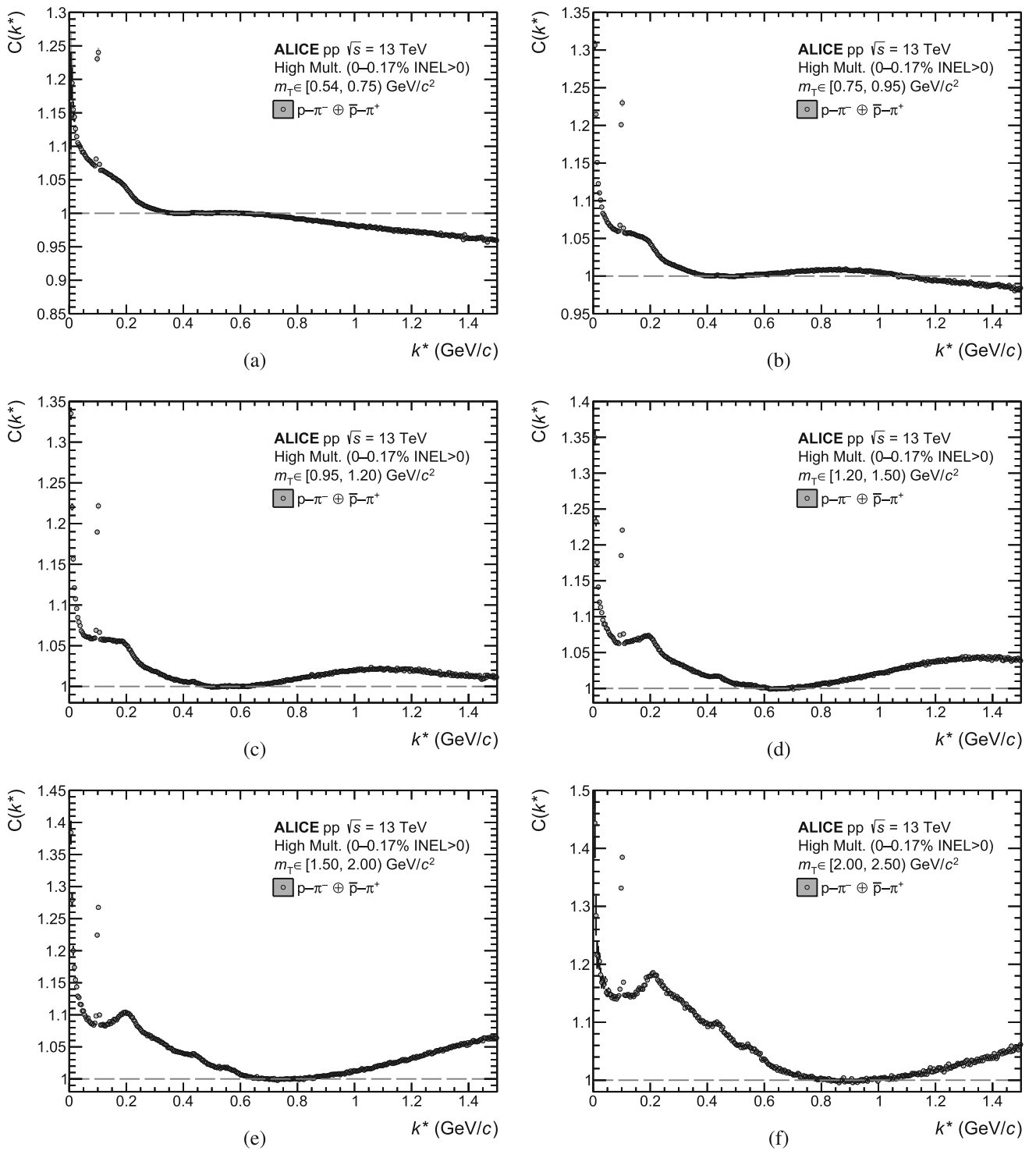
Fig. 11 The experimental correlation function of p-\pi^- pairs as a function of the pair relative momentum k^* in several intervals of the pair m_T : a [0.54, 0.75] GeV/c 2 , b [0.75, 0.95] GeV/c 2 , c [0.95, 1.2] GeV/c 2 ,
