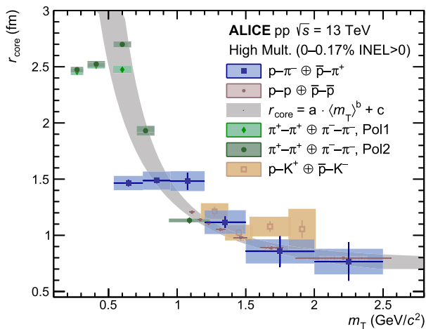
Fig. 6 Extracted core source size r_{\text{core}} for primordial p-\pi^- pairs for several m_T ranges. The obtained result is compared with the results from p-p pairs [24], \pi^\pm-\pi^\pm and p-K^+ pairs [22]. The statistical (systematic) uncertainties are shown as lines (boxes). The extrapolated scaling of p-p pairs [24] is shown as the gray band
