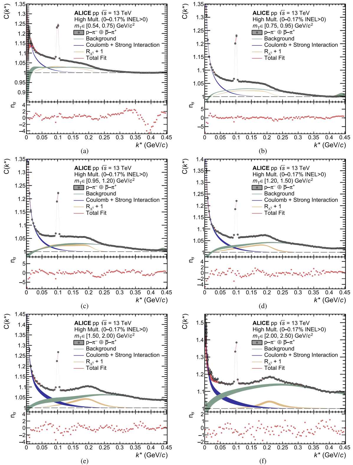
Fig. 4 Upper panel: The p\pi^- experimental correlation function is shown in black as a function of the pair relative momentum k^* for several intervals of the pair m_T : a [0.54, 0.75] GeV/c 2 , b [0.75, 0.95] GeV/c 2 , c [0.95, 1.20] GeV/c 2 , d [1.20, 1.50] GeV/c 2 , e [1.50, 2.00] GeV/c 2 , and f [2.00, 2.50] GeV/c 2 . The lines and boxes show the statistical and systematic uncertainties of the experimental data, respectively. The fit
