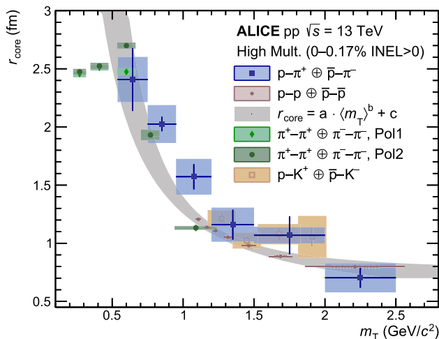
Fig. 3 Extracted source size r_{\text{core}} of primordial p\text{--}\pi^+ pairs as a function of the pair transverse mass. The results are compared with the r_{\text{core}} extracted from p\text{--}p pairs [24] as well as \pi^{\pm}\text{--}\pi^{\pm} and p\text{--}K^+ pairs [22] in HM pp collisions at \sqrt{s} = 13 TeV by ALICE. The lines (boxes) show the statistical (systematic) uncertainties. The gray band represents the extrapolated scaling of p\text{--}p pairs [24]
