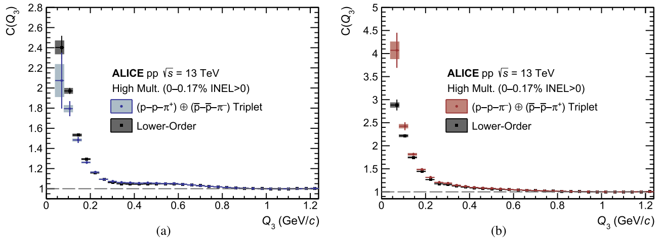
Fig. 8 Comparison of the three-particle correlation functions of a p\text{-}p\text{-}\pi^+ and b p\text{-}p\text{-}\pi^- to their respective total lower-order contributions (grey). The statistical and systematic uncertainties are shown by the lines and boxes, respectively. The lower-order contribution is given
