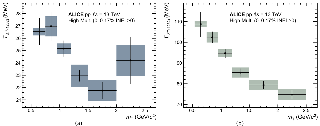
Fig. 2 Results for the a \Delta^{++} spectral temperature and b width as a function of the pair transverse mass m_T for the \Delta^{++}(1232) with the statistical (lines) and systematic (boxes) uncertainties
