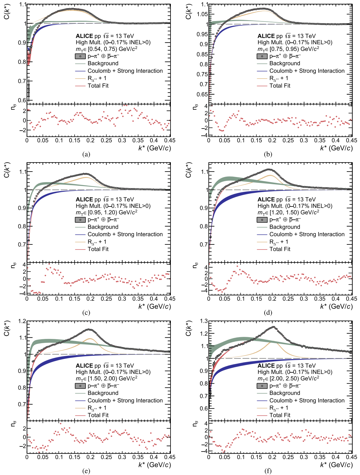
Fig. 1 Upper panel: The experimental correlation function of p-\pi^+ pairs (black) as a function of the pair relative momentum k^* in several intervals of the pair m_T : a [0.54, 0.75] \text{ GeV}/c^2 , b [0.75, 0.95] \text{ GeV}/c^2 , c [0.95, 1.20] \text{ GeV}/c^2 , d [1.20, 1.50] \text{ GeV}/c^2 , e [1.50, 2.00] \text{ GeV}/c^2 , and f [2.00, 2.50] \text{ GeV}/c^2 . The lines (boxes) show the statistical (systematic) uncertainties of the experimental data. The red bands show the fit result
