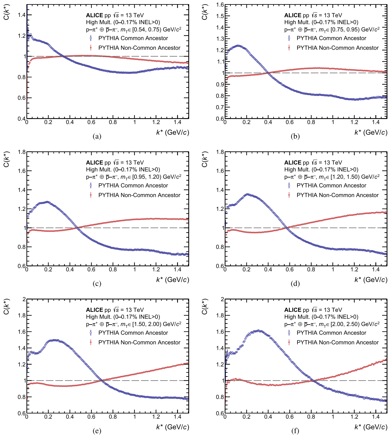
Fig. 12 The correlation function of p-\pi^+ pairs for common and non-common ancestor obtained with PYTHIA 8.2 (Monash 2013 Tune) [65,66] together with GEANT3 [67] as a function of the pair relative momentum k^* in several intervals of the pair m_T : a [0.54, 0.75] \text{GeV}/c^2 , b [0.75, 0.95] \text{GeV}/c^2 , c [0.95, 1.20] \text{GeV}/c^2 , d
