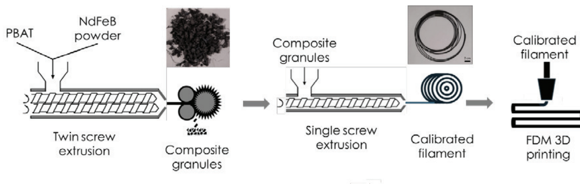
Figure 2 Experimental set-up to produce composite granules and calibrated filaments
