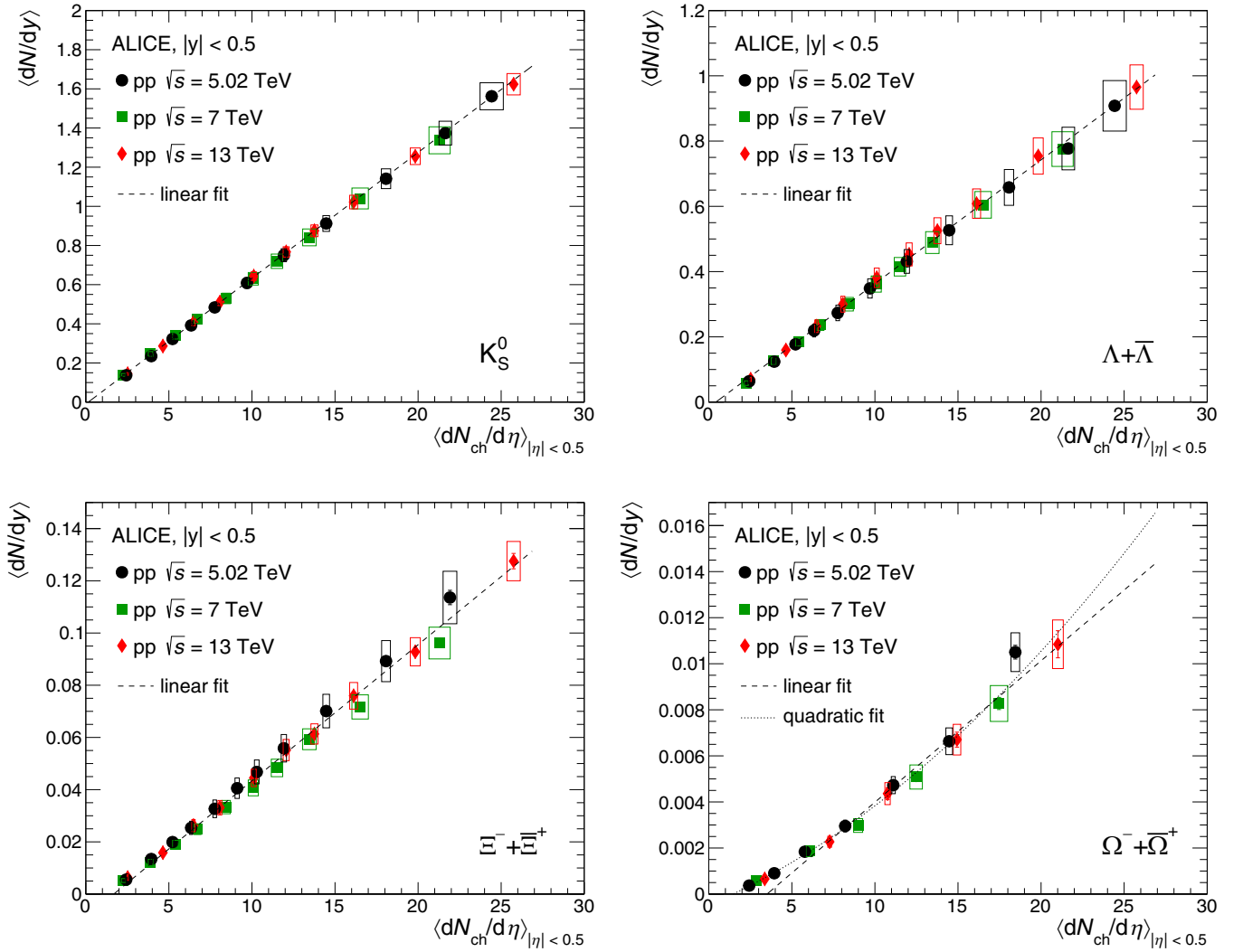
FIG. 4. p_T -integrated yields in pp collisions at different center-of-mass energies and midrapidity as a function of the event multiplicity for K_S^0 and \Lambda (top panels), \Xi and \Omega (bottom panels). \sqrt{s} = 5.02 TeV results are shown as black dots, \sqrt{s} = 7 TeV results [13] as green squares and \sqrt{s} = 13 TeV results [14] as red diamonds. Statistical uncertainties are represented as error bars and systematic uncertainties as boxes whose width represents the systematic error on the multiplicity determination. Linear combined fits are shown as dashed lines, while the quadratic fit to the \Omega progression is shown as a dotted line.
