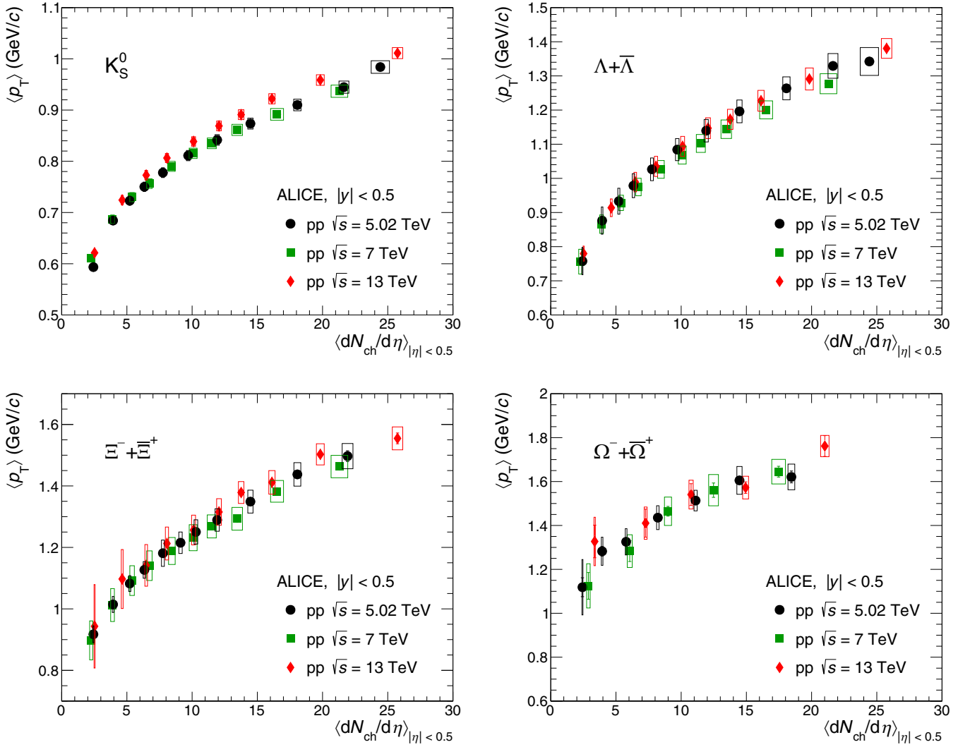
FIG. 2. \langle p_T \rangle in pp collisions at different center-of-mass energies and midrapidity as a function of the event multiplicity for K_S^0 and \Lambda (top panels), \Xi and \Omega (bottom panels). \sqrt{s} = 5.02 TeV results are shown as black dots, \sqrt{s} = 7 TeV results [13] as green squares, and \sqrt{s} = 13 TeV results [14] as red diamonds. Statistical uncertainties are reported as error bars, systematic uncertainties as boxes whose width represents the systematic error on the multiplicity determination.
