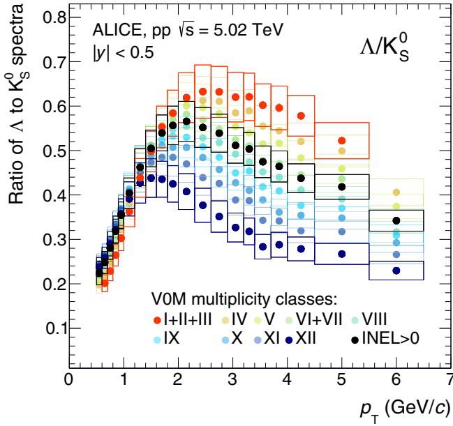
FIG. 3. p_T distribution of \Lambda/K_S^0 ratio in pp collisions at \sqrt{s} = 5.02 TeV and midrapidity for different multiplicity classes are shown with different colors. The lowest, highest, and the \text{INEL} > 0 classes are highlighted.
