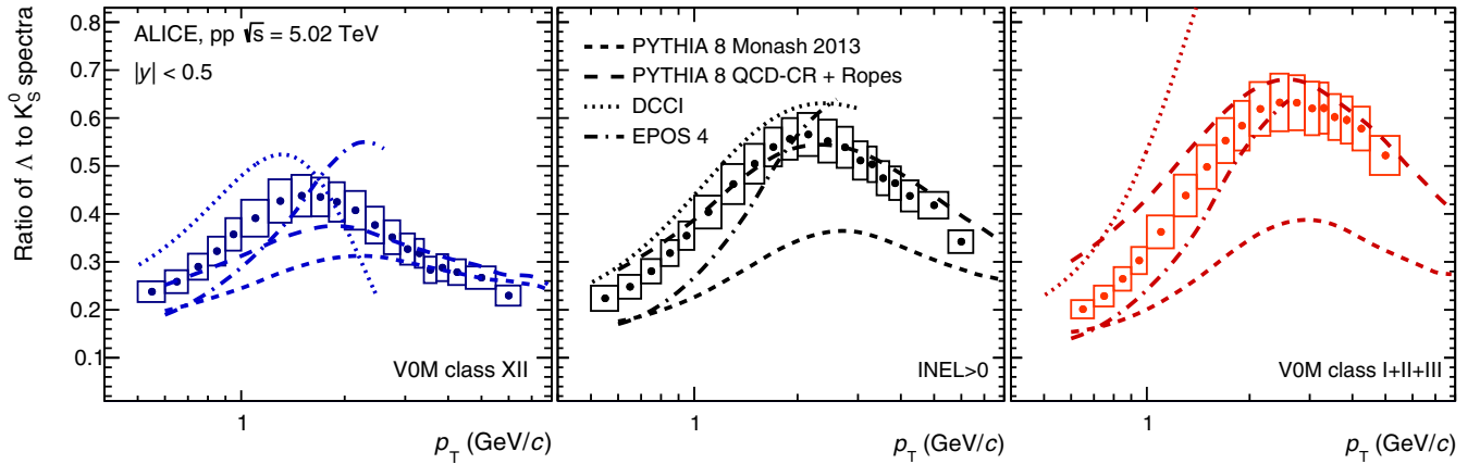
FIG. 6. p_T distribution of \Lambda/K_S^0 ratio in the INEL > 0 event class (center) and low and high-multiplicity classes (left and right panels, respectively) from pp collisions at \sqrt{s} = 5.02 TeV. Data are compared with PYTHIA 8 Monash 2013 (dashed lines), PYTHIA 8 QCD-QR+Ropes (long-dashed lines), DCCI (dotted lines), and EPOS 4 (dash-dotted lines) MC generators.
