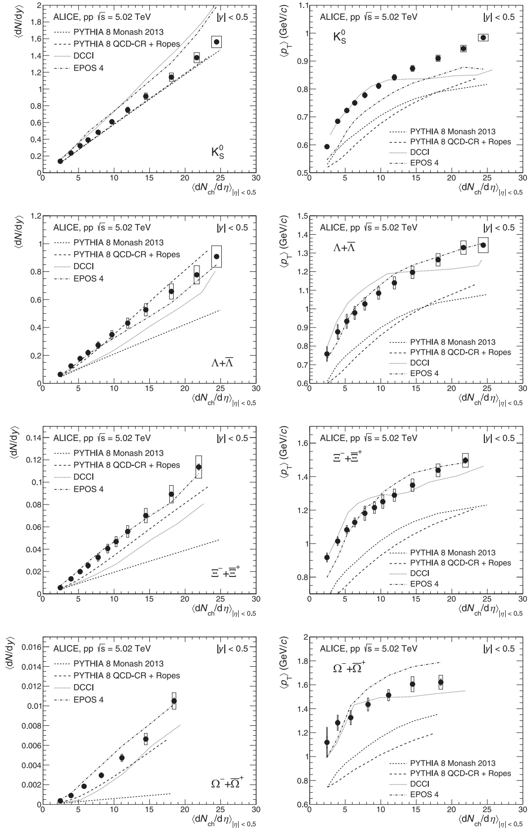
FIG. 5. p_T -integrated yields (left column) and \langle p_T \rangle (right column) at \sqrt{s} = 5.02 TeV for K_S^0 , \Lambda , \Xi , and \Omega compared with MC generators PYTHIA 8 Monash 2013 (Ref. [43], dashed line), PYTHIA 8 QCD-CR+Ropes (Ref. [19], long-dashed line), DCCI (Ref. [24], dotted line) and EPOS 4 (Ref. [46], dash-dotted line).
