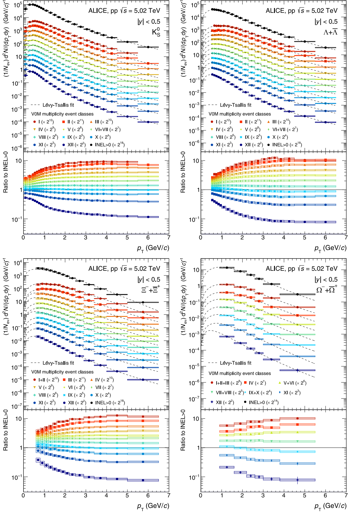
FIG. 1. p_T distributions at midrapidity for K_S^0 , \Lambda , \Xi , and \Omega for multiplicity classes and INEL > 0 , as indicated. Statistical uncertainties are shown as error bars, the systematic ones as boxes. The bottom panels present the ratio of all spectra to the INEL > 0 one. The dashed curves show the Lévy-Tsallis [37] fit to the p_T distributions.
