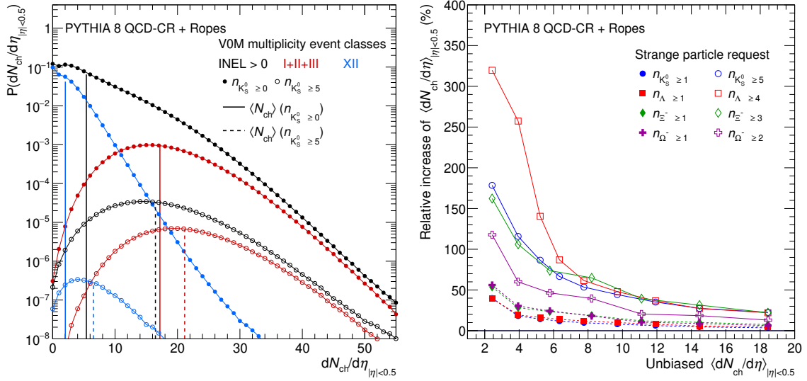
Figure 5. Illustration of the strangeness-induced charged-particle multiplicity bias effect from PYTHIA 8 QCD-CR + Ropes simulation. ( left ) dN_{ch}/d\eta|_{|\eta|<0.5} distribution in the INEL > 0, V0M-(I+II+III) and V0M-XII event classes. Open markers are the corresponding dN_{ch}/d\eta|_{|\eta|<0.5} resulting from the additional request of at least 5 K_S^0 in the event. Continuous and dashed vertical lines show the averages of the unbiased and biased multiplicity distributions, respectively. ( right ) Relative shift in the \langle dN_{ch}/d\eta \rangle for all the different V0M event classes when requiring at least one (full markers) or more than one (open markers) strange particles in the event. Lines are shown to guide the eye.
