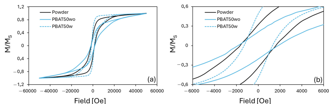
Figure 11. Hysteresis loops for PBAT50w/wo as representative samples (a) compared to that of the pristine powder, normalized to M_s , as reported in Table 4. Details of the curves in the low field range (b).
