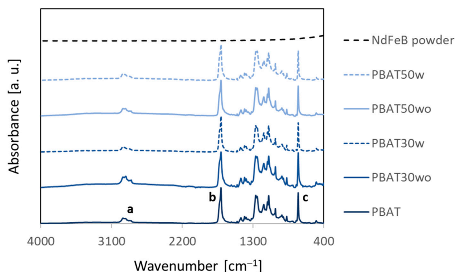
Figure 6. IR spectra of pristine PBAT, different magnetic composites, and NdFeB powder. Labels a, b and c indicate the main absorption bands of the polymer.
