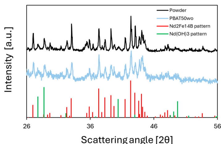
Figure 9. Comparison of the XRD spectrum of the composite (blue line) with that of the recycled powder sieved below 50 mm (black line). NdFeB (red bars) and Nd(OH) 3 (green bars).
