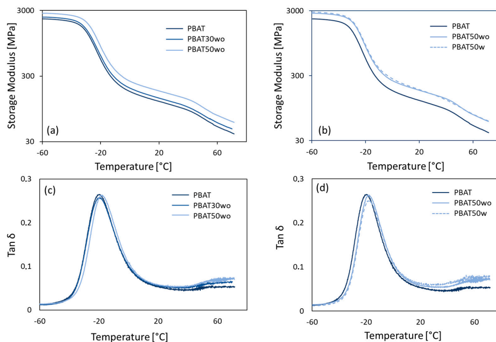
Figure 7. DMA and Tan \delta curves of magnetic composites at different NdFeB powder contents printed without (a,c) and with (b,d) the magnetic support.
