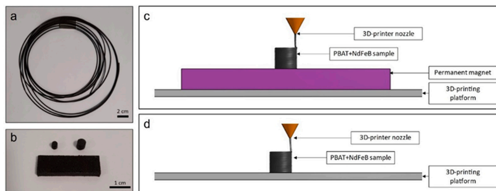
Figure 4. The magnetic filament loaded with 50% NdFeB, as a representative sample (a); some of the 3D-printed samples (b); 3D printer configurations with (c) and without (d) the permanent magnet on the printing platform.
