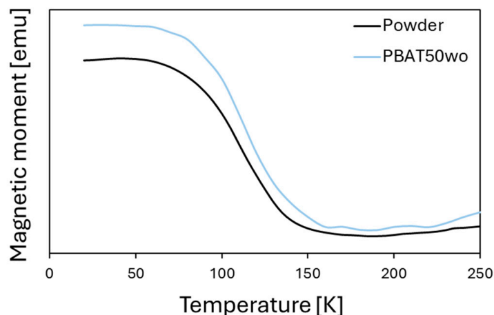
Figure 10. Magnetization of composite PBAT50wo, as representative sample, (blue line) and powder (black line) as a function of the temperature measured with a constant magnetic field of 1 kOe.
