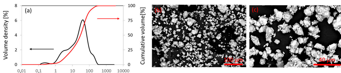
Figure 5. Distributive and cumulative particle size distribution curves (a) and SEM image of NdFeB powder (b,c) at different magnifications.
