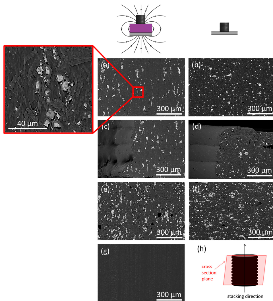
Figure 8. SEM images of PBAT30w (a)—in the inset, NdFeB particles in the PBAT30w sample at higher magnifications, PBAT30wo (b), side view of PBAT30w (c), side view of PBAT30wo (d)—as representative samples, PBAT50w (e), PBAT50wo (f), and not-loaded PBAT (g); graphic representation of analyzed surfaces (h). On the top, the two printing configurations are schematized, with the magnetic field lines generated by the permanent magnet.
