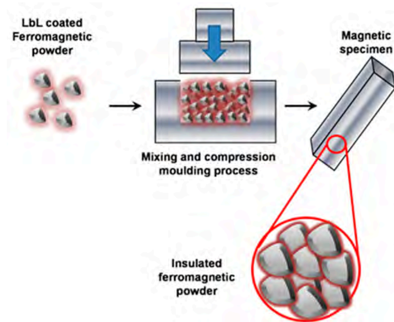
Figure 2. Compaction of the coated iron powder.
