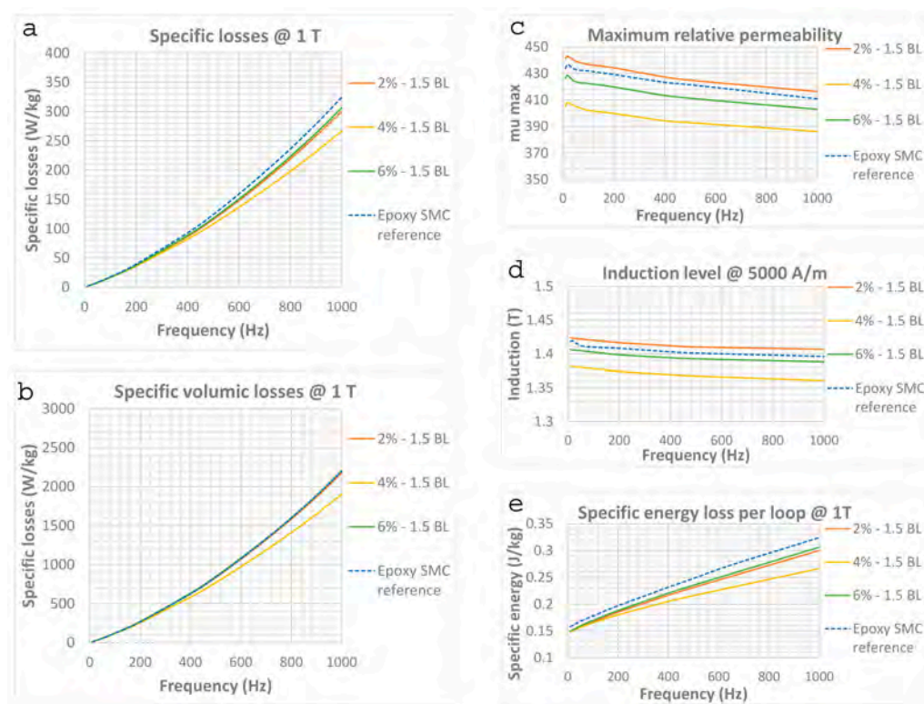
Figure 8. Magnetic and energetic comparison as a function of the variation in the SiO 2 with coating obtained with 1.5 BL (3 layers): Specific iron loss @ 1 T as a function of frequency related to weight (a) and volume (b); maximum relative magnetic permeability as a function of frequency (c); magnetic induction @ 5000 A/m as a function of frequency (d) and specific energy @ 1 T as a function of frequency (e).
