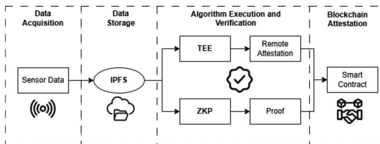
Figure 1. Overview of the proposed certification segment of the damage assessment pipeline.
