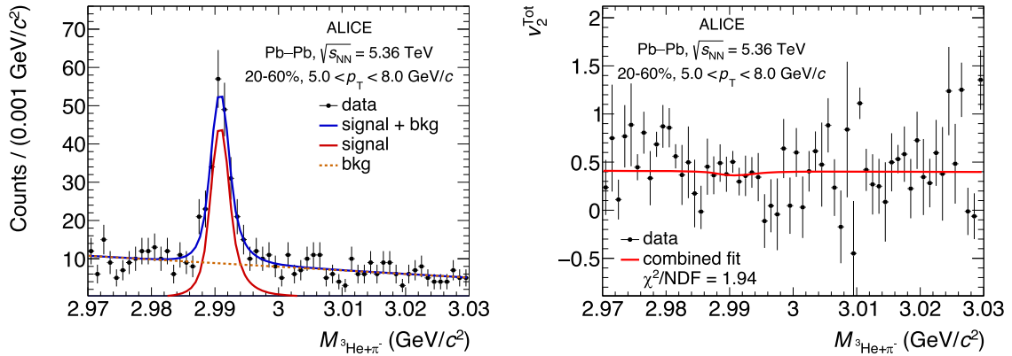
Fig. 1. Invariant-mass distribution of ^3\text{H} candidates (left) and v_2 as a function of the invariant mass (right), in the 5 < p_T < 8 \text{ GeV}/c transverse-momentum interval and the 20–60% centrality interval. In the left panel, the solid red line represents the fit with a DSCB function (signal) while the dotted line displays the fit of the background with a second-order polynomial function. The total fit is shown with the solid blue line. In the right panel, the solid red line represents the fit function described in Eq. (5).
