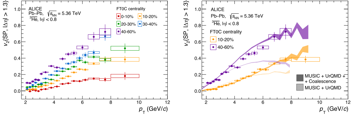
Fig. 2. Measured v_2 of {}^3\text{He} as a function of p_T for the various centrality intervals (left) and comparison with predictions of hydrodynamical models [56] with and without a coalescence afterburner for two selected centrality intervals (right). Error bars represent statistical uncertainties, while boxes indicate systematic uncertainties, respectively. The widths of the model bands represent their statistical uncertainties.
