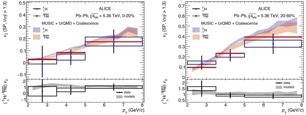
Fig. 3. v_2 of {}^3\text{He} (red markers) and hypertriton (blue markers) as a function of p_T for the 0-20% (left panel) and 20-60% (right panel) centrality intervals. Error bars represent statistical uncertainties, while boxes indicate systematic uncertainties, respectively. The data points are compared with the coalescence model expectations (see the text for details) for the two nuclear species.
