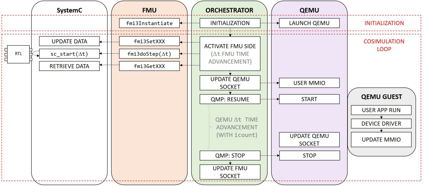
Fig. 3. Overview of the co-simulation framework. The orchestrator instantiates both domains (QEMU and FMU), then executes a time-synchronized loop: FMU receives updated input and runs for \Delta t ; the results are copied to the QEMU MMIO area; QEMU runs for \Delta t executing the user application, eventually updating the MMIO through the device driver.
