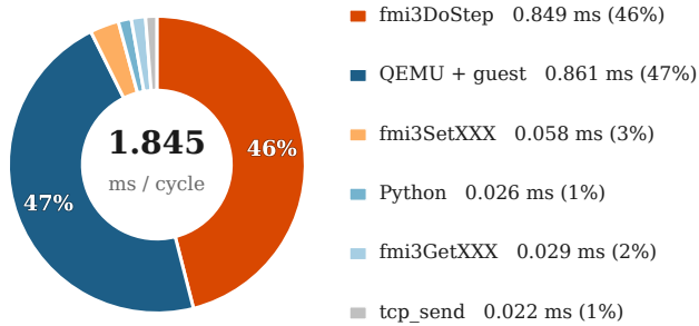
Fig. 4. Single-cycle time breakdown of the I2C vHIL co-simulation on RISC-V, considering mean latencies over 2,500 steps.
