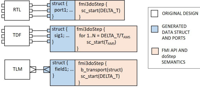
Fig. 2. Wrapping strategy at RTL, TDF, and TLM abstraction levels. Port aggregation structs are auto-generated per model, and fmi3DoStep semantics are adapted to each abstraction's timing model.
