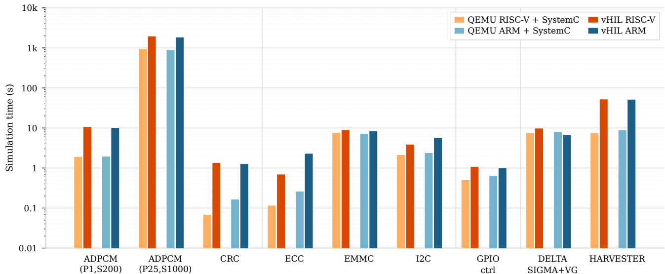
Fig. 5. Comparison of QEMU + native SystemC co-simulation against the full vHIL framework on both RISC-V and ARM targets.
