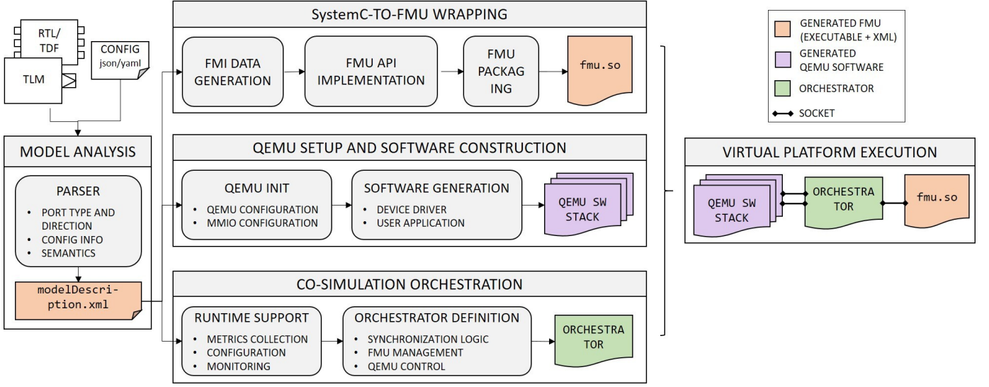
Fig. 1. Overview of the SystemC-to-FMU toolchain and vHIL integration, highlighting the role of the orchestration layer in coordinating QEMU, FMU, and SystemC. Starting from the initial SystemC description and a configuration file, model analysis (left) drives automated FMU generation (top) and QEMU-based platform construction (middle). An orchestrator is then defined (bottom) to combine FMU and QEMU at runtime for vHIL execution.
