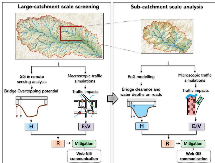
Figure 1 - Workflow of the multi-scale assessment of bridge risk derived from overtopping hazard and traffic impacts.
