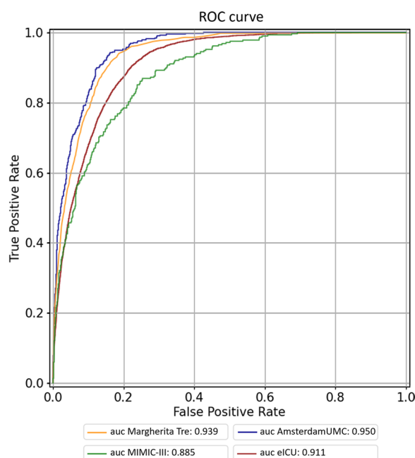
Fig. 2 auROC curves of retrospective validation sets. auROC: area under receiver operating characteristic curve
