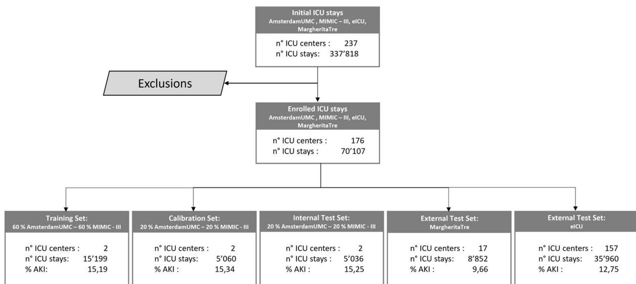
Fig. 1 Scheme of data split into different sets. No ICU stays: Number of ICU stays associated with unique patients in each dataset
