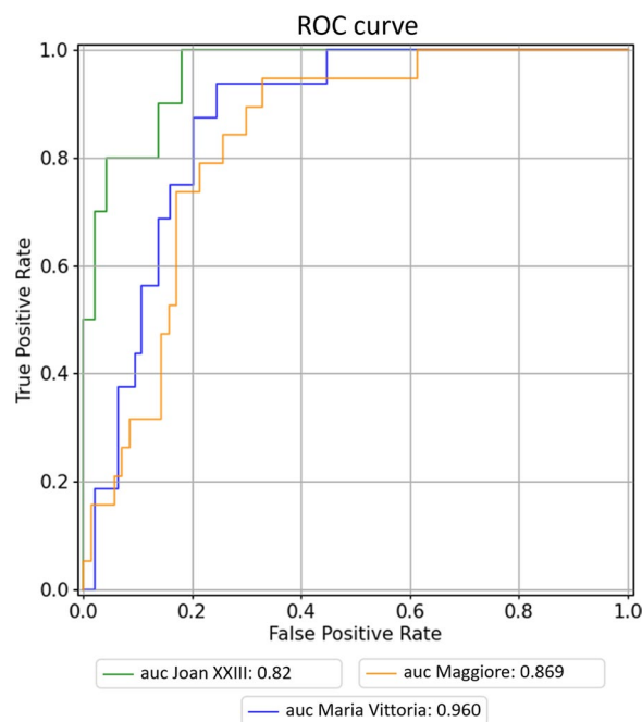
Fig. 3 auROC curves of prospective validation sets. auROC: Area under receiver operating characteristic curve
