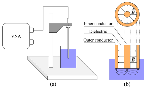
Fig. 1. Open-ended coaxial probe technique: (a) Measurement set-up; (b) cross-sections of the coaxial probe.
