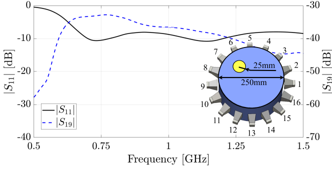
Fig. 1. Simulated scattering parameters, |S_{11}| and |S_{19}| , for the 16-antenna circular array with a geometry schematic and dimensions included in the bottom-right corner scheme. Permittivity values based on [3].
