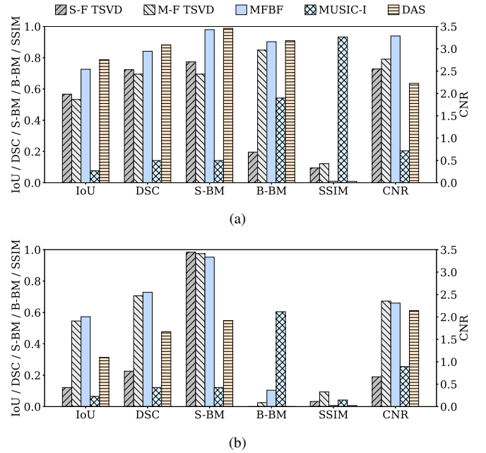
Fig. 2. Performance metrics of (a) full-multiplexing and (b) partial-multiplexing configuration
