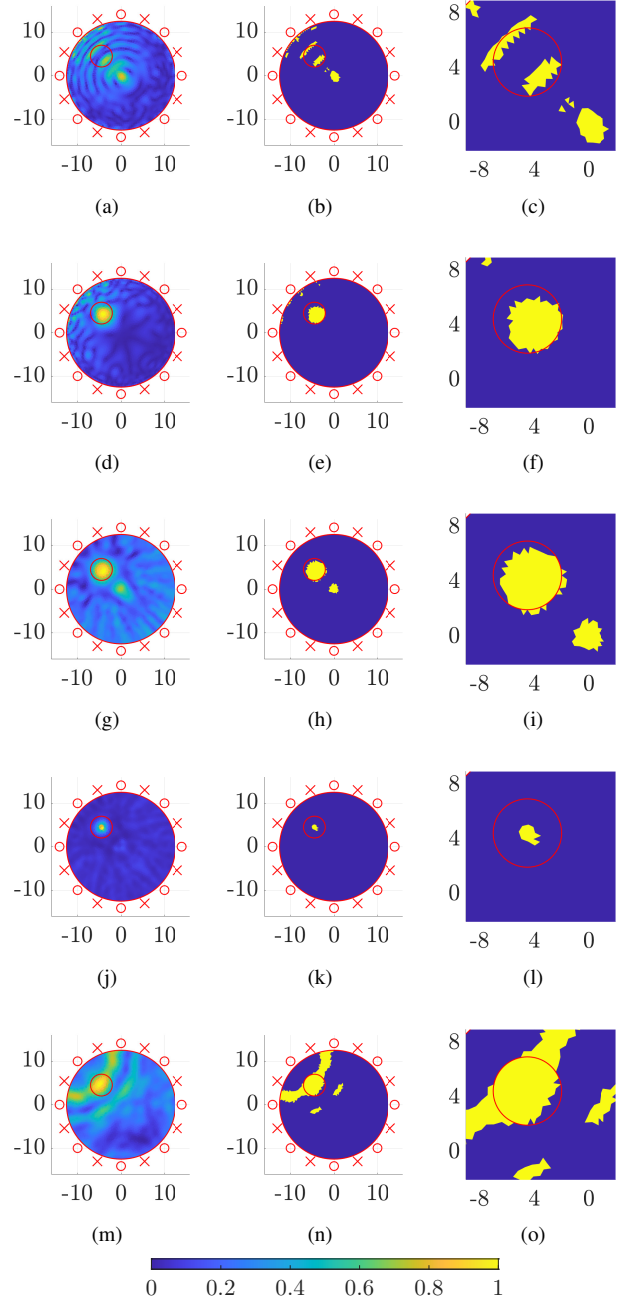
Fig. 4. Normalized reconstructions for the partial-multiplexing configuration using different MWI algorithms. (a-c) S-F TSVD, @1GHz; (d-f) M-F TSVD; (g-i) MFBF; (j-l) MUSIC-I; (m-o) DAS. Each row shows: (left) normalized reconstruction; (middle) binary mask by thresholding the reconstruction at 0.563 ( \approx 5 dB); (right) a zoom-view of the target region. Dimensions in [cm]. The internal red contour outline the hotspot area. The red crosses indicate the positions of the phase center of the transmitters, while the circles indicate the receivers.
