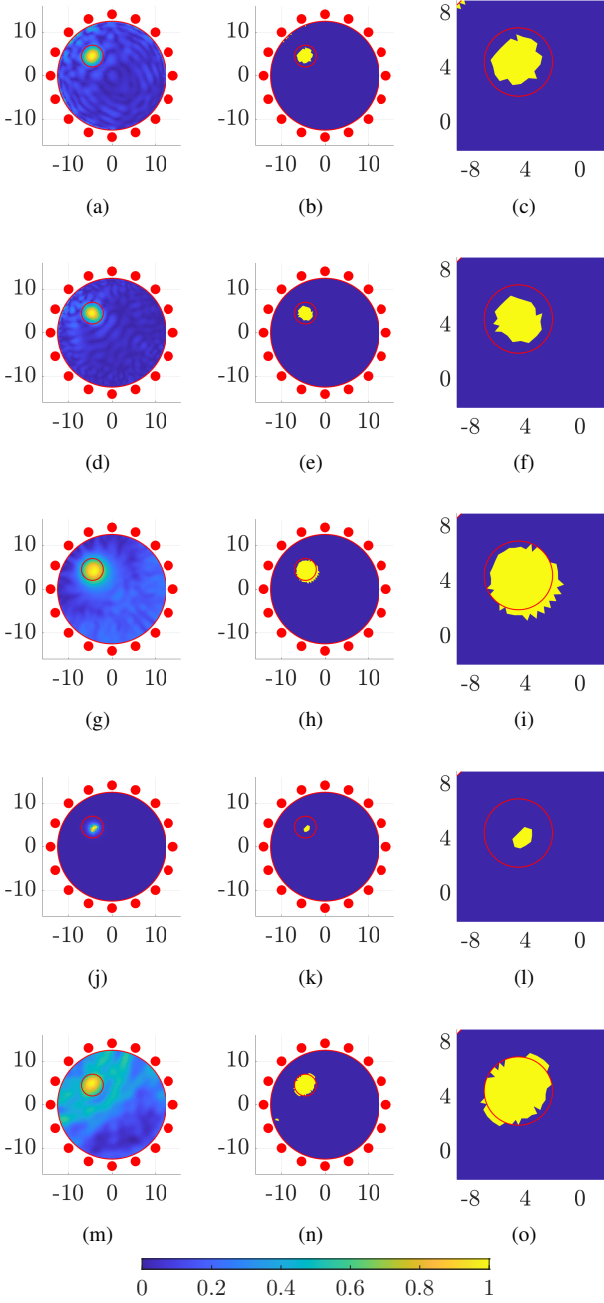
Fig. 3. Normalized reconstructions for the full-multiplexing configuration using different MWI algorithms (a-c) S-F TSVD, @1GHz; (d-f) M-F TSVD; (g-i) MFBF; (j-l) MUSIC-I; (m-o) DAS. Each row shows: (left) normalized reconstruction; (middle) binary mask by thresholding the reconstruction at 0.563 ( \approx 5 dB); (right) a zoom-view of the target region. Dimensions in [cm]. The internal red contour outline the hotspot area. The red points indicate the positions of the phase center of the transceiver elements.
