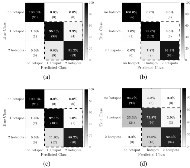
Fig. 3. Confusion matrices on tested data for different SNR values: (a) 70 dB, (b) 50 dB, (c) 30 dB, (d) 10 dB.
