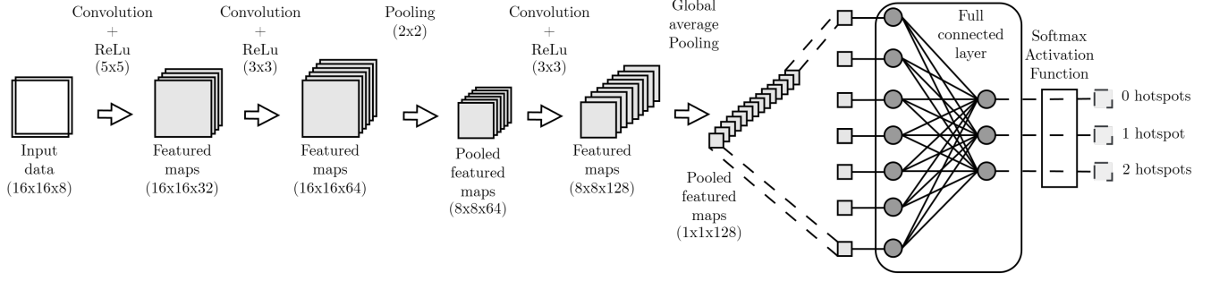
Fig. 2. Proposed 2D-CNN architecture for three-class hotspot classification
