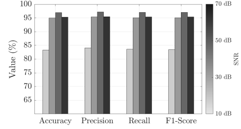
Fig. 4. Comparison of classification performance on tested data for different SNR values: 10dB, 30dB, 50dB and 70dB.
