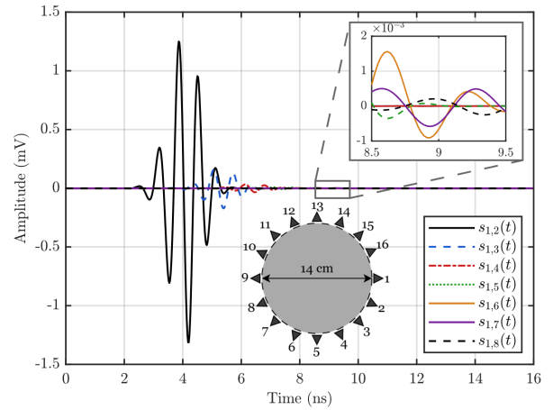
Fig. 1. Time-domain multi-static scattered signals of the simulated scenario, homogeneous dielectric permittivity of the background medium (compost).
