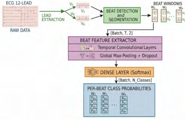
Fig. 2. Overview of the proposed beat-level classification pipeline from raw ECG signals to class probabilities.
