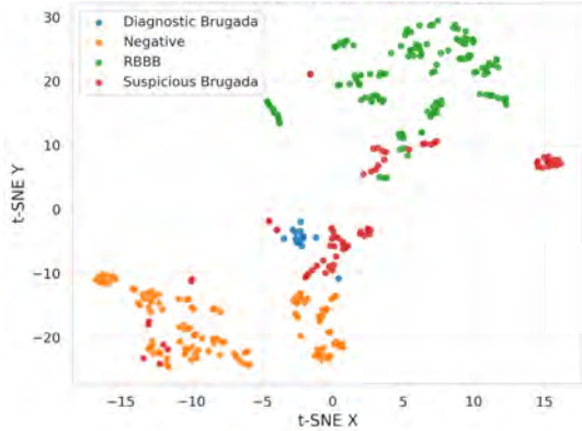
Fig. 4. t-SNE projection of beat-level features extracted by the 4-class model on the representative test set.
