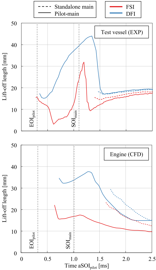
Fig. 9. Time evolution of lift-off length from vessel experiments (top) and engine simulations (bottom) for FSI (red) and DFI (blue) configurations. Solid lines represent pilot injection cases, while dashed lines correspond to standalone main cases. Pilot-main scheme: DT_{pilot} = 0.7 ms (i.e., 5 CA deg) and m_{f,pilot}\% = 10\% (i.e., 2.3 mg) for engine, DT_{pilot} = 0.8 ms and m_{f,pilot} = 2.5 mg for vessel. (For interpretation of the references to colour in this figure legend, the reader is referred to the web version of this article.)
