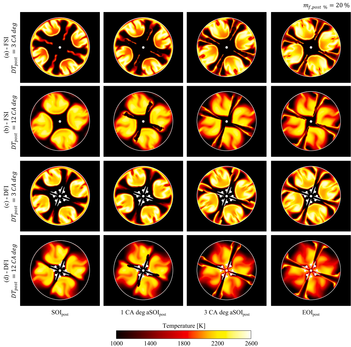
Fig. 14. Temperature distribution on a plane containing the spray axis for the FSI and DFI configurations at different time instants (from left to right), in the case with post-injection featuring m_{f,post}\% = 20\% . Results are shown for FSI with DT_{post} = 3 CA deg (a) and 12 CA deg (b), and for DFI with DT_{post} = 3 CA deg (c) and 12 CA deg (d).
