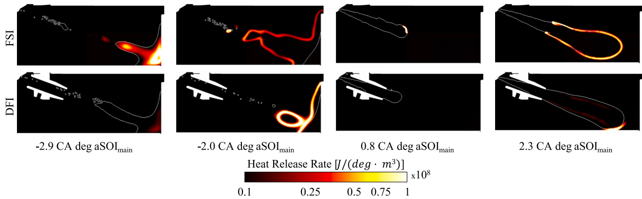
Fig. 7. Heat release rate (HRR) distribution shown on a logarithmic scale in a vertical plane including the injector and spray axes in the pilot-main scheme with DT_{pilot} = 5 CA deg and m_{f,pilot\%} = 10\% , for both FSI (top) and DFI (bottom) configurations at different time instants ( -2.9 deg aSOI_{main} , -2.0 deg aSOI_{main} , 0.8 deg aSOI_{main} and 2.3 deg aSOI_{main} ). The isoline representing fuel injection corresponds to an overall equivalence ratio of 1.
