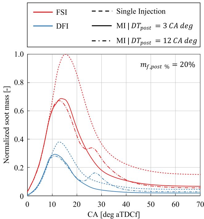
Fig. 13. Normalized soot mass as a function of the crank angle, for both FSI (red) and DFI (blue) for the standalone main case (dashed line) and main-post cases with DT_{post} = 3 CA deg (solid line) and DT_{post} = 12 CA deg dwell time (dash-dot line) and m_{f,post}\% = 20\% . (For interpretation of the references to colour in this figure legend, the reader is referred to the web version of this article.)
