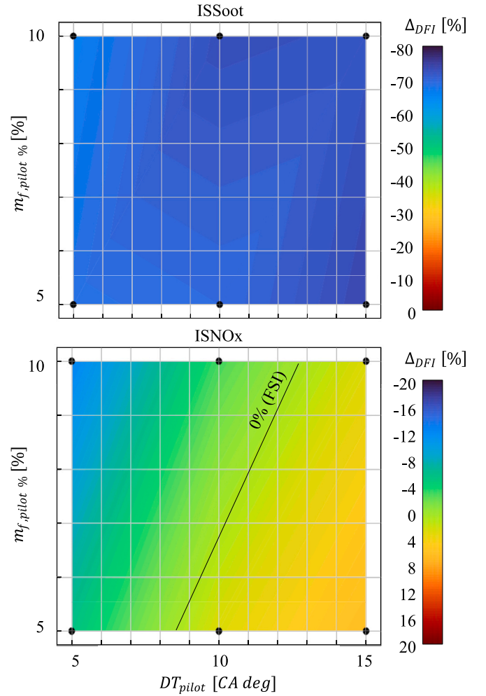
Fig. 4. Percentage difference between DFI and FSI configurations for the MI case (pilot-main injection) as a function of DT_{pilot} and m_{f,pilot\%} , for indicated specific soot (top) and NOx (bottom) emissions.
