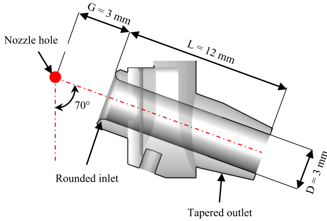
Fig. 1. Sketch of the D3L12G36 duct design.
