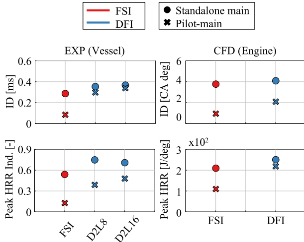
Fig. 6. Experimental vessel-derived data (left) and engine simulation results (right) for ignition delay (ID, top) and peak heat release rate (HRR) of the premixed burn phase (bottom) of the main injection. FSI configuration results are shown in red, DFI in blue. Standalone main injection strategy is represented by circle markers, while pilot-main injection scheme is indicated by X markers. Pilot-main scheme: DT_{pilot} = 0.8 ms and m_{f,pilot} = 2.5 mg for vessel, DT_{pilot} = 0.7 ms (i.e., 5 CA deg) and m_{f,pilot} = 10\% (i.e., 2.3 mg) for engine. Details on the experimental campaign in [32]. (For interpretation of the references to colour in this figure legend, the reader is referred to the web version of this article.)
