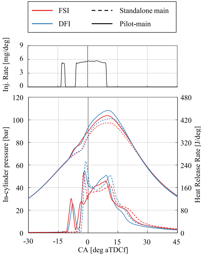
Fig. 5. Injection rate (top), in-cylinder pressure and heat release rate (bottom) for both FSI (red) and DFI (blue). Standalone main case shown as dashed lines, pilot-main case ( DT_{pilot} = 5 CA deg and m_{f,pilot} = 10\% m_{f,tot} ) as solid lines. (For interpretation of the references to colour in this figure legend, the reader is referred to the web version of this article.)
