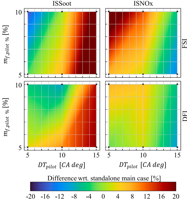
Fig. 3. Percentage difference between the multi-injection case (pilot-main injection) and standalone main case as a function of DT_{pilot} and m_{f,pilot\%} , for indicated specific soot (left) and NOx (right) emissions, for both FSI (top) and DFI (bottom) configurations.
