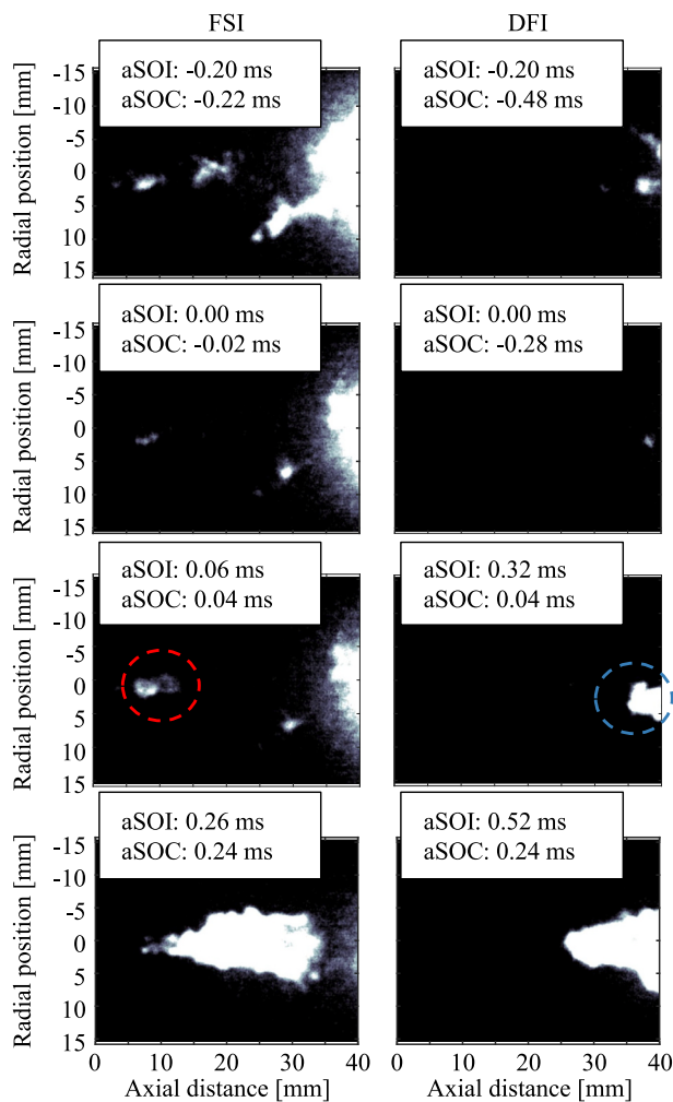
Fig. 8. Experimental OH^* chemiluminescence images for (left) FSI and (right) DFI (D2L8 configuration) captured at four time instants for the pilot-main injection scheme: (from top to bottom) combustion recession of the pilot combustion at 0.2 ms before SOI_{main} ; SOI_{main} ; SOC main ; developed flame at 0.24 ms aSOC_{main} . Circle markers indicate the ignition location of the main injection.
