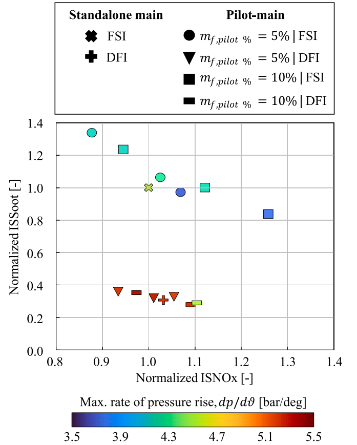
Fig. 10. Scatter plot of maximum rate of pressure rise, used as a combustion noise indicator, on a normalized indicated specific soot-NOx diagram. Standalone main cases are shown with X markers for FSI and cross markers for DFI configurations. Multiple injection cases are represented with circles for FSI and m_{f,pilot}\% = 5\% , triangle markers for DFI and m_{f,pilot}\% = 5\% , square markers for FSI and m_{f,pilot}\% = 10\% , and rectangular markers for DFI and m_{f,pilot}\% = 10\% .
