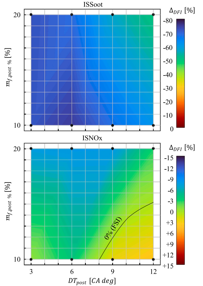
Fig. 12. Percentage difference between DFI and FSI configurations for the MI case (main-post injection) as a function of DT_{post} and m_{f,post\%} , for indicated specific soot (top) and NOx (bottom) emissions.
