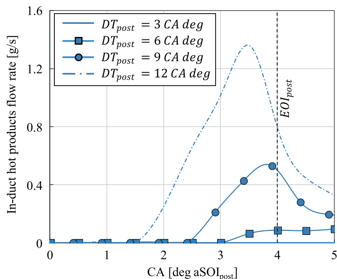
Fig. 15. In-duct entrainment of hot gases for MI cases featuring m_{f,post} = 20\% and a DT_{post} = 3 CA deg (solid line), DT_{post} = 6 CA deg (square-marked solid line), DT_{post} = 9 CA deg (circle-marked solid line) and DT_{post} = 12 CA deg (dash-dot line).
