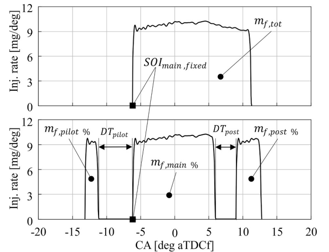
Fig. 2. Schematic illustration of the original single-injection profile (top) and derived multi-injection pattern (bottom), covering both pilot-main and main-post injection configurations.
