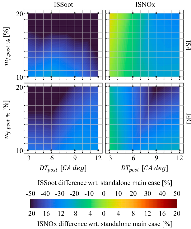
Fig. 11. Percentage difference between the multi-injection case (main-post injection) and standalone main case as a function of DT_{post} and m_{f,post\%} , for indicated specific soot (left) and NOx (right) emissions, for both FSI (top) and DFI (bottom) configurations.
