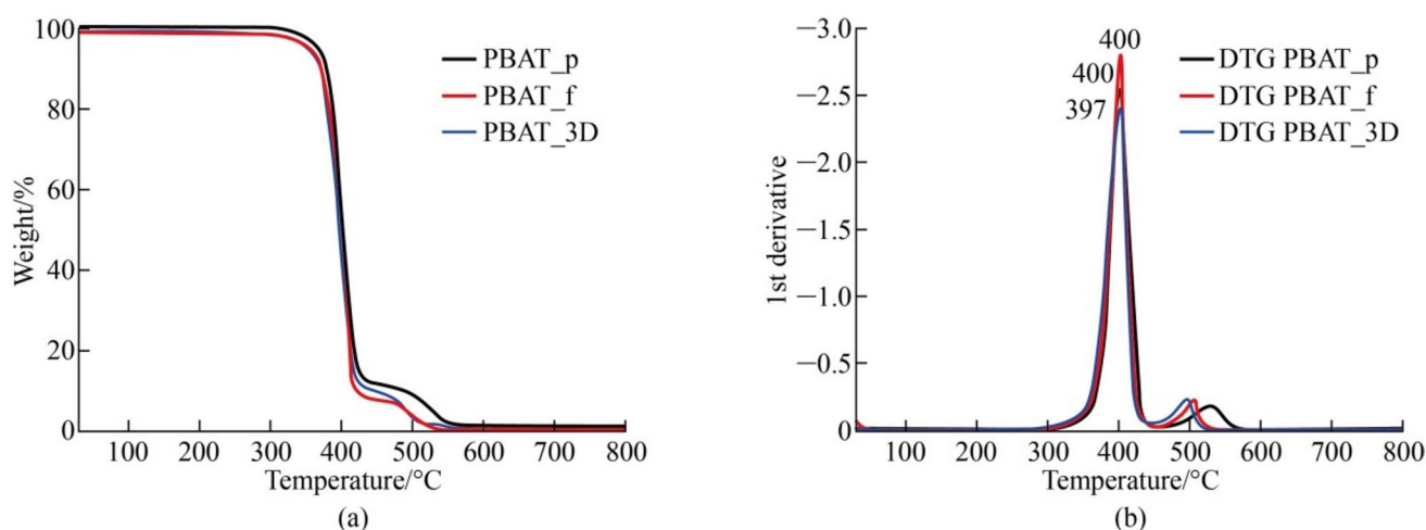
Fig. 3 a TG and b DTG curves of PBAT samples: pellet, filament, and printed
