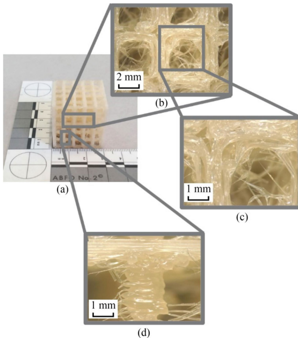
Fig. 8 a Macroscopic view of a PHBH printed lattice structure, b thin surface membranes and filament webbing, c stringing and bridging sagging between lattice struts, d detail of filament deposition and surface irregularities
