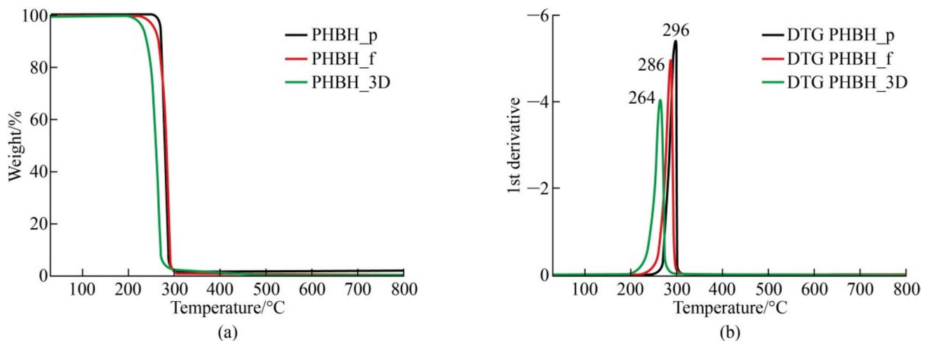
Fig. 2 TG and DTG curves of PHBH: pellet, filament, and printed
