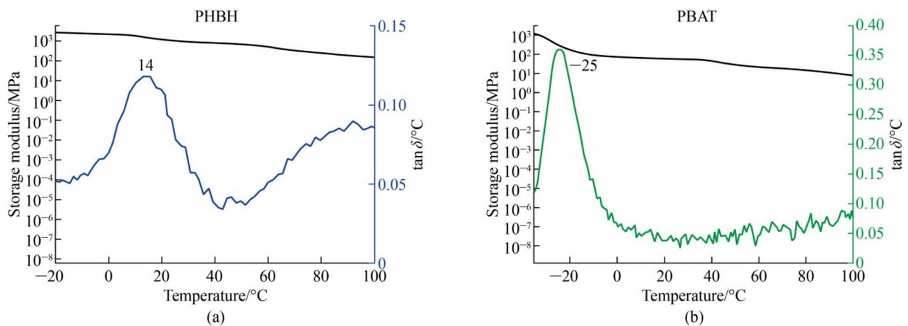
Fig. 6 DMA curves of a PHBH and b PBAT 3D-printed parts realized by FFF
