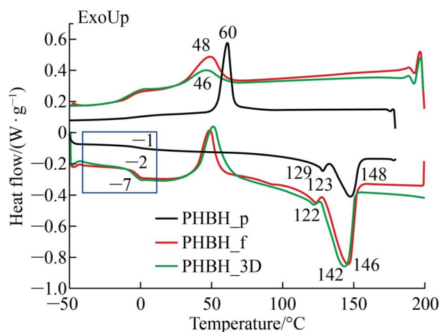
Fig. 4 DSC curves PHBH samples: pellet, filament, and printed via FFF
