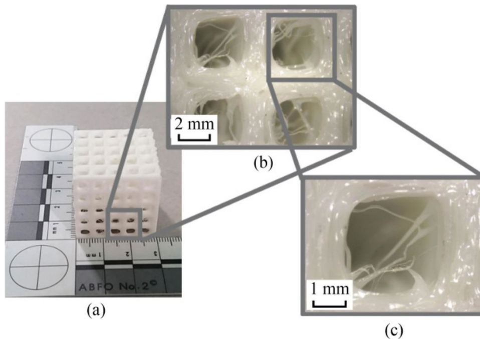
Fig. 10 a Macroscopic view of a PBAT printed lattice structure, b magnified view of lattice pore morphology, and c detail of minor filament stringing inside lattice cells
