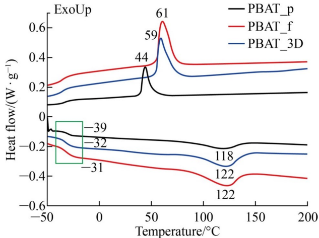
Fig. 5 DSC curves PBAT samples: pellets, filament, and printed via FFF
