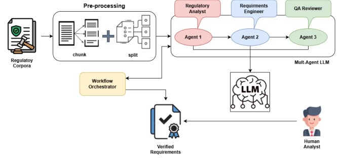
Fig. 1. System overview: regulatory corpora are preprocessed into chunks; B5 runs three sequential agent roles via CrewAI on a shared Ollama Llama 3 8B endpoint; outputs are evaluated against expert gold.
