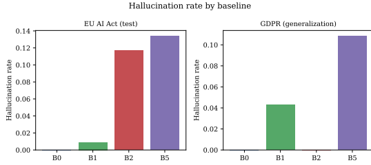
Fig. 6. Hallucination rate comparison across baselines (EU AI Act test and GDPR generalization).
