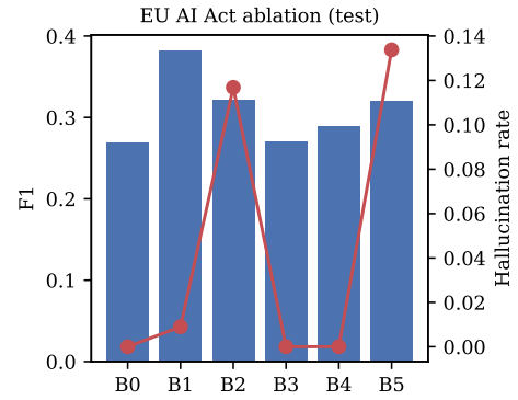
Fig. 7. EU AI Act ablation (B0–B5).
