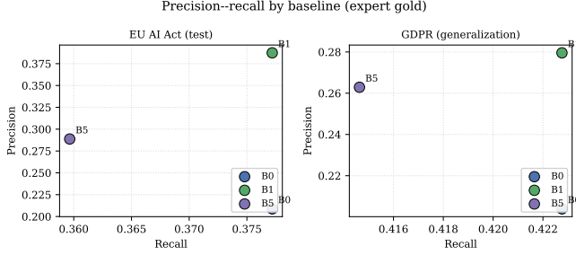
Fig. 2. Precision-recall landscape (B0, B1, B5).
