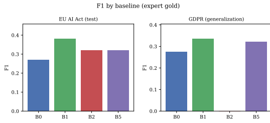
Fig. 5. F1 comparison across baselines (EU AI Act test and GDPR generalization).
