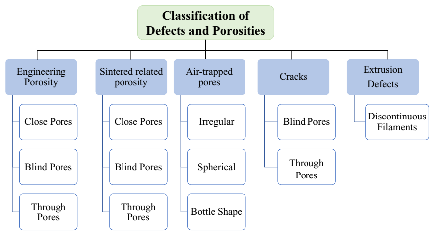
FIGURE 27 | Type of porosities in AM of advanced ceramic.
