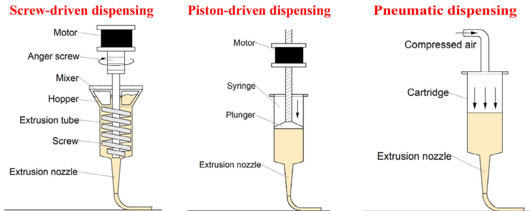
FIGURE 2 | Schematic illustration of the main nozzle configurations used in slurry-based extrusion 3D printing.
