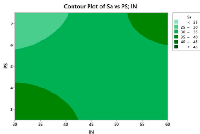
FIGURE 9 | Mean arithmetical roughness S_a ( \mu\text{m} ) as a function of infill and printing speed plotted conturally. Reproduced with permission [164]. Copyright 2020, MDPI.
