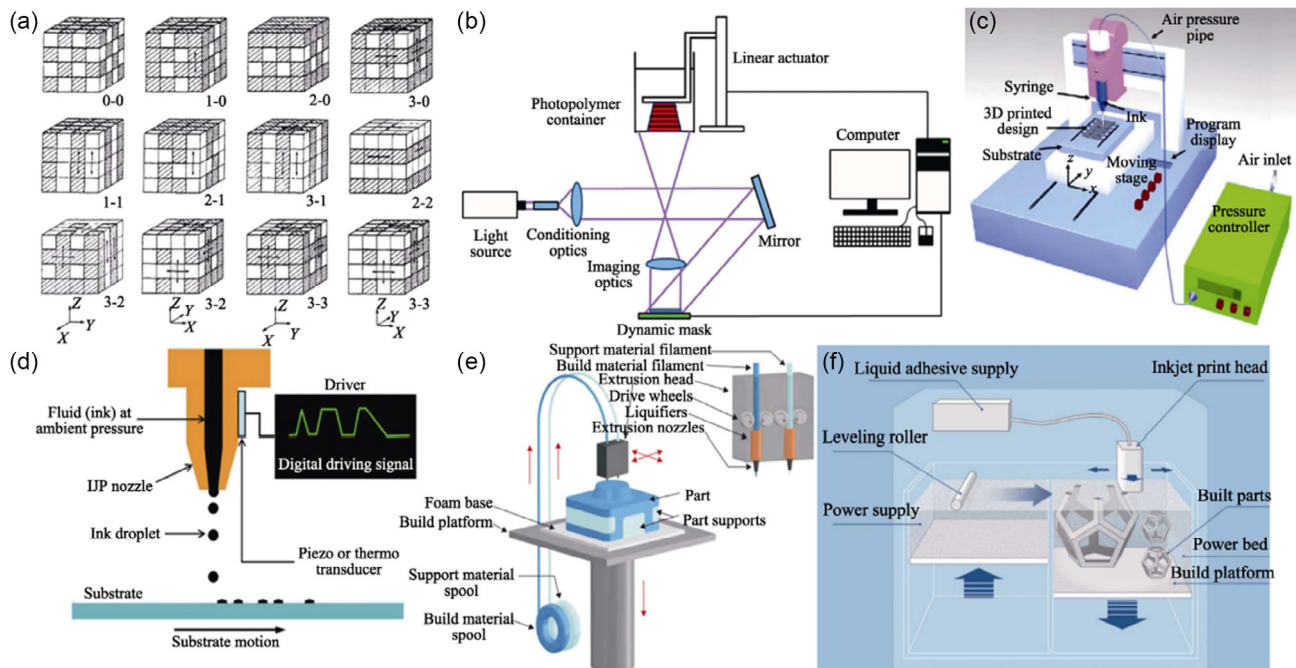
FIGURE 26 | Connections of piezoelectric ceramics and graphic representations of commonly utilized additive manufacturing techniques for the preparation of piezoelectric ceramics. Reproduced with permission [258]. Copyright 2022, Science Press.
