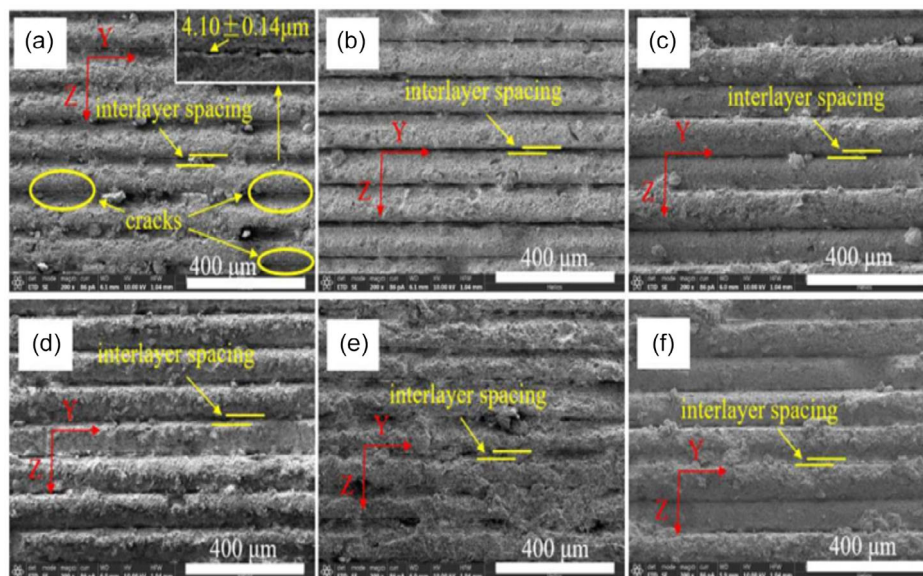
FIGURE 16 | Scanning electron microscope (SEM) images of an alumina part made by stereolithography placed at different times of heat treatment (a: 30 min, b: 60 min, c: 90 min, d: 120 min, e: 150 min, f: 180 min). Reproduced with permission [237]. Copyright 2020, Frontiers.
