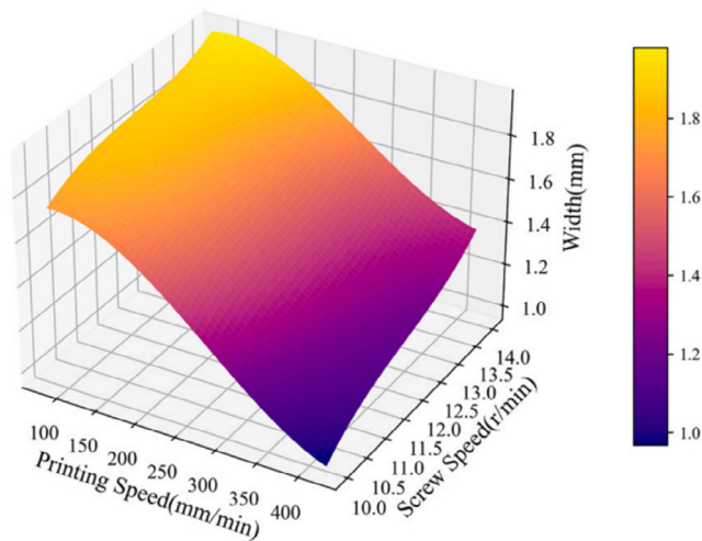
FIGURE 10 | Response surface showing the influence of print speed and screw rotation speed on deposition line width. Reproduced with permission [164]. Copyright 2020, MDPI.
