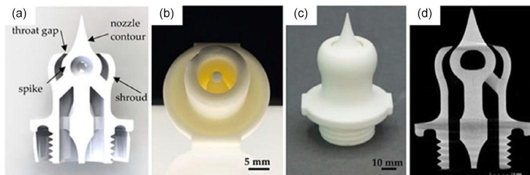
FIGURE 25 | \text{Al}_2\text{O}_3 nozzles produced via additive manufacturing utilizing the CeraFab 7500 printing apparatus. Sectional representation of an aerospike nozzle (a), 2.5 N nozzle (b), 10 N nozzle (c), and computed tomography image of the 10 N nozzle (d). Reproduced with permission [253]. Copyright 2022, MDPI.
