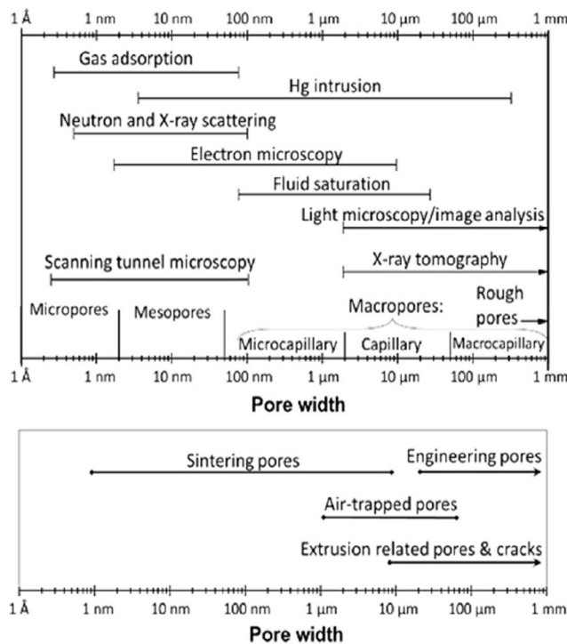
FIGURE 28 | Investigation of porosities and defects length in EAM ceramics. Reproduced with permission [37]. Copyright 2021, Elsevier.
