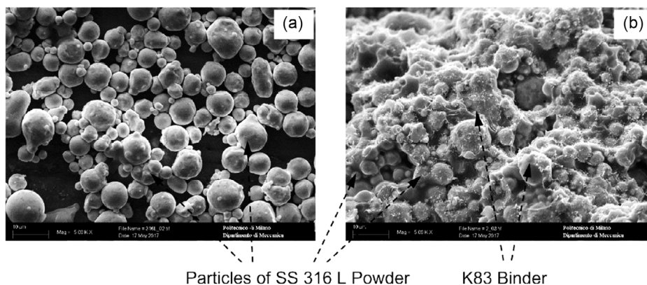
FIGURE 7 | SEM images of (a) SS316L powder and (b) the fractured surface of a feedstock pellet with a solid loading of SS316L powder. Reproduced with permission [104]. Copyright 2019, Elsevier.
