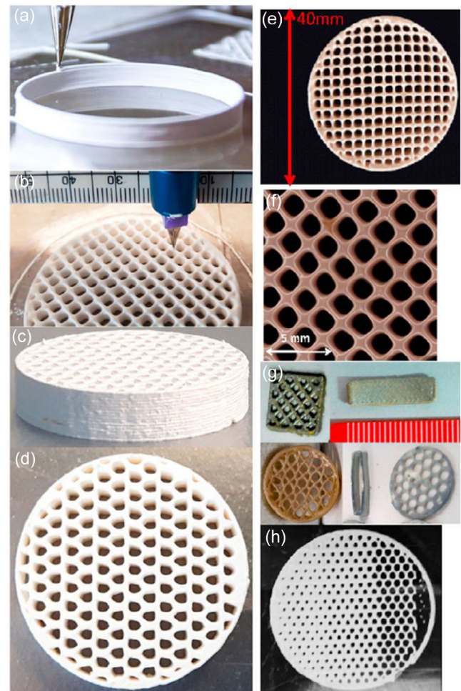
FIGURE 24 | (a) Image of a hollow circular heating element in the printing process, (b) image of the RC nozzle 3D printing the foundational layers of a honeycomb heating element (50 mm diameter), (c) lateral perspective of green printed BT honeycomb specimen, (d) superior perspective of green printed BT honeycomb specimen, (e) top view optical micrograph of a sintered full-size honeycomb heating element, (f) optical micrograph of a sintered heating element featuring a square grid structure, (g) images of typical circular, elliptical, square, and rectangular strip-printed heating elements exhibit customizable porosity, and (h) a 3D-printed green sample featuring a graded porous structure. Reproduced with permission [252]. Copyright 2019, Elsevier.
