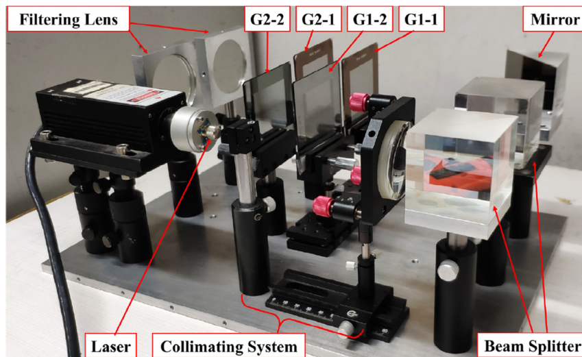
FIGURE 8 | Schematic representation of the customized coherent gradient sensing (CGS) system used for in situ process monitoring. Reproduced with permission [147]. Copyright 2020, Elsevier.
