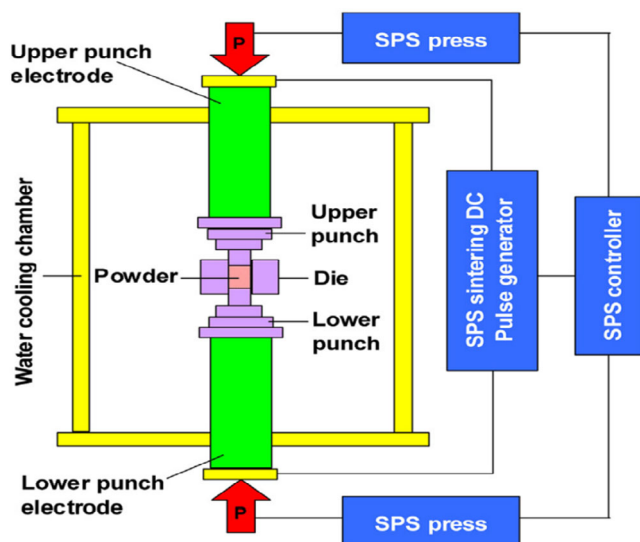
FIGURE 12 | Schematic of the SPS process. Reproduced with permission [210]. Copyright 2014, Elsevier.
