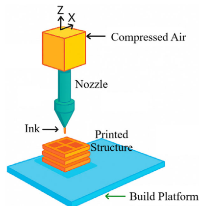
FIGURE 5 | Schematic diagram of DIW used for manufacturing ceramic parts.
