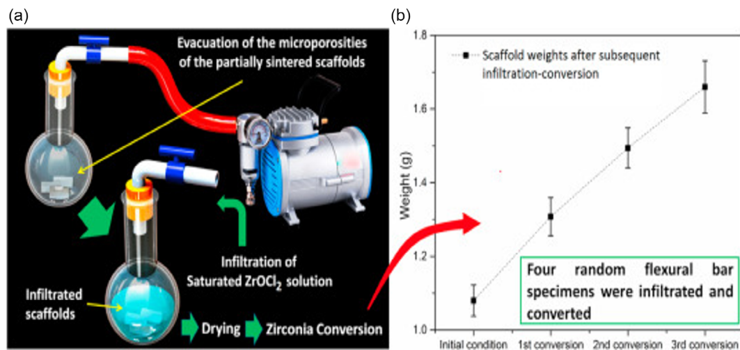
FIGURE 18 | (a) Schematic of infiltration of saturated \text{ZrOCl}_2 solution in zirconia-alumina-based ceramics and (b) diagram of weight-infiltration cycle that as a result by increasing the infiltration cycle, the weight of ceramic increased. Reproduced with permission [236]. Copyright 2020, Elsevier.
