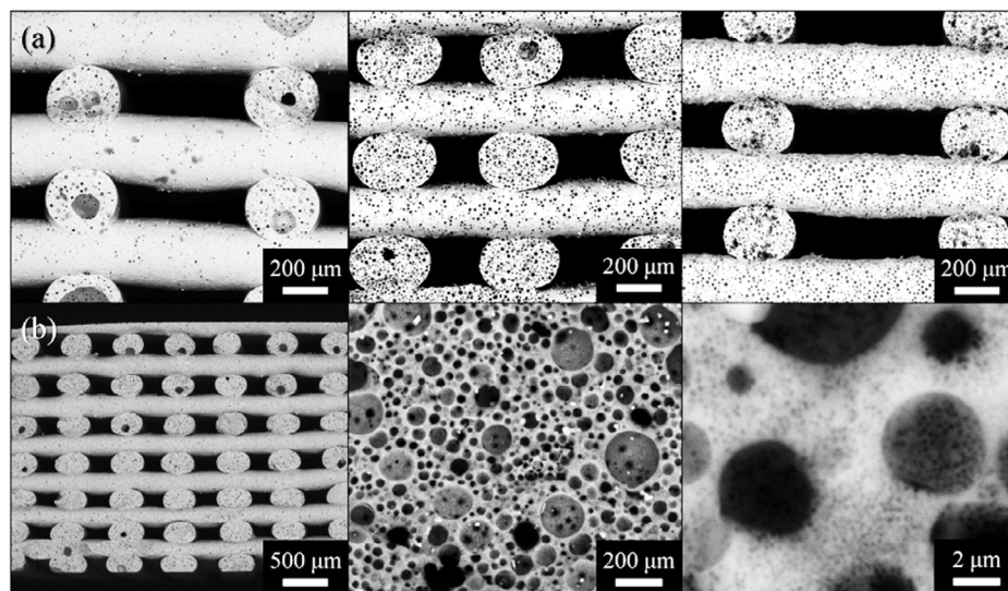
FIGURE 6 | SEM images of: (a) SiOC pyrolyzed porous scaffolds printed via DIW, derived from the removal of varying amounts of PMMA particles (50, 60, and 80 vol%); and (b) a SiOC scaffold exhibiting a hierarchical pore structure, obtained by combining PMMA particles of different nominal sizes (25 and 0.46 \mu\text{m} ). Reproduced with permission [103]. Copyright 2022, Elsevier.
