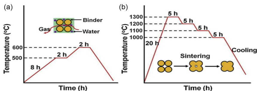
FIGURE 14 | Heat treatment cycle applied to (a) debinding and (b) sintering barium titanate component. Reproduced with permission [235]. Copyright 2020, Elsevier.
