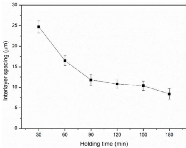
FIGURE 17 | Variation in interlayer spacing of stereolithography-fabricated alumina parts as a function of heat-treatment duration. Reproduced with permission [237]. Copyright 2020, Frontiers.
