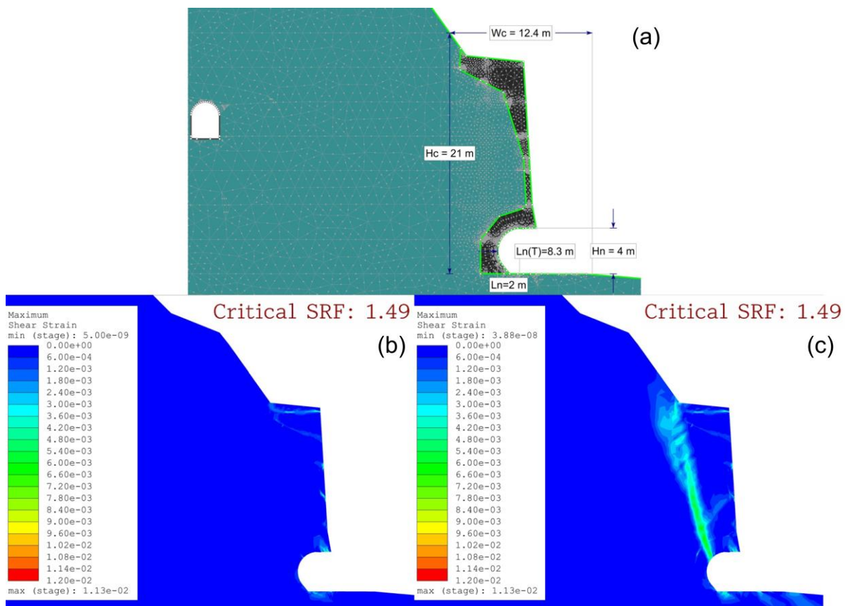
Figure 4. (a) Post-collapse cliff geometry used for the forecasting scenario; (b) maximum shear strains; (c) progressive increase of the maximum shear strain up to limit conditions.
