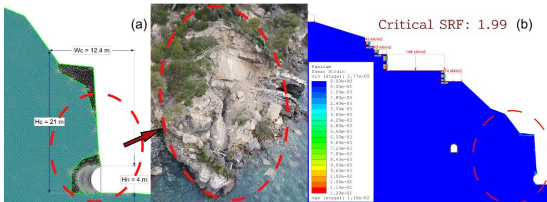
Figure 3. (a) Cliff geometry used for the current (post-collapse) scenario, together with a field photograph of the post-rockfall condition; (b) maximum shear strains.
