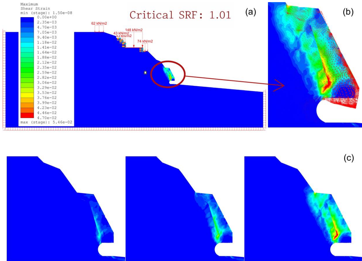
Figure 2. Maximum shear strain contours and critical SRF (a); maximum total displacements (b); evolution of the maximum shear strains with the progressive retreat of the notch (c).
