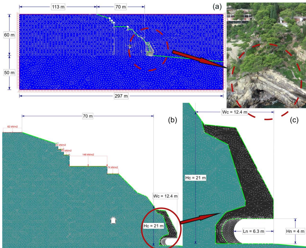
Figure 1. Numerical model setup: (a) overall geometry, dimensions, and boundary conditions, together with a field photograph of the cliff and basal notch; (b) applied external actions represented as equivalent uniformly distributed loads (building floors and road surfaces); (c) detail of the cliff-toe region showing the cliff geometry ( H_c , W_c ) and notch geometry ( H_n , L_n ), with local mesh refinement. The black layer represents the weathered rock layer.
