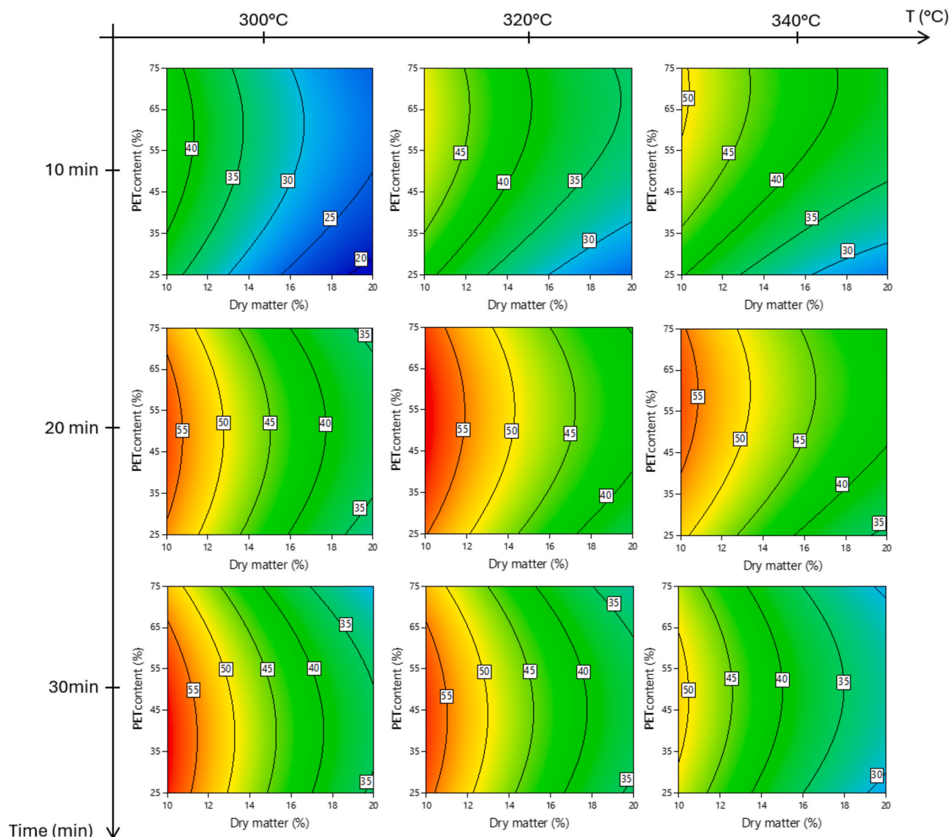
Fig. 5. Contour plot of EG yield DoE.
