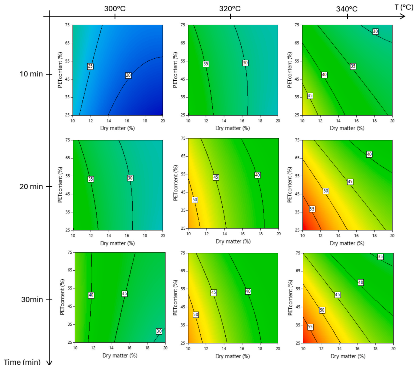
Fig. 6. Contour plot of CL yield.
