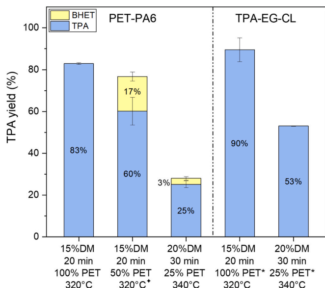
Fig. 4. Influence of specific reaction conditions on TPA and BHET yield (♦ has been replicated 12 times instead of 2). Asterisks (*) indicate values expressed as monomer equivalents relative to the initial polymer mass.
