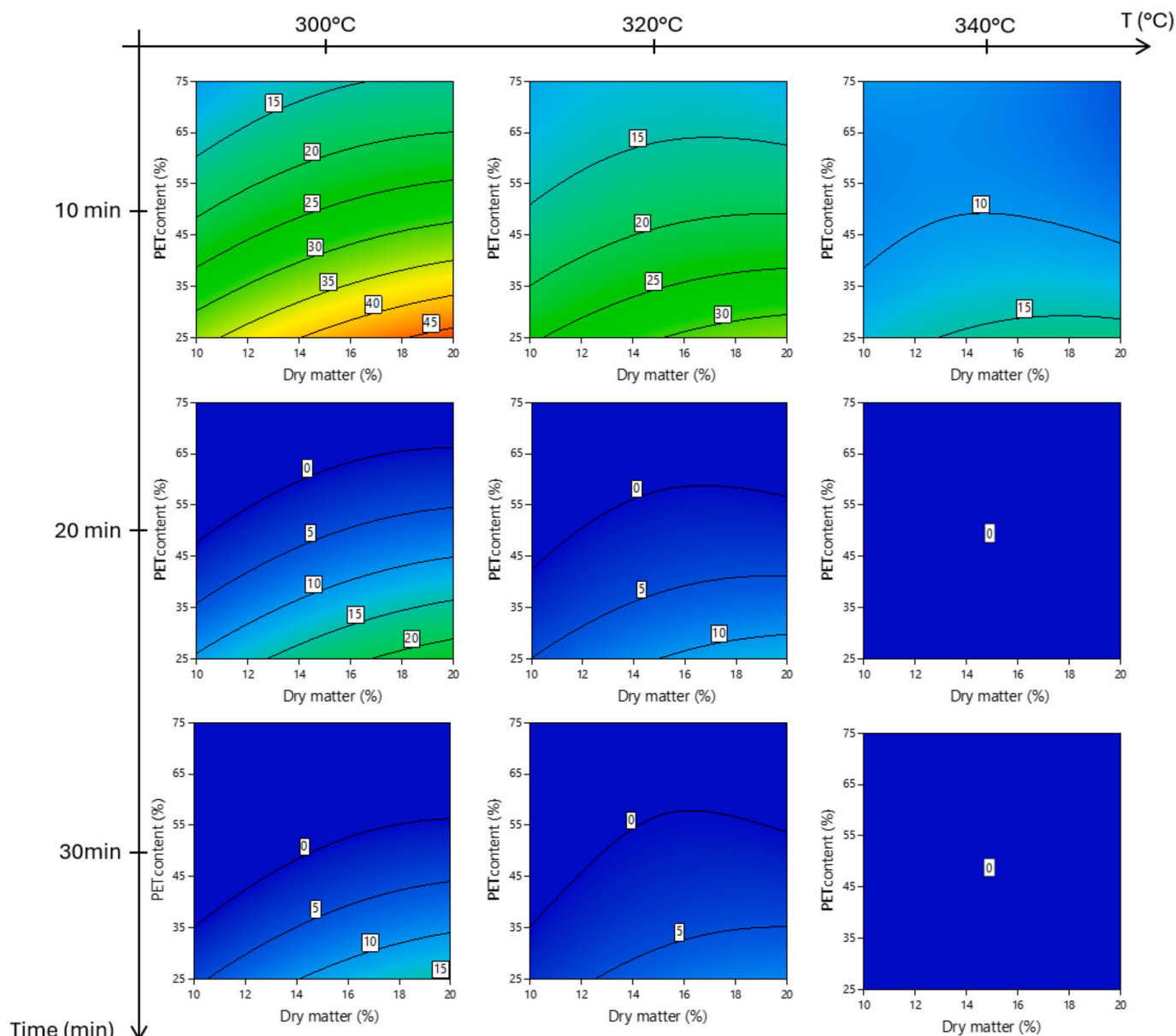
Fig. 1. Contour plot of RS yield.
