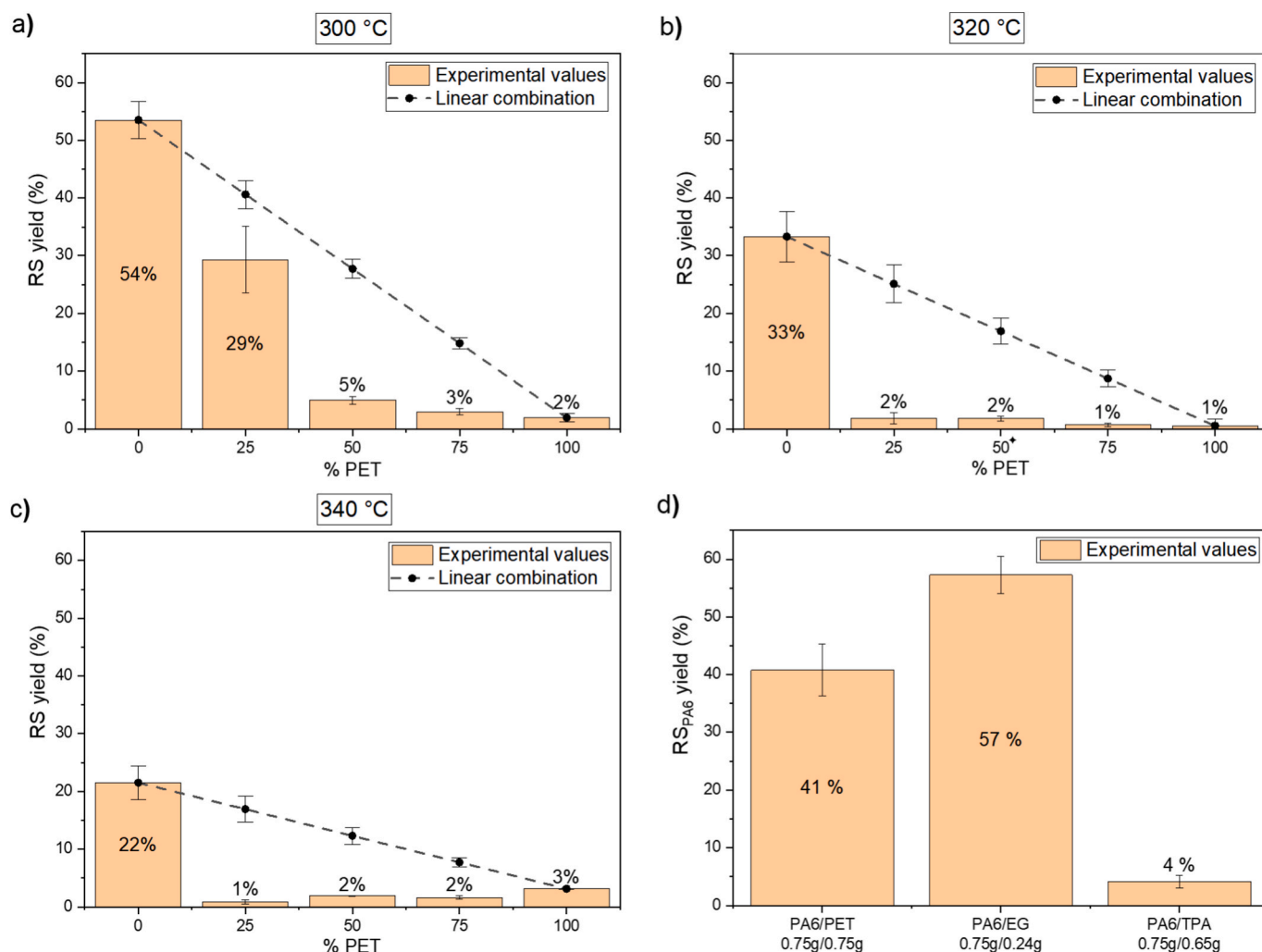
Fig. 2. Influence of PET content on RS yield at different temperatures: (a) 300 °C, (b) 320 °C (♦ has been replicated 12 times instead of 2), and (c) 340 °C. Operating conditions: reaction time 20 min, DM 15%. (d) Influence of the PA6 co-feed component (PET, EG or TPA) on RS_{PA6} yield. Operating conditions: reaction temperature 300 °C, DM 15%, reaction time 10 min.
