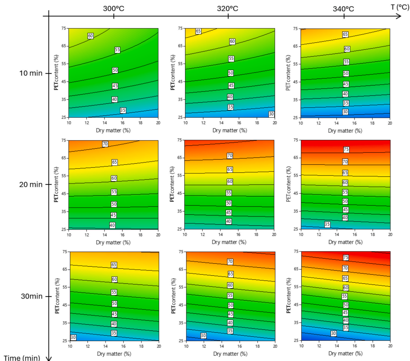
Fig. 3. Contour plot of TPA yield.
