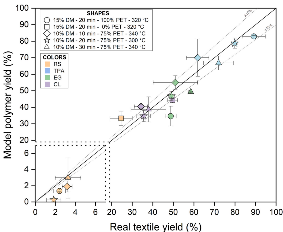
Fig. 9. Comparison of experimentally-obtained product yields from textiles and model polymers under different conditions. Dotted lines refer to \pm 10\% deviation from bisector.
