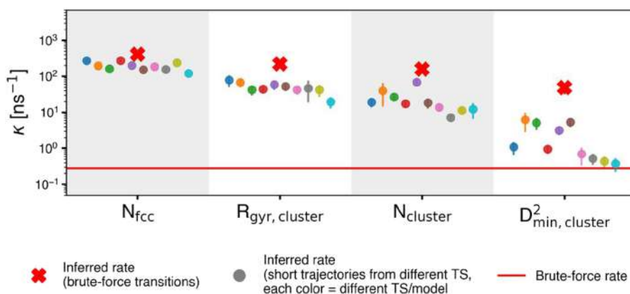
FIG. 5. Comparison of kinetic rates as a function of the order parameters, using different approaches. The solid red line represents the rate directly observed from brute-force simulations initialized in the initial basin A. The red crosses and the colored dots correspond to estimations obtained from stochastic models. In the case of red crosses, the models were built using all spontaneous transitions. In the case of colored dots, the models were inferred from short trajectories initialized from ten different transition-state configurations (TSs), each color referring to a distinct TS-based model. Improved order parameters yield more accurate rate estimations, with the inferred rates systematically converging toward the brute-force value.
