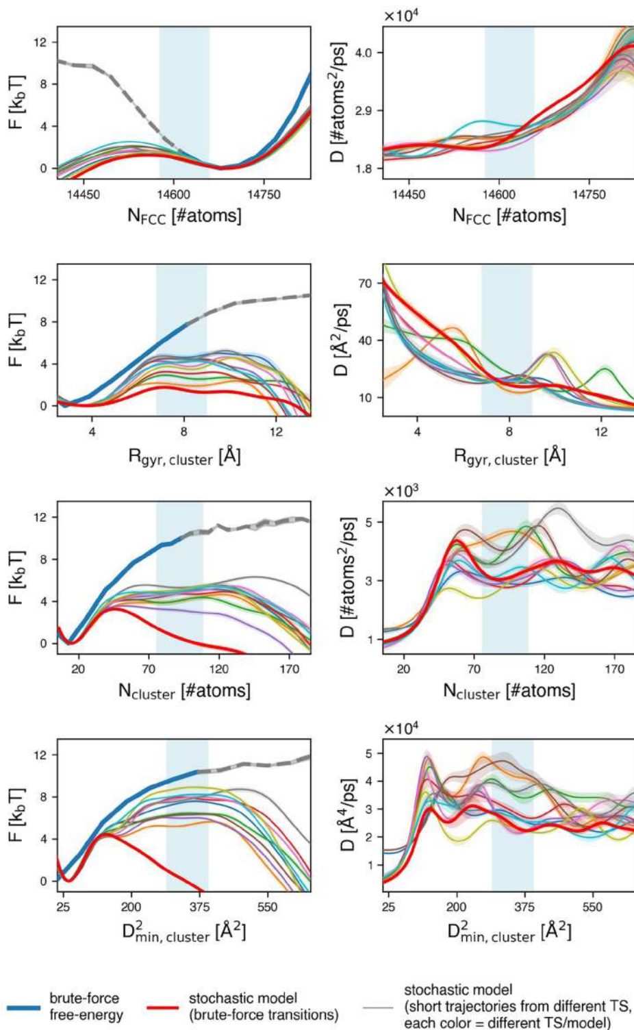
FIG. 4. Estimated profiles of free-energy ( F ) and diffusion-coefficient ( D ) obtained using a Langevin model for various order parameters. The thick red line represents the inferred profiles from spontaneous brute-force transitions, while the thin colored lines correspond to models constructed from trajectories initialized at ten randomly selected transition states. The solid blue line shows the brute-force free-energy estimate, for comparison. The shaded light blue region highlights the transition state region.
