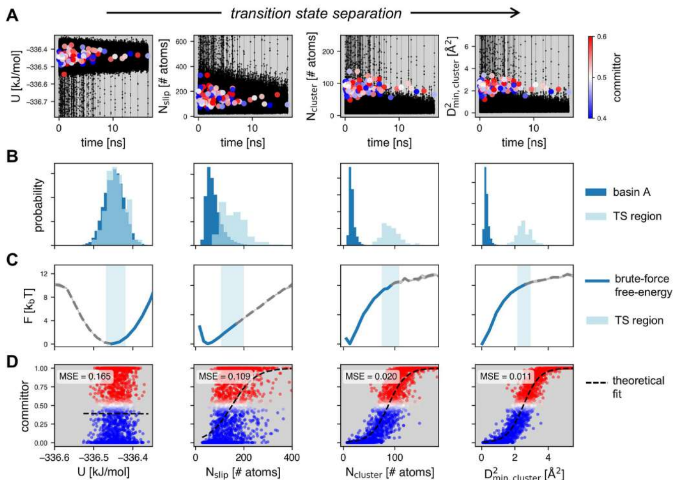
FIG. 3. (a) Reactive trajectories illustrating the evolution of the order parameters over time. Scatter points highlight the transition states, with colors representing the committor probability. (b) Probability histograms for the initial basin (blue) and the transition-state region (light blue) with committor probability between 0.4 and 0.6. (c) Free-energy barrier estimates as a function of the order parameters. The solid blue curve represents the equilibrium free-energy profile, while the dashed gray curve extends the profile in the out-of-equilibrium region beyond the transition. The blue shaded region highlights the transition-state region. (d) Committor probability as a function of the order parameters. The dashed line shows an analytical fit obtained using a logistic function, with the corresponding mean squared error.
