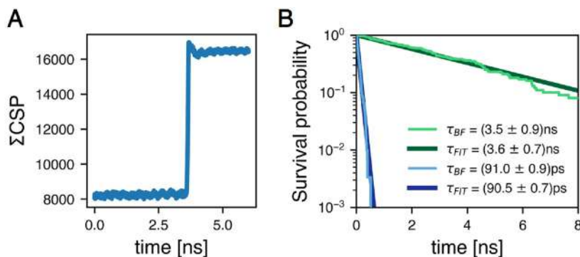
FIG. 2. (a) Example of time evolution of an order parameter ( \Sigma\text{CSP} ), illustrating the separation between state A (initial crystalline metastable state) and state B (defect crystal post-transition state). (b) Distribution of the transition times under two different applied shear strain conditions ( \gamma = 10.525\% , green curves, and \gamma = 10.550\% , blue curves). The survival probability, shown on a semilogarithmic scale, represents the fraction of systems that have not yet undergone the transition at a given time. The mean transition time is estimated both by direct brute-force sampling ( \tau_{BF} ) and by fitting an exponential distribution ( \tau_{fit} ), with means and standard errors shown in the legend.
