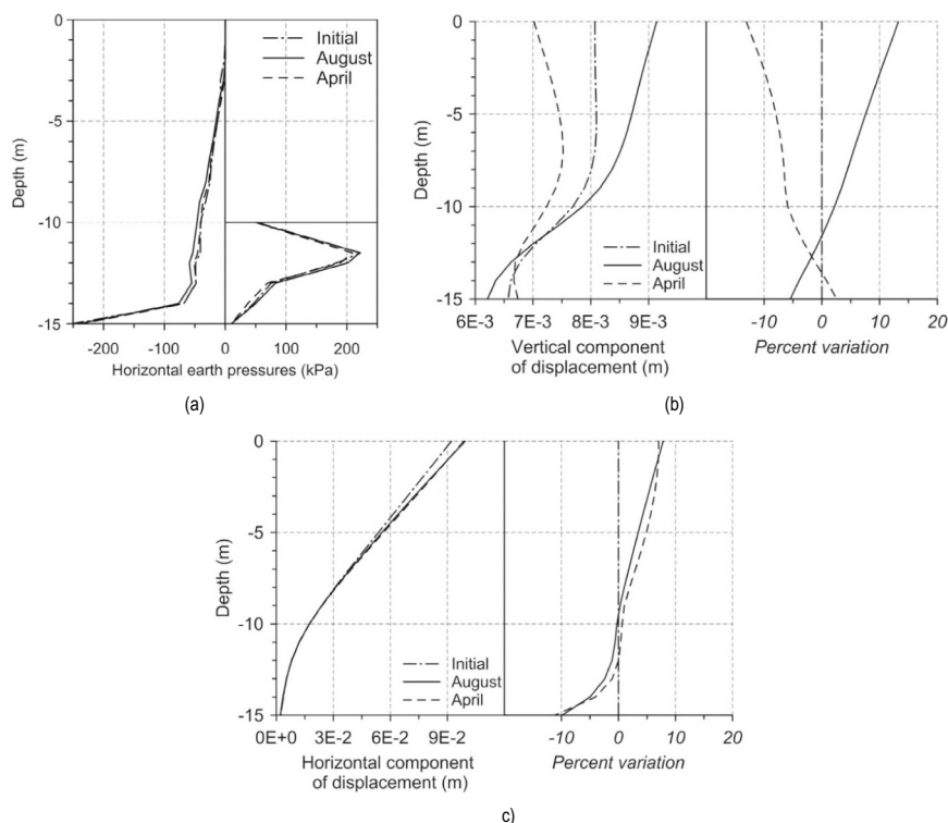
Fig. 4.4 (a) Horizontal earth pressure on the structure and (b) vertical and (c) horizontal components of the displacement (Sterpi et al., 2017)
