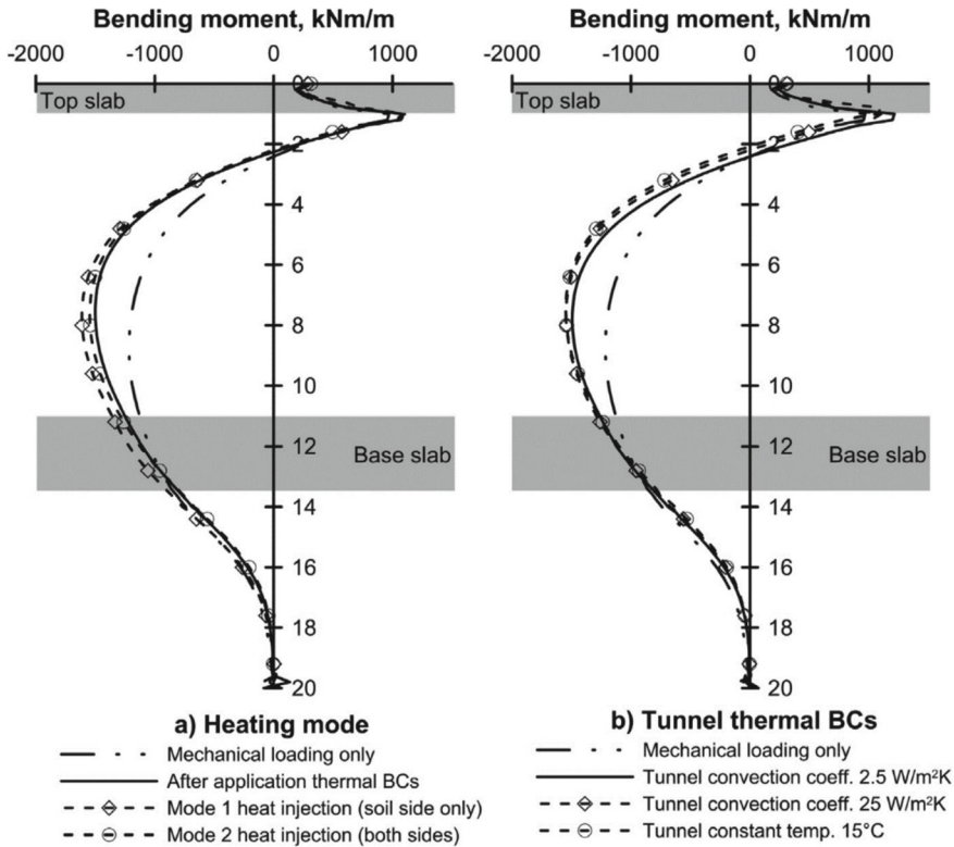
Fig. 4.7 Example of the variation of bending moment along an energy diaphragm wall, for different heating modes and thermal conditions at the excavation side (Bourne-Webb et al., 2016a)
