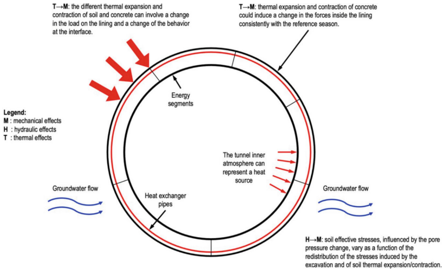
Fig. 4.8 Main issues involved in the geotechnical and structural design of energy tunnels (modified from Soga & Rui, 2016 and Ma et al., 2022)
