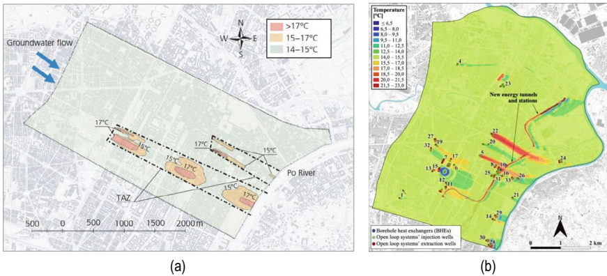
Fig. 5.6 Examples of Thermally Altered Zone (TAZ) in an urban area due to geothermal exploitation from open loop systems (a, Barla et al., 2020b) and their impact on an energy tunnel (b, Barla et al. 2025)
