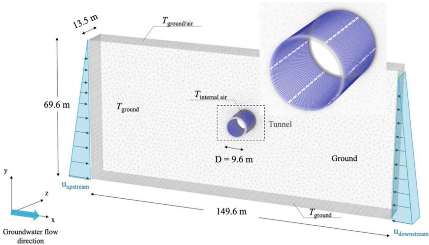
Fig. 3.6 3D view of the numerical model of an energy tunnel with indication of the hydraulic and thermal boundary conditions
