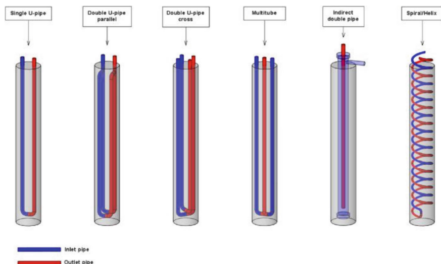
Fig. 6.1 Energy pile configurations (Fadejev et al., 2017)
