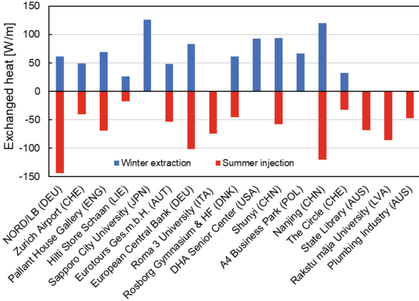
Fig. 3.1 Heat exchange per meter of pile length in real energy piles (from Cost Action Foliage, Salciarini et al. 2026)
