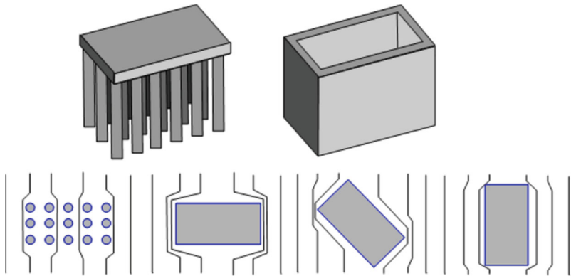
Fig. 5.5 Dam effect related to the type of infrastructure (CFMS and SYNTEC, 2017)
