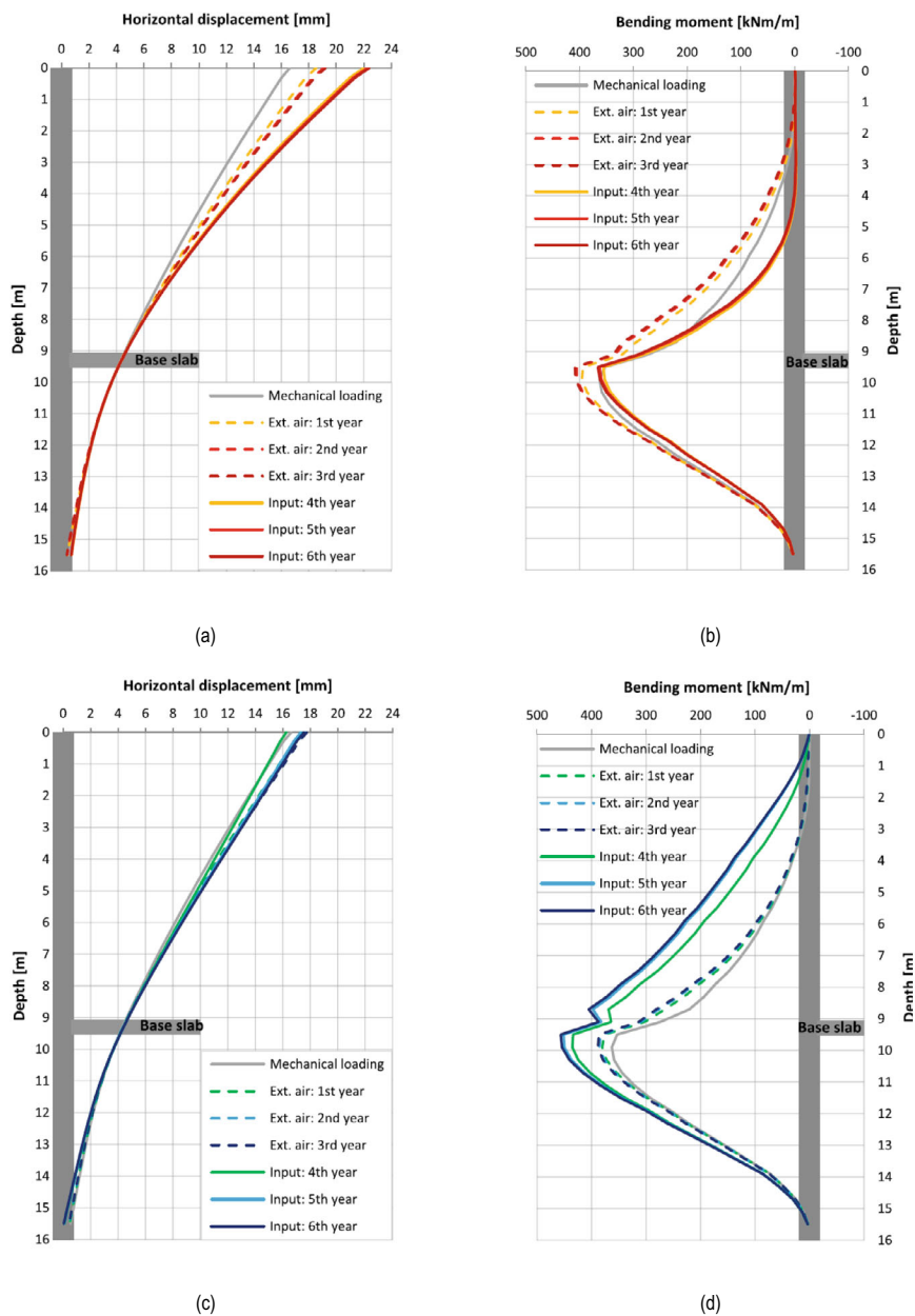
Fig. 4.6 Horizontal displacements and bending moment solicitations at different time frames during summer (a), (b) and winter season (c), (d) (Barla et al., 2020a)
