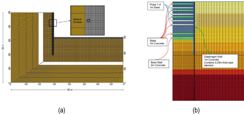
Fig. 4.3 Examples of (a) FDM and (b) FEM model for thermo-mechanical analysis of energy diaphragm walls (Barla et al. 2020a; Soga et al., 2015)
