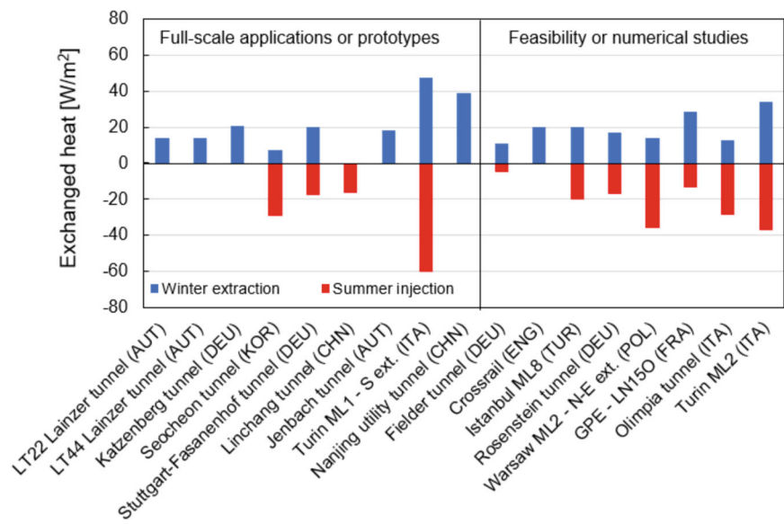
Fig. 3.4 Heat exchange per square meter of tunnel surface (from Cost Action Foliage, Salciarini et al. 2026)
