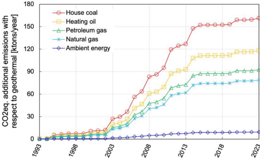
Fig. 1.3 CO 2 equivalent emissions for thermal energy production from fuels (house coal, heating oil, petroleum and natural gases) or air source heat pumps with respect to geothermal energy (Salciarini et al. 2025)
