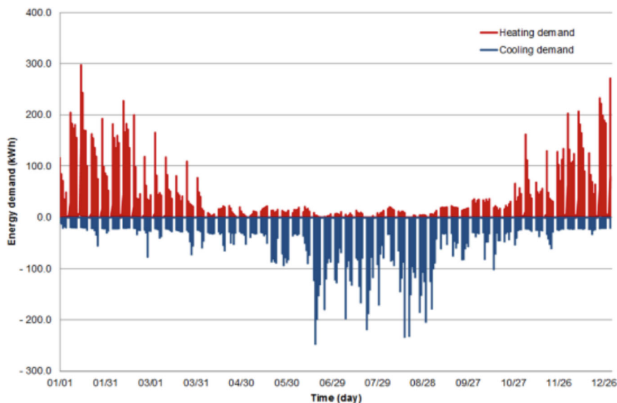
Fig. 2.4 Example of hourly energy demand in an office building
