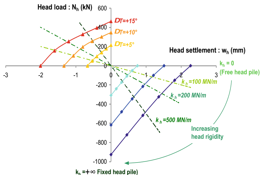
Fig. 4.2 Typical diagram of head settlement and head load variation due to thermal loading for different head rigidity levels (Burlon et al., 2013)
