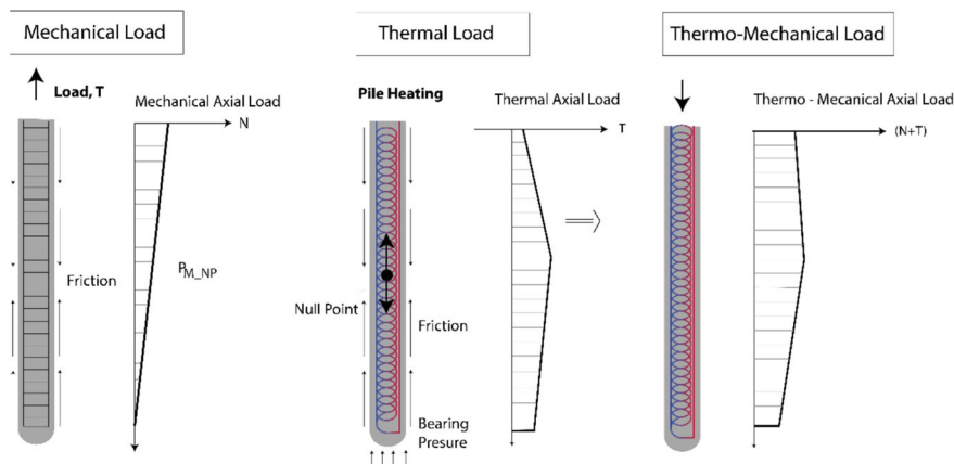
Fig. 4.1 Schematic illustration of thermo-mechanical behaviour of energy piles
