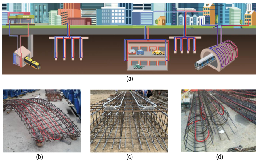
Fig. 1.2 a Illustration of the dual role of energy geostructures (courtesy of Foliage Cost Action) and example photos of, b energy tunnel lining (Politecnico di Torino, Italy), c energy diaphragm wall (Politecnico di Torino, Italy) and d energy pile (courtesy of Eneren, Italy)
