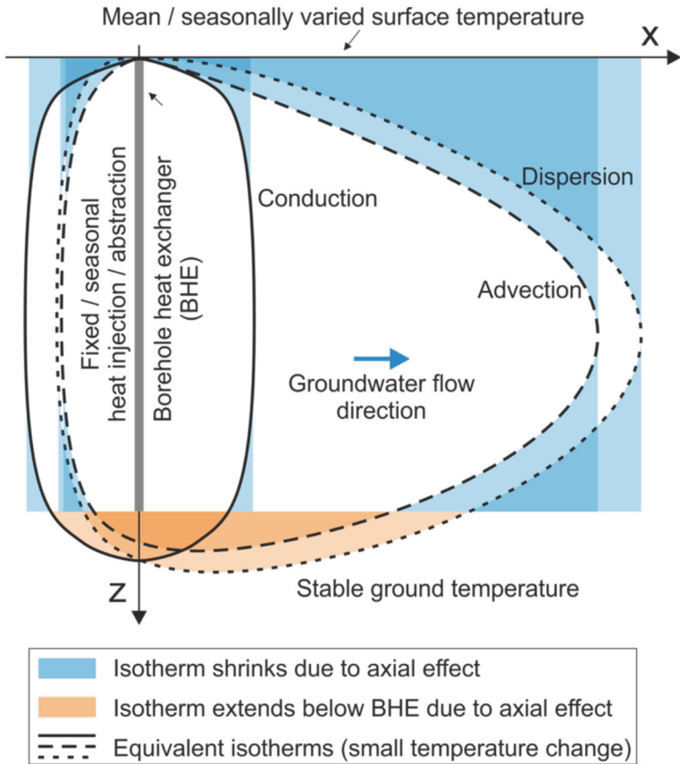
Fig. 5.1 Processes of heat transfer from BHE installed in homogeneous aquifer showing the effect of axial (in z direction) conduction and dispersion, groundwater advection and longitudinal and transverse dispersion. Equivalent Isotherms are shown for different mechanisms at same time (Pedchenko, 2019)
