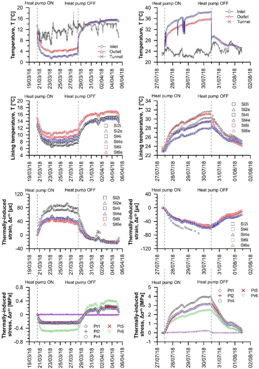
Fig. 4.9 Example of thermo-mechanical effects induced by thermal activation on the lining: winter mode test (left) and summer mode test (right) (Insana, 2020; Insana et al., 2020)
