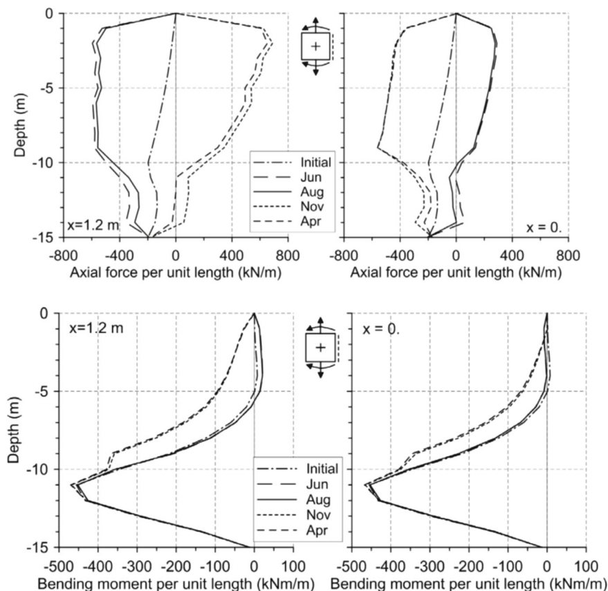
Fig. 4.5 Axial force and bending moment at different time frames in two different vertical cross sections (Sterpi et al., 2017)
