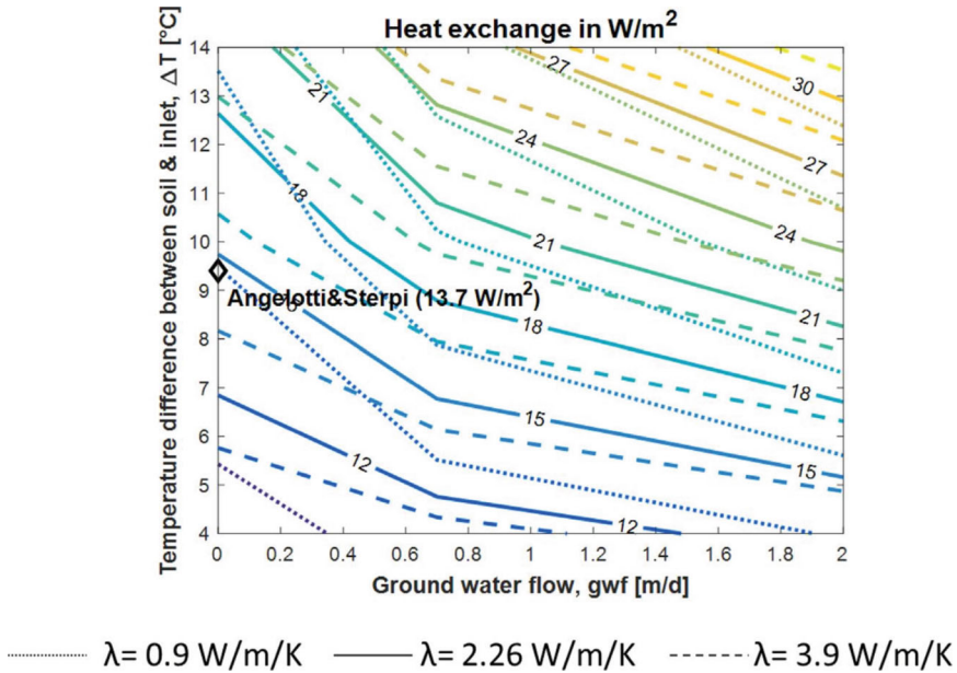
Fig. 3.3 Extracted heat in W/m 2 for energy walls (Di Donna et al. 2021)
