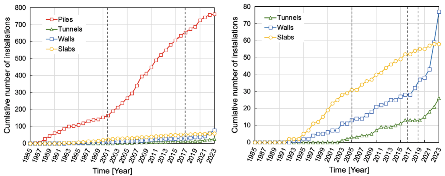
Fig. 1.4 Evolution of EGs installations (Salciarini et al. 2026)
