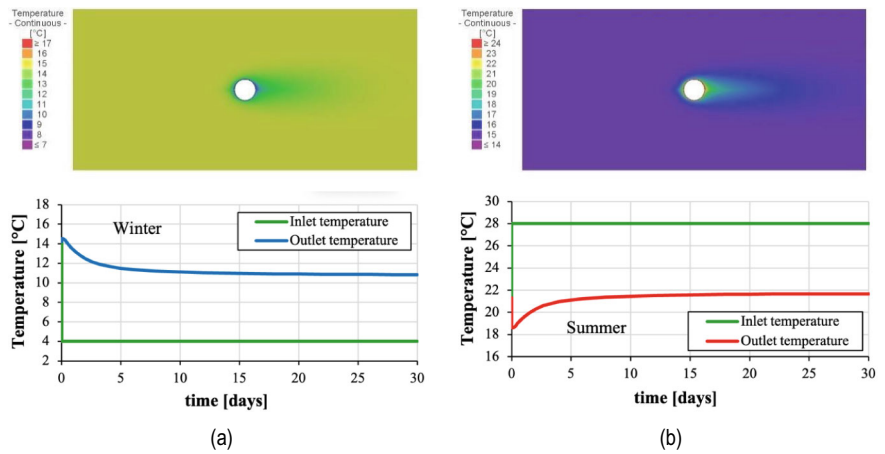
Fig. 3.7 Example of the result of a thermo-hydraulic 3D analysis: ground temperature and temperature calculated at the outlet of the geothermal circuit a in winter and b in summer
