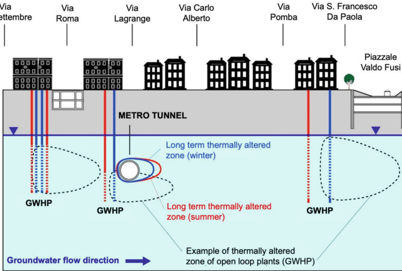
Fig. 5.2 Example illustration showing possible interferences in a specific urban context (courtesy of Geosolving Srl, Italy)
