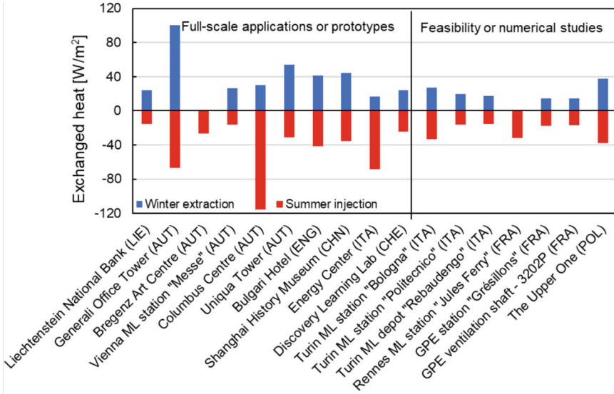
Fig. 3.2 Heat exchange per square meter of wall surface (from Cost Action Foliage, Salciarini et al. 2026)
