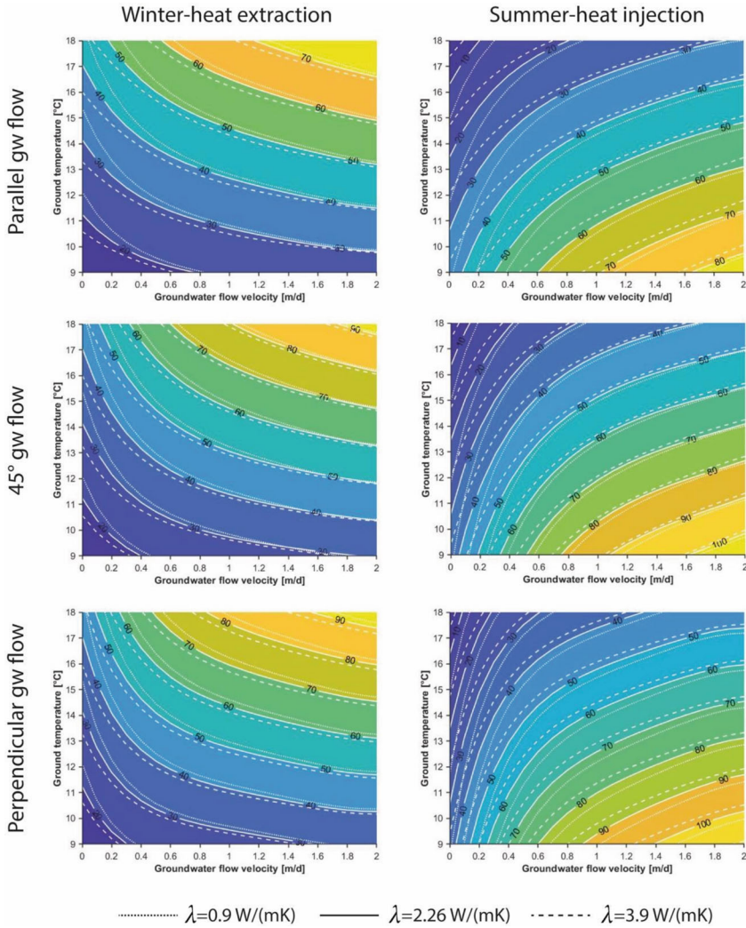
Fig. 3.5 Design charts for the evaluation of the geothermal potential in \text{W/m}^2 in winter and in summer for different directions of groundwater flow with respect to the tunnel axis ( 0^\circ , 45^\circ and 90^\circ ) (Insana and Barla 2020; Insana 2020)
