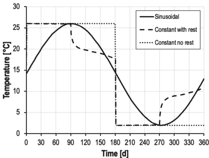
Fig. 2.3 Examples of temperature variation for different types of thermal loading functions
