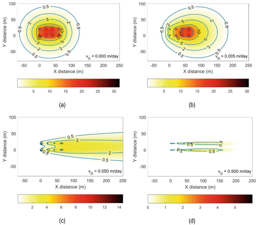
Fig. 5.4 Plan view of BHE field with isotherms of temperature change (K) for different Darcy groundwater velocities ( v_D ): (a) v_D = 0 m/day, (b) v_D = 0.005 m/day, (c) v_D = 0.05 m/day, (d) v_D = 0.5 m/day. Note that colour scales end with different maximal temperatures. Moving finite line source analytical solution (MFLS) was used (Pedchenko, 2019)
