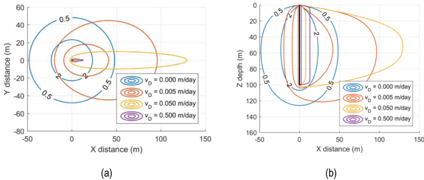
Fig. 5.3 Isotherm for 0.5 and 2 K temperature change for a range of Darcy's groundwater velocities ( v_D ) generated using analytical solution (moving finite line source). Vertical borehole heat exchanger of 100 m length is located at X Y = [0, 0] m. (a) Plan view; (b) Profile view (Pedchenko, 2019)
