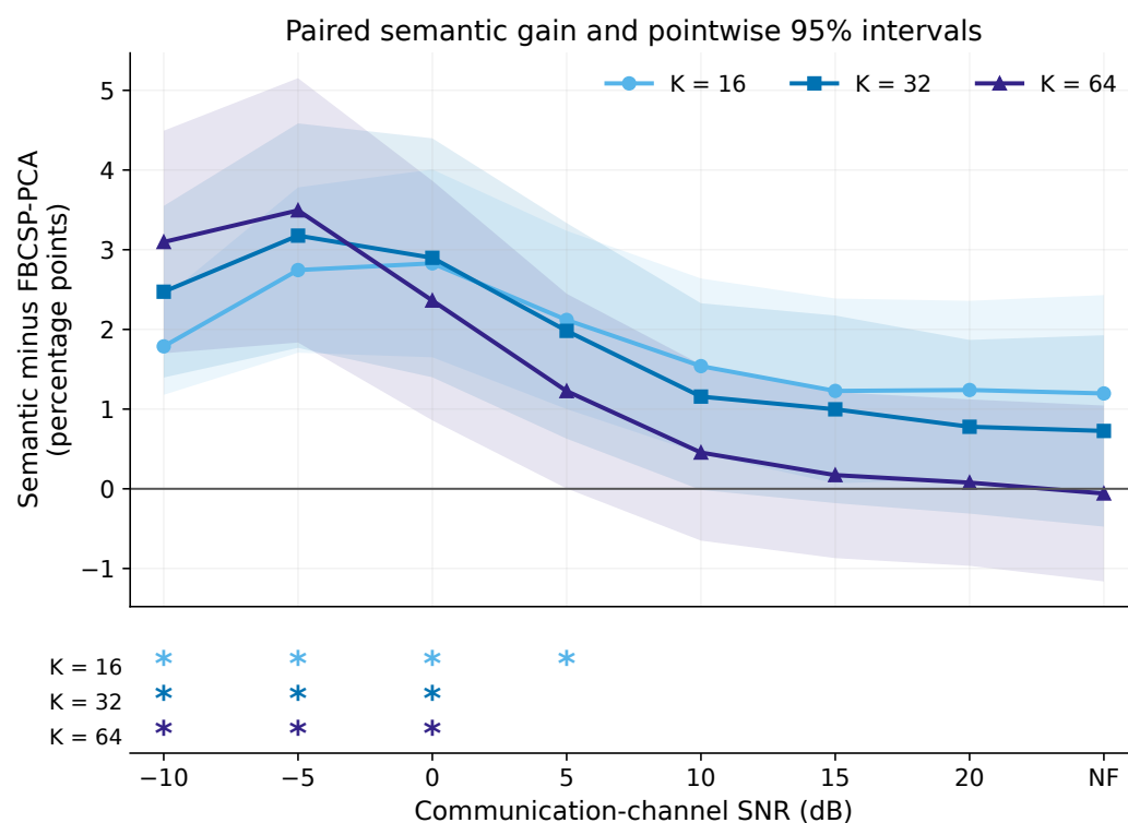
Figure 3. Semantic-minus-FBCSP–PCA balanced-accuracy difference. Bands show descriptive pointwise 95% confidence intervals; asterisks in the lower rows denote exact max- |t| -adjusted p < 0.05 ; NF, noise-free.
