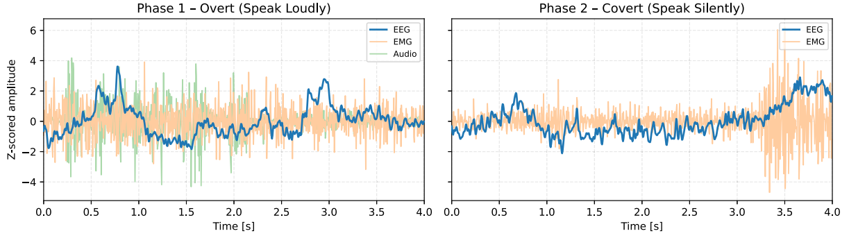
Fig. 3. Representative multimodal trial from participant S02 (run 09). Phase 1 (overt speech) shows z-scored EEG, EMG, and audio waveforms during spoken articulation. Phase 2 (covert inner speech) shows the corresponding EEG and EMG activity during the covert interval, which may still contain low-amplitude residual articulatory activity. Audio is absent in this phase. All signals are z-scored within channel.
