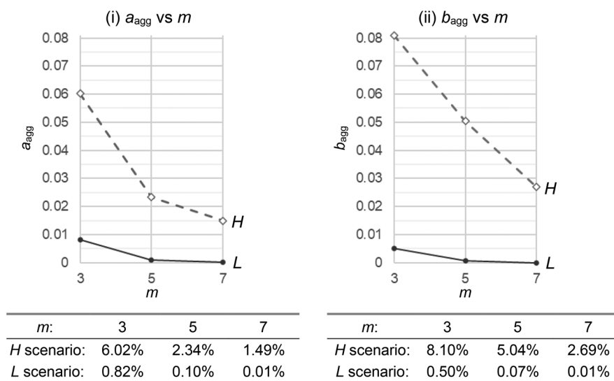
FIGURE 7 | Effect of the number of inspectors ( m ) in terms of reduction in a_{agg} and b_{agg} , considering the two error-rate scenarios ( H and L ). The tables below show the numerical values plotted.
