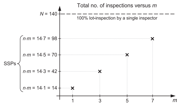
FIGURE 9 | Comparison of the total number of inspections required per lot, under different inspection strategies: full 100% inspection of an entire lot by a single inspector, versus SSPs (with sample size n ) executed by either a single inspector ( m = 1 ) or by a group of inspectors ( m = 3, 5, 7 ). The example assumes N = 140 and n = 14 . Even with multiple inspectors, the SSPs use substantially fewer inspections than 100% lot inspection (dashed line).
