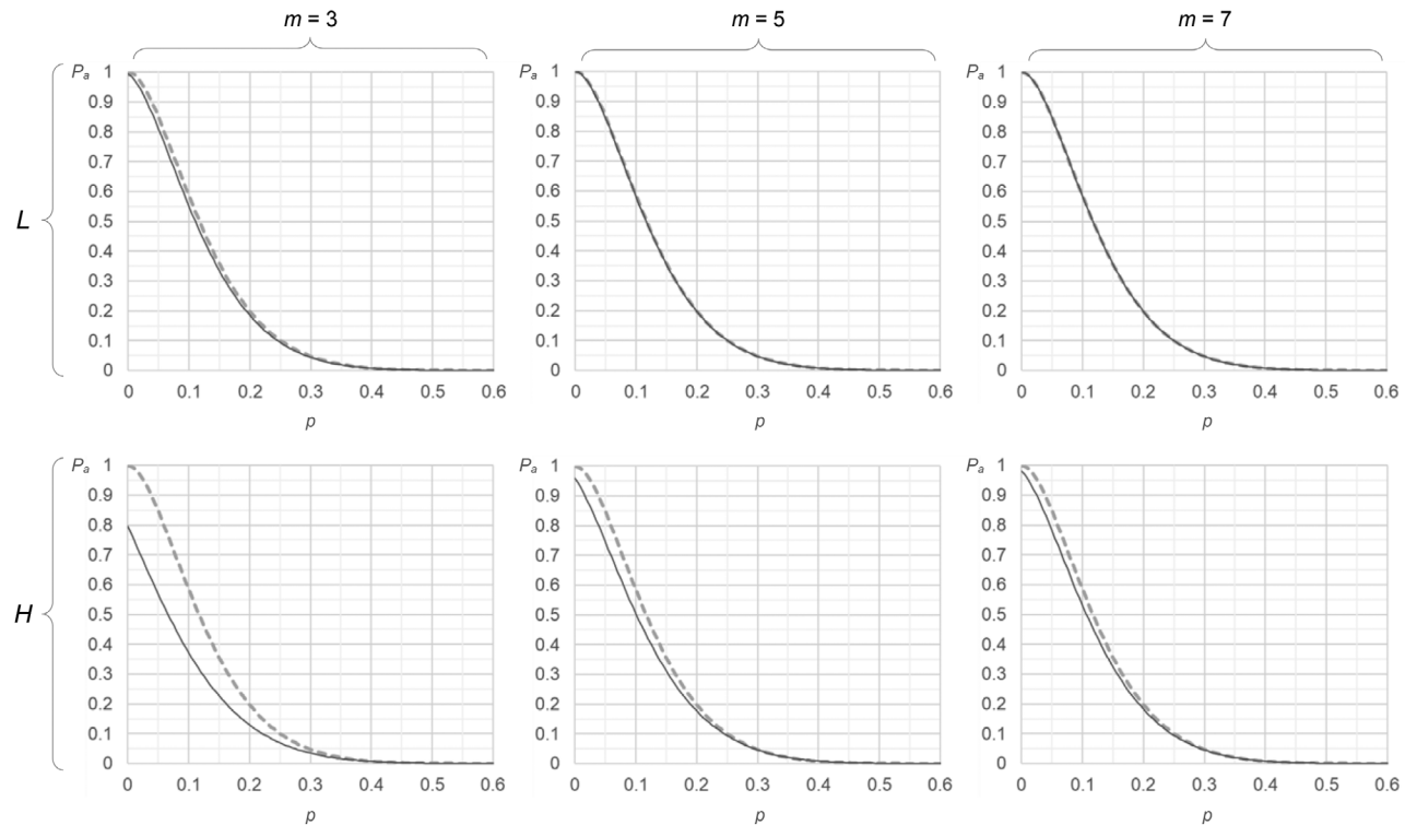
FIGURE 8 | OC curves for the multiple-inspector SSP under varying conditions: two error scenarios ( L in top row, H in bottom row) and different number of inspectors ( m = 3, 5 and 7 , in the columns). In each plot, the solid line represents the actual OC curve with inspectors' errors and the dashed line represents the ideal OC curve (with no inspection errors). In the L scenario, even a group of m = 3 inspectors produces an OC curve virtually identical to the ideal one. In the H scenario, larger groups ( m = 5 or 7 ) are needed to closely approximate the ideal OC curve, although m = 3 still shows some deviation. Overall, increasing the number of inspectors drives the OC curve of the sampling plan to converge toward the error-free ideal one, illustrating the compensatory effect of multiple inspectors.
