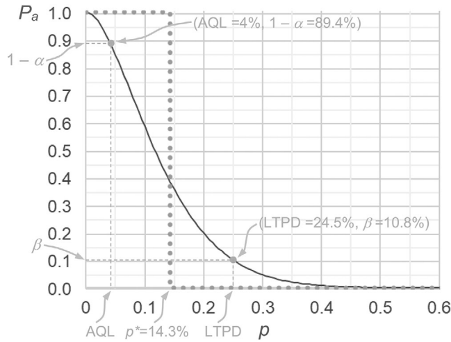
FIGURE 3 | The solid line represents the Type-B OC curve for a SSP with parameters n = 14 and c = 1 . This SSP was designed such that p^* \approx 14.3\% (the ‘knee’ of the ideal step-shaped OC curve for 100% inspection; dashed line from Figure 1) lies roughly midway between an AQL of 4% and an LTPD of 24.5%, yielding corresponding producer’s and consumer’s risks of about 10.6% and 10.8%, respectively. In other words, the chosen SSP is characterised by an OC curve that ensures a protection level and/or severity in line with the ideal step-shape OC curve of 100% inspection (cf. Figure 1).
