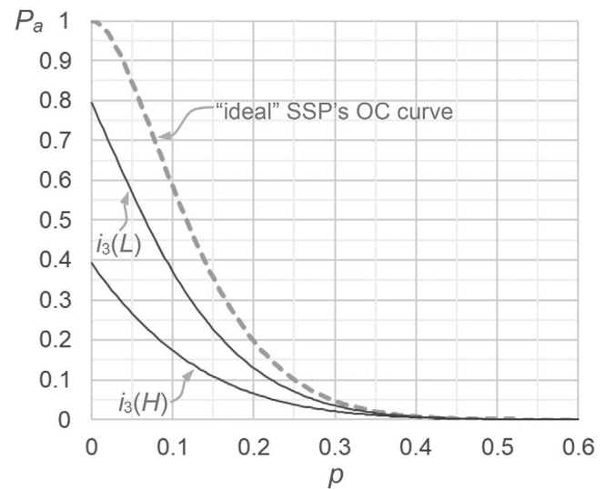
FIGURE A1 | OC curves for a single inspector ( i_3 ), in the L scenario (with a_3 = 6.5\% and b_3 = 6.0\% ) and in the H scenario (with a_3 = 14.1\% and b_3 = 16.8\% ). The OC curves were constructed using the model in Equation A3. For ease of comparison, the ideal OC curve with no errors, constructed using the model in Equation 12, is also shown (as a dashed line).
