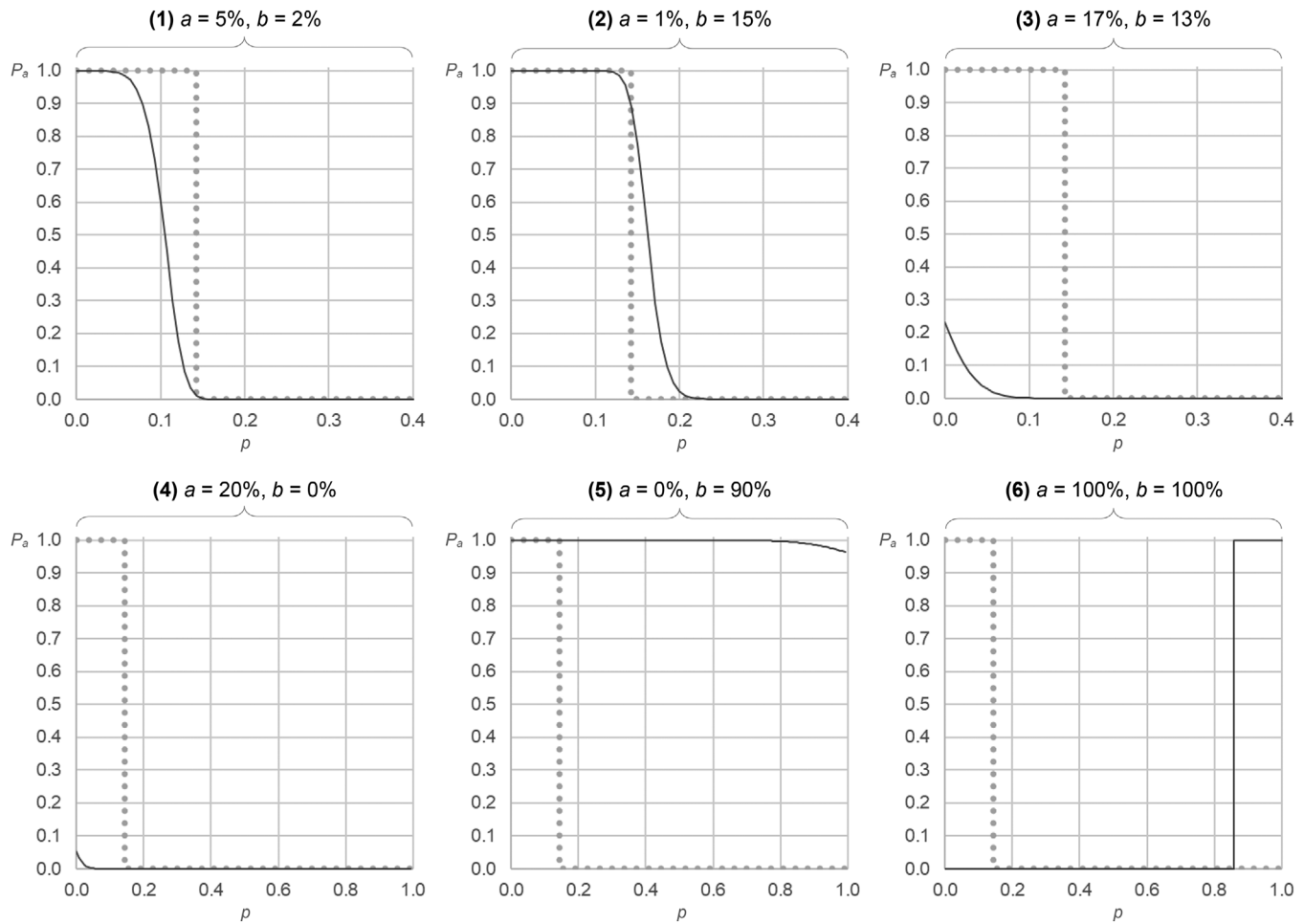
FIGURE 2 | Effect of inspection-error rates on OC curves for a single-inspector 100% inspection, with N = 140 and D^* = 20 . For six combinations of a and b , the OC curves are obtained using the model in Equation 9. The parameters a and b were varied within very wide ranges to make their effects more visible. For greater generality, the horizontal axes of the curves show p = D/N ; furthermore, the horizontal axis of the top three plots is truncated at p = 0.4 , for more clarity. In each of the six plots, the ideal step-shaped OC curve (with no errors) is shown as a dotted line for reference (cf. Equation 1 and Figure 1).
