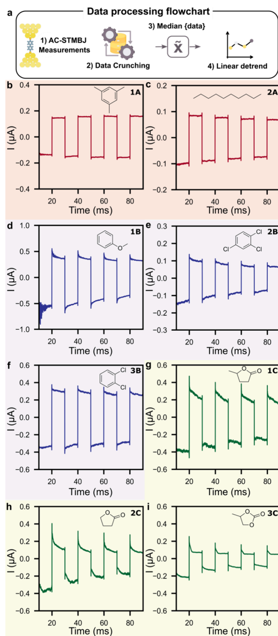
Figure 2. (a) Flowchart of the AC-STMBJ data processing pipeline: acquisition of the raw traces, data crunching, trace-by-trace median extraction, and linear detrending. (b–i) Representative single current traces measured in the investigated solvents: mesitylene, decane, anisole, 1,2,4-trichlorobenzene, 1,2-dichlorobenzene, \gamma -valerolactone, \gamma -butyrolactone, and propylene carbonate.
