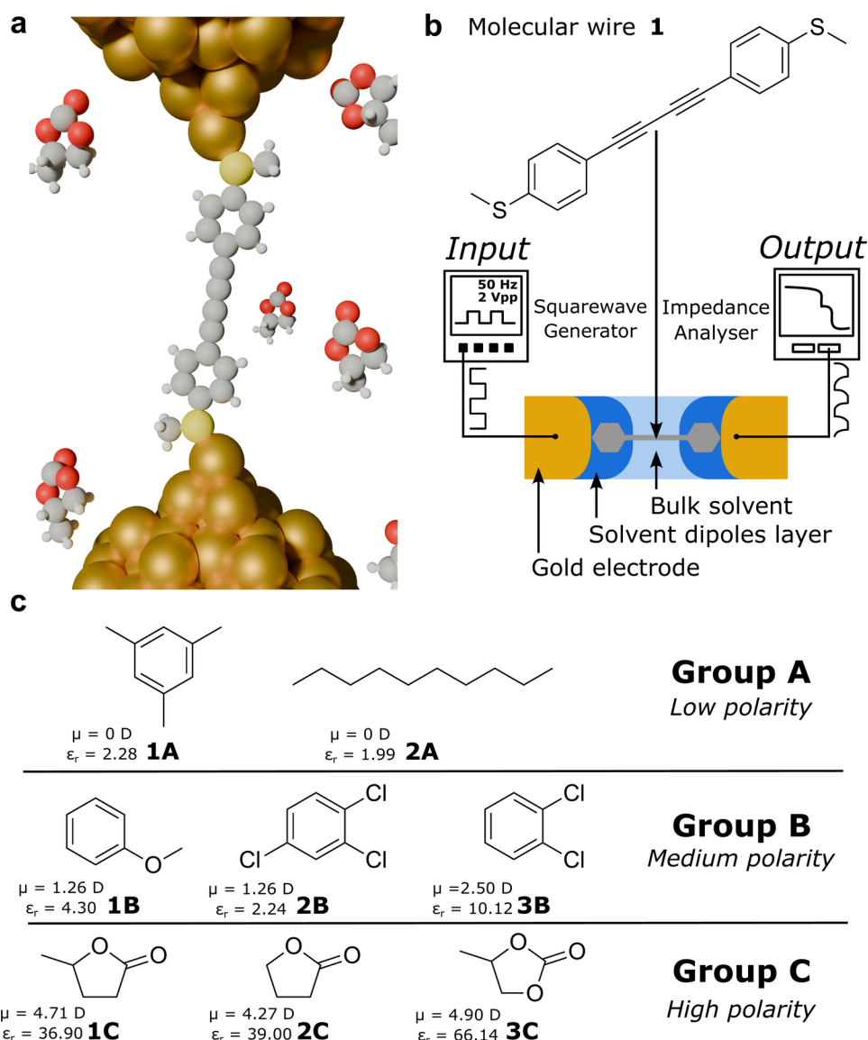
Figure 1. (a) Rendered representation of a representative device configuration, showing a bis(thioanisyl)butadiynyl molecular wire bridging two Au electrodes via coordinative S–Au bonds. A limited number of solvent molecules is included to qualitatively illustrate the local environment. (b) Schematic of the experimental setup employed in this work. A square-wave voltage ( 2 V_{pp} i.e. \pm 1 V, 50 Hz) is applied to the single-molecule junction (SMJ), while the output signal reflects time-dependent impedance (current) variations. The SMJ conductance is continuously monitored under different solvent environments. (c) Set of solvents investigated in this study, selected based on polarity in order to span a broad range of physicochemical properties, with the molecular dipole moment \mu and the static relative permittivity \epsilon_r reported beneath each structure: 1A mesitylene, 2A decane, 1B anisole, 2B 1,2,4-trichlorobenzene, 3B 1,2-dichlorobenzene, 1C \gamma -valerolactone, 2C \gamma -butyrolactone, and 3C propylene carbonate. The three panels correspond to Group A (low polarity, \mu < 0.5 D, \epsilon_r < 2.5 ), Group B (medium polarity, \mu = 1.2 - 2.5 D, \epsilon_r = 2.2 - 10.1 ) and Group C (high polarity, \mu > 4 D, \epsilon_r > 35 ). Numerical values for all eight solvents are collected in Table S1.
