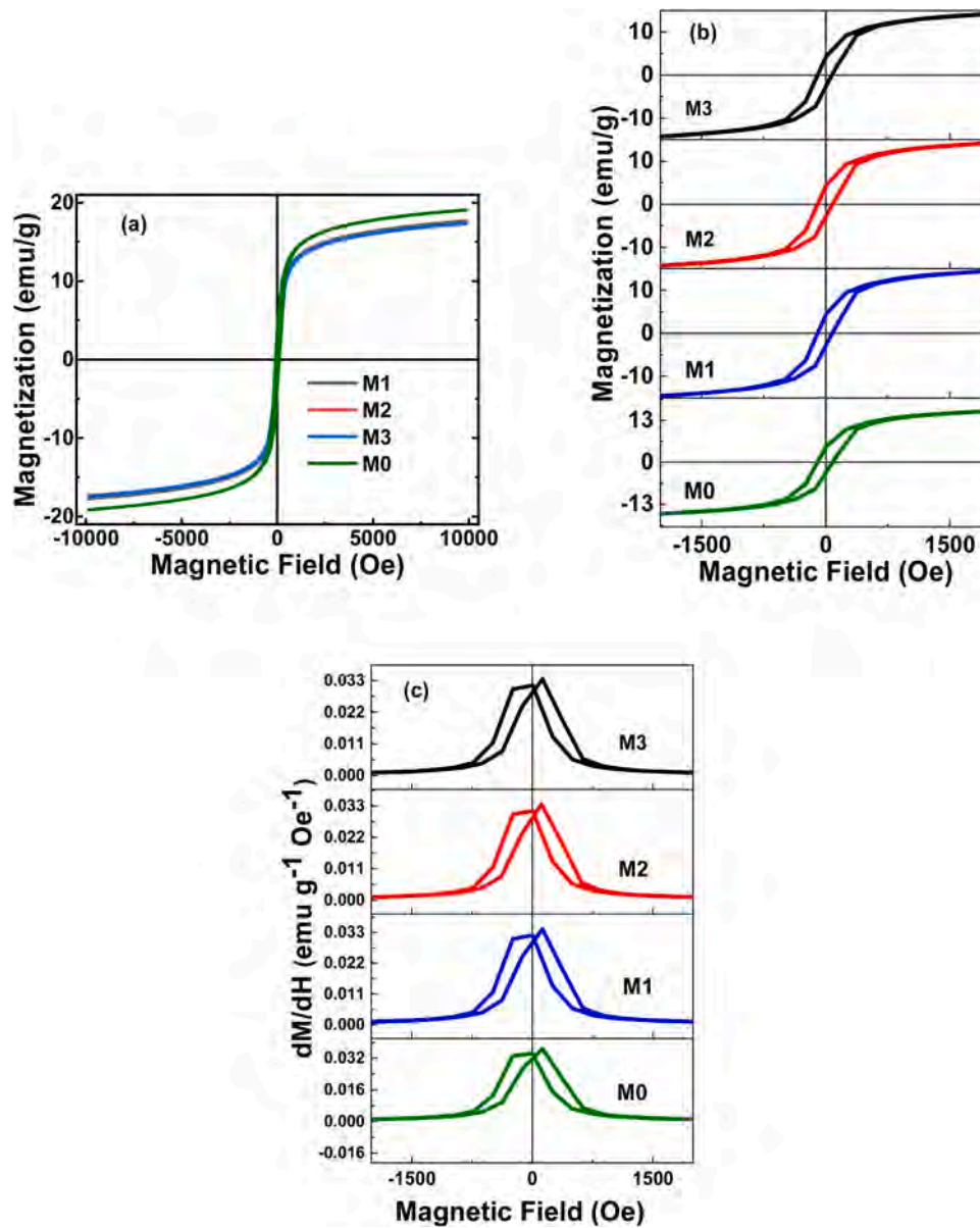
Fig. 9. Hysteresis-loops (a,b), (c) Corresponding first derivatives.
