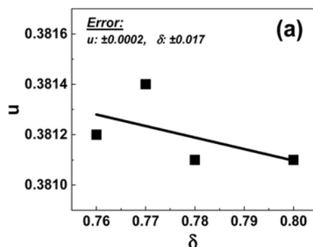
Fig. 4. (a) Plot of u with \delta , (b) Annealing-time dependence of M_{s(\text{th})} at 0 K.
