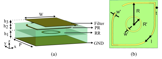
Fig. 2. (a) Unit cell. (b) Polarization rotator (PR) and ring resonator (RR) from top view. GND: ground. Period ( P ): 10 mm, filter width ( W ): 6.5 mm, edge clearance: t : 0.5 mm, substrate heights ( h_{1,2} ): 1.5 mm, 1.25 mm respectively, air gap h_3 : 0.5 mm, split gap size ( l ): varying, PR radius ( R ): 4.5 mm, RR radius ( R' ): 1.7 mm. Copper trace width ( w' ): 250 \mu\text{m} . FR4 substrates (green), copper (yellow)
