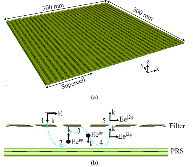
Fig. 1. (a) RIS panel configured for a 30^\circ deflection. (b) Step-by-step visualization of the phase doubling concept using reflections. The flow (solid cyan line) shows the wave undergoing five steps, where additional phase \varphi is accumulated via reflections. PRS: Polarization rotating surface. k : wave vector. E : Electric field
