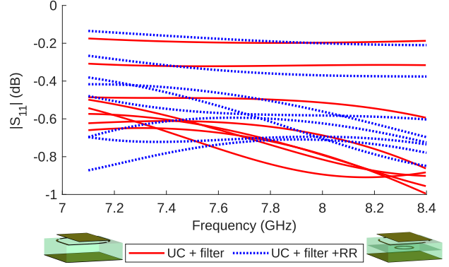
Fig. 5. Amplitude comparison of the 3-bit states for two different unit cell designs, both excited in TM mode: Design including a filter (solid lines), and the design including a filter, and a ring resonator (dotted lines). Substrate height: 2.75 mm and 3.2 mm for designs with and without RR respectively.
