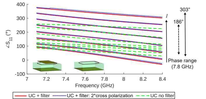
Fig. 4. Phase comparison of the 3-bit states for design including a filter (solid and dotted lines), and the design without filter (dashed lines). Both excited in TM mode. Small and large phase ranges are for unit cells (UC) without and with the filter respectively. 2* indicates the phase values multiplied by two. Each state is defined by a split gap size l shown in table I and the increasing order is shown by an arrow. Substrate height: 3.2 mm
