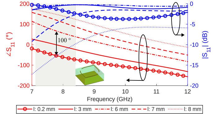
Fig. 3. Phase and amplitude of the polarization rotator for the cross polarization state at different values of l . The desired band is highlighted with gray rectangle. Substrate height: 3.2 mm
