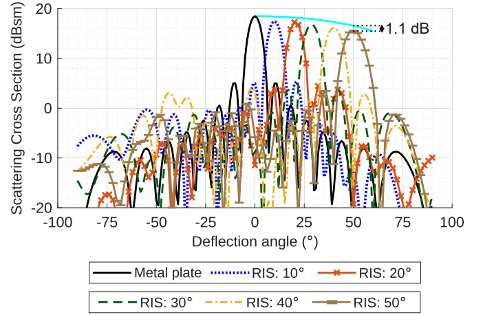
Fig. 8. Beam scanning at 7.8 GHz for different deflection angles. Scan loss (solid cyan line) calculated with respect to a copper plate having the same surface as RIS.
