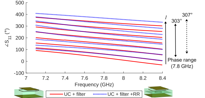
Fig. 6. Phase comparison of the design with and without the ring resonator for 3 bit states. Each state is defined by a split gap size l shown in table I and the increasing order is shown by an arrow. Substrate height: 2.75 mm and 3.2 mm for designs with and without RR respectively.
