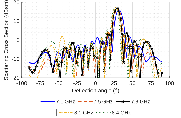
Fig. 7. Radiation pattern at different frequencies of RIS designed for 30° deflection angle.
