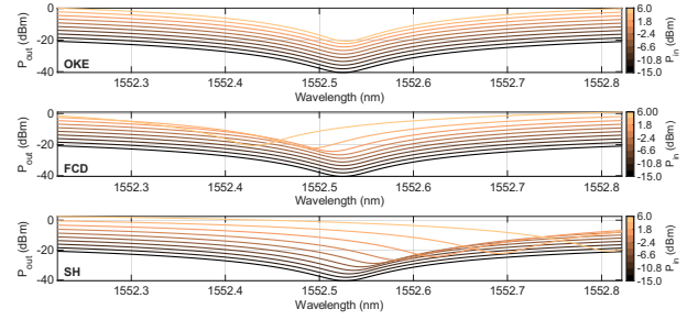
Fig. 2. Output power spectra of the MRR for varying input power levels, obtained by simulating the model with all nonlinear effects turned off, except one at a time.
