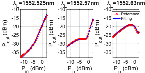
Fig. 1. Comparison between PSO-fitted simulations (blue) and measurements (red) of P_{\text{out}}-P_{\text{in}} curves at different values of input laser wavelength \lambda_L .
