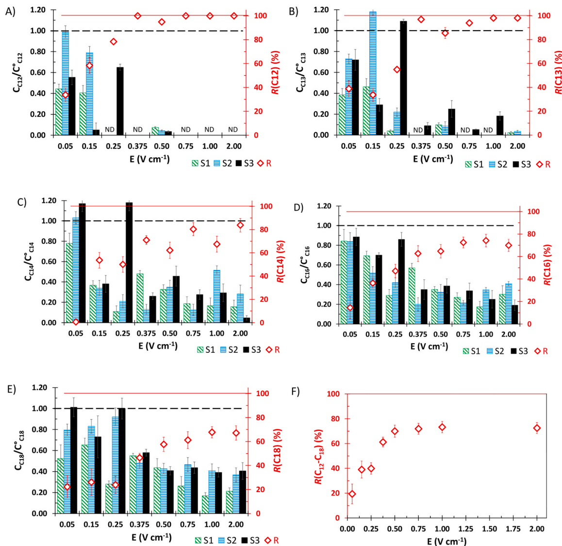
Fig. 3. Effect of E strength on the C_i/C^\circ in the regions S1, S2 and S3 (primary y-axis) and total removal, R(C_i) , from the kaolin (secondary y-axis) of each contaminant (A) C12, (B) C13, (C) C14, (D) C16, (E) C18. (F) Effect of E strength on the removal of the mixture C_{12-C18} from the kaolin R(C_{12-C18}) . Black dashed line (— — —) marks C_i/C^\circ equal to 1 (at the time zero of treatment) (primary y-axis). Red solid line marks the 100% of R (secondary y-axis). Compact graphite electrodes. Time: 96 h. ND: Not detected. Electrochemical cell: I.
