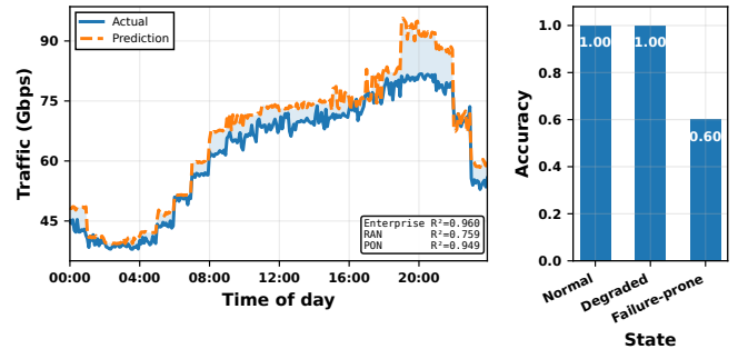
Fig. 2: Left: XGBoost traffic forecasting. Right: RF network-state classification.
