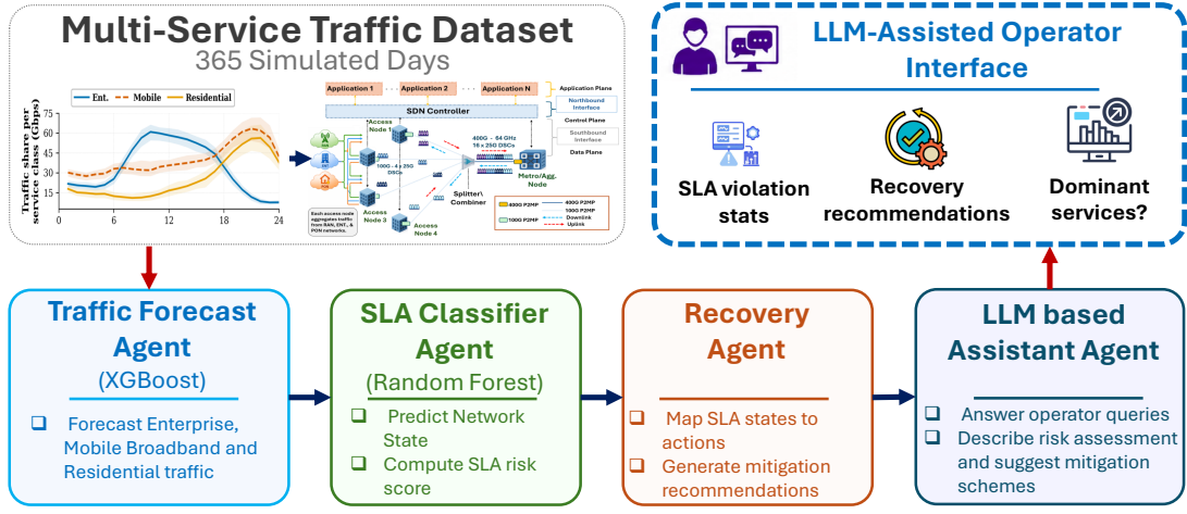
Fig. 1: Multi-agent framework for SLA management.
