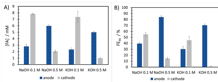
Fig. 3. Effect of the SE concentration on [FA] (3A) and FE FA (3B) achieved at the end of the electrolyses for both anodic and cathodic processes. Electrolyses were performed at 11 mA cm -2 using a tin cathode and a BDD anode for 2 hours in a divided cell with an aqueous solution of NaOH or KOH in both compartments and 0.5 M MeOH in the anolyte.
