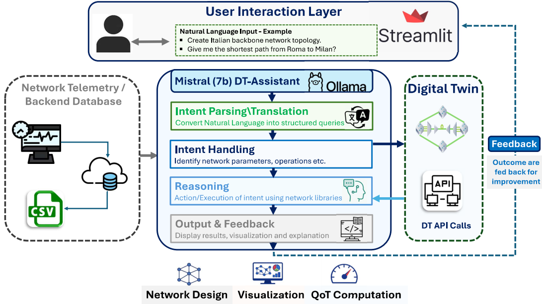
Fig. 1: LLM-orchestrated Digital twin architecture for intelligent optical network operations
