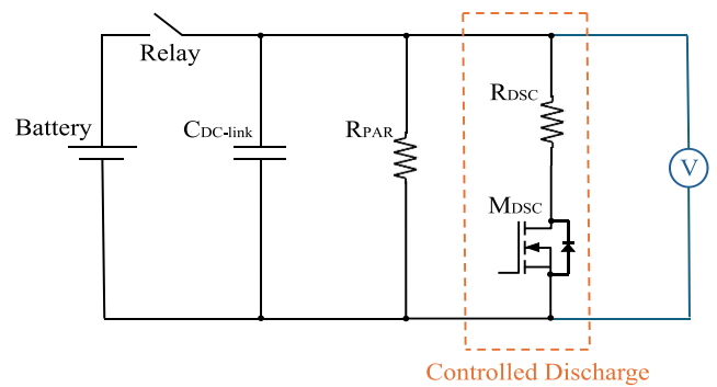
FIGURE 2. Functional electrical schematic of the proposed condition monitoring test circuit showing the inverter's dc-link capacitor connected to the battery using a safety high-voltage relay (or contactor) and the proposed discharge circuit.
