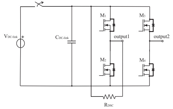
FIGURE 8. Schematic of the experimental test rig, where a MOSFET ( M_2 ) is used as the discharging switch.
