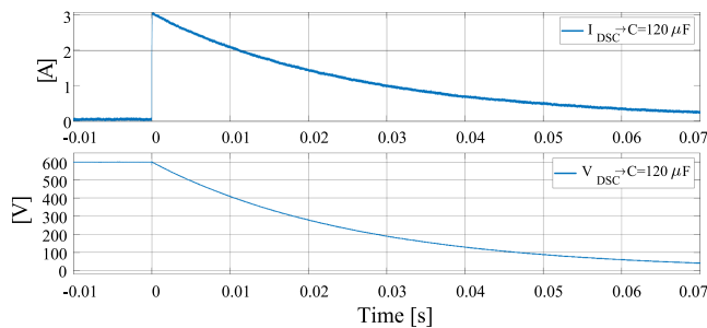
FIGURE 13. Voltage and current discharge profiles of the 120 \mu\text{F} capacitor measured with the oscilloscope.
