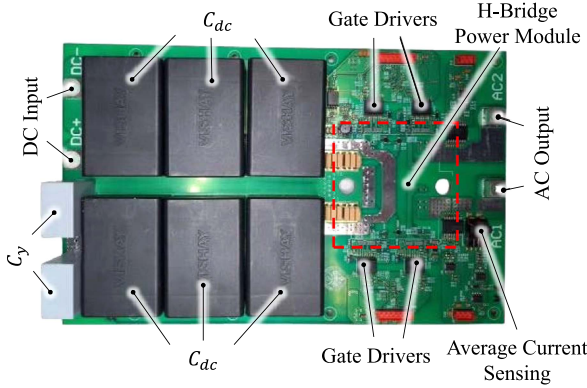
FIGURE 7. Experimental H-bridge converter.
