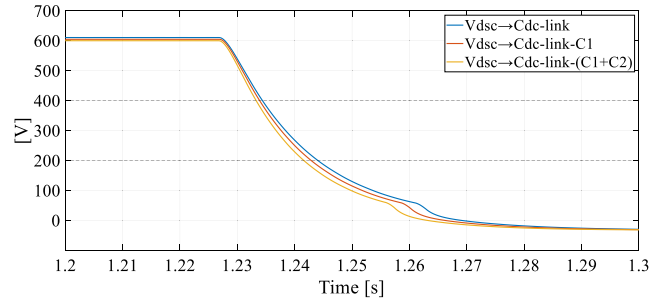
FIGURE 10. Voltage discharge profiles of three capacitors, measured with the H-bridge embedded voltage sensor, when R_{DSC} = 200 \, \Omega . The discharge voltage profiles are integrated between V_{start} = 400 \, \text{V} and V_{end} = 200 \, \text{V} .
