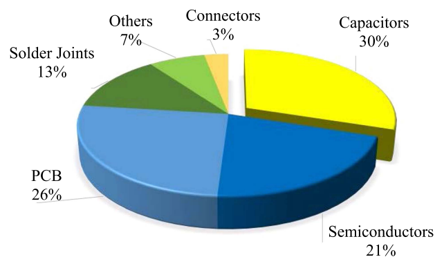
FIGURE 1. Distribution of failure modes in power electronic converters [4].
