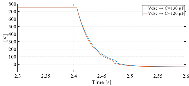
FIGURE 12. Voltage discharge profiles of both 130 and 120 \mu\text{F} capacitors measured with the H-bridge embedded voltage sensor. The discharge voltage profiles are integrated between V_{\text{start}} = 650 \text{ V} and V_{\text{end}} = 100 \text{ V} .
