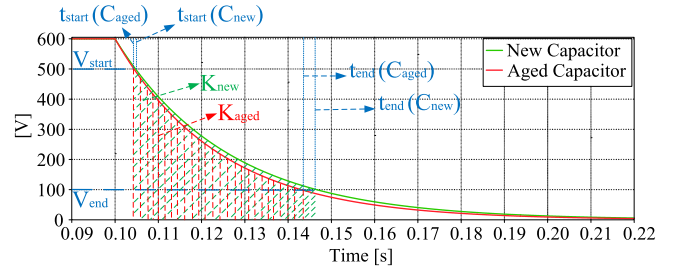
FIGURE 4. Voltage profiles of both new and aged capacitors.
