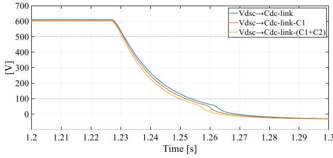
FIGURE 9. Voltage discharge profiles of three capacitors, measured with the H-bridge embedded voltage sensor, when R_{DSC} = 200 \, \Omega . The discharge voltage profiles are integrated between V_{start} = 500 \, \text{V} and V_{end} = 100 \, \text{V} .
