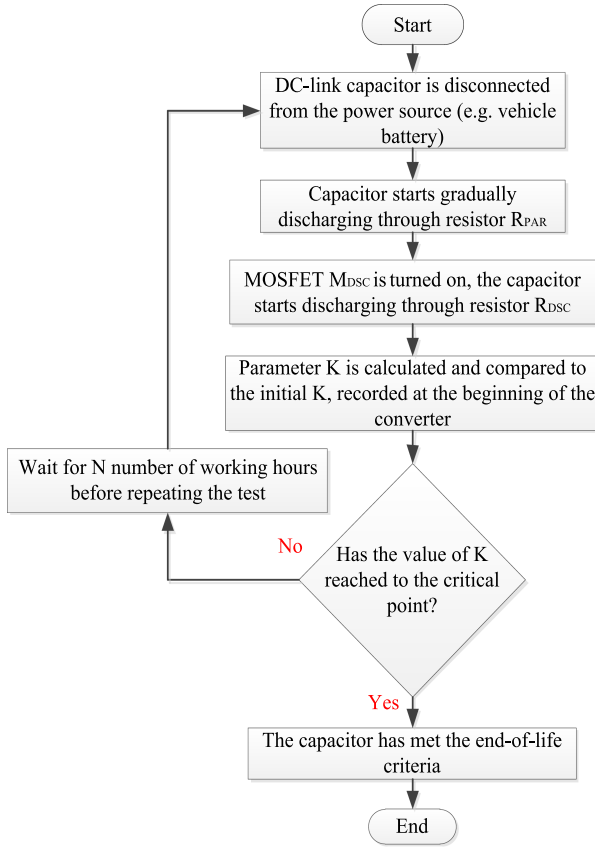
FIGURE 3. Flowchart of the proposed condition monitoring test.
