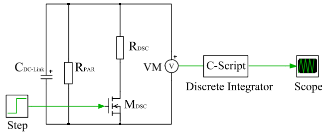
FIGURE 5. PLECS implementation of the controlled discharging test.
