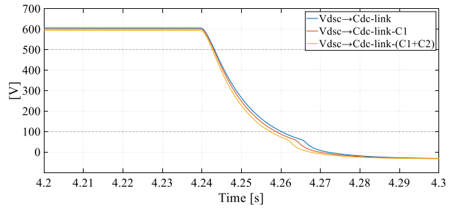
FIGURE 11. Voltage discharge profiles of three capacitors, measured with the H-bridge embedded voltage sensor, when R_{DSC} = 150 \, \Omega . The discharge voltage profiles are integrated between V_{start} = 500 \, \text{V} and V_{end} = 100 \, \text{V} .
