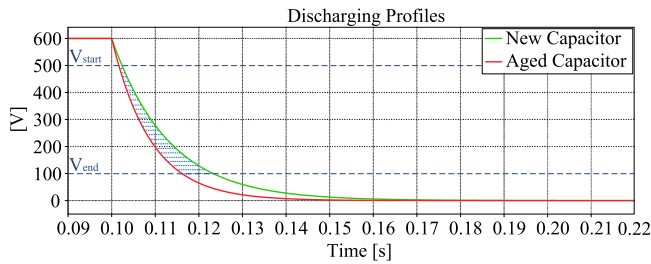
FIGURE 6. Difference between the voltage profiles of the new capacitor and the aged one.
