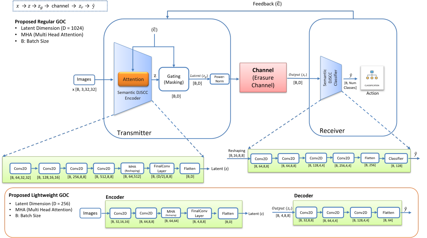
Fig. 1: Proposed GOC model pipeline.
