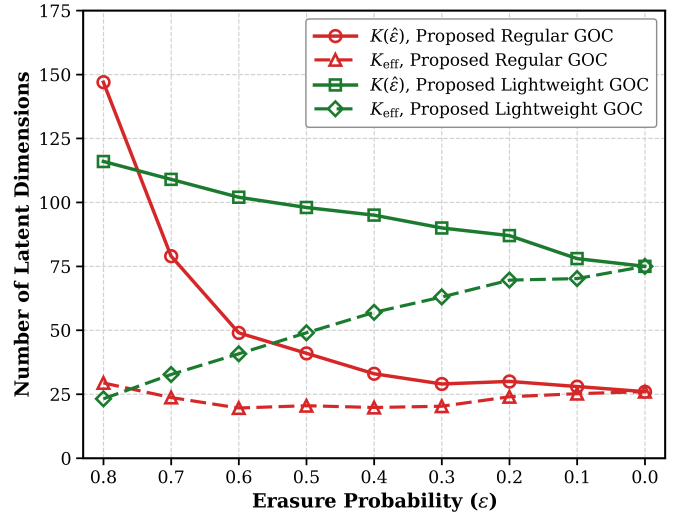
Fig. 3: Number of active transmitted latent dimensions K(\hat{\epsilon}) and effective number of dimensions received at the decoder, K_{\text{eff}} = K(\hat{\epsilon})(1 - \epsilon) , versus the erasure probability \epsilon , for the proposed regular GOC and the proposed lightweight GOC.
