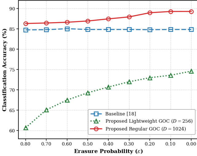
Fig. 2: Classification accuracy of the proposed regular GOC, proposed lightweight GOC, and baseline [18] versus erasure probability \epsilon .
