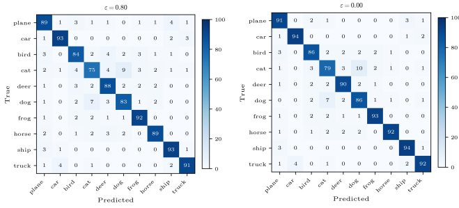
Fig. 4: Confusion matrices of the proposed regular GOC on CIFAR-10 dataset.
