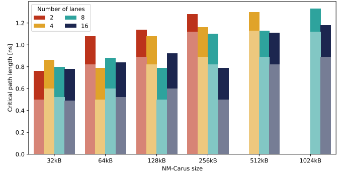
Figure 2: Critical path of the NM-Carus configurations. Bars are split into two: the lighter part represents the portion of the timing portion taken by the SRAM banks, while the darker part represents the delay introduced by logic cells.
