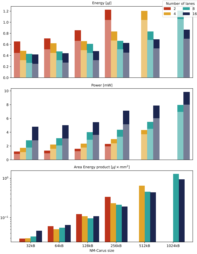
Figure 3: Power, energy and area energy product of NM-Carus for different configurations when running at 100 MHz an 8-bit matrix multiplication ( A[10 \times 10] \times B[10 \times 1024] ). Power and energy bars are split into two: the lighter part represents the portion of the power dissipated by SRAM banks, while the darker part represents the logic cells.
