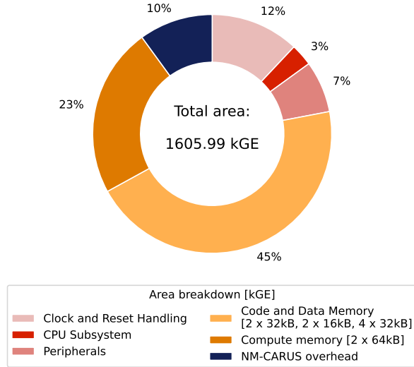
Figure 4: Area breakdown of X-HEEP with two NM-Carus instances. Area reported on the pie-chart is in equivalent kilogates (kGE).
