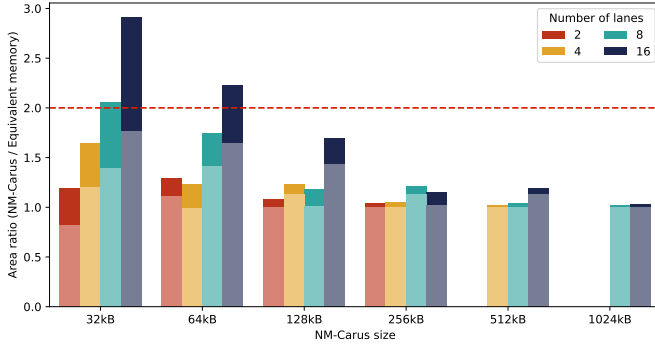
Figure 1: Ratio between the area of differently configured NM-Carus instances and conventional single-bank SRAM memories with equivalent sizes. The dashed line represents the NMC overhead threshold defined in [7] as equal to 2. Bars are split into internal SRAM area (lighter color) and the logic cell area (darker color).
