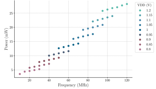
Figure 3: Total chip power consumption vs. operating frequency at supply voltages from 0.8 V to 1.2 V under a representative arithmetic workload.
