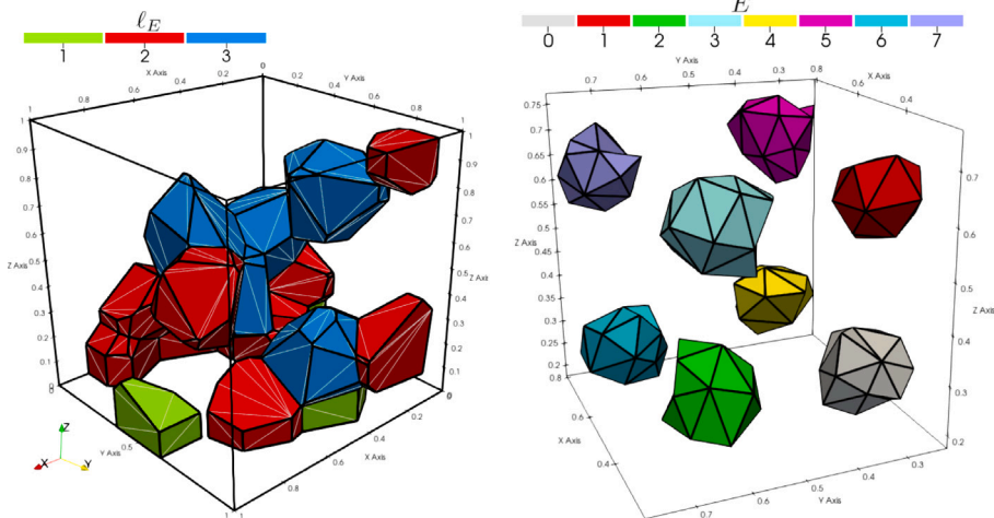
(a) Convex polyhedra randomly selected from \mathcal{D}_{\text{voro-poisson}} second mesh of the dataset in Sorgente et al. (2022), adding the sub-triangulation of faces. Each polyhedron is colored depending of the value of \ell_E given by Algorithm 1. (b) Concave polyhedra obtained by random agglomeration of tetrahedra.
